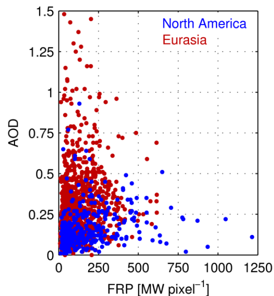
Fig. 3.6: Scatterplot between AOD and FRP for Eurasia (red) and North America (blue). The data points represent all boreal forest pixels (2007-2012) with a p -value < 0.05 and r > 0.3 .
