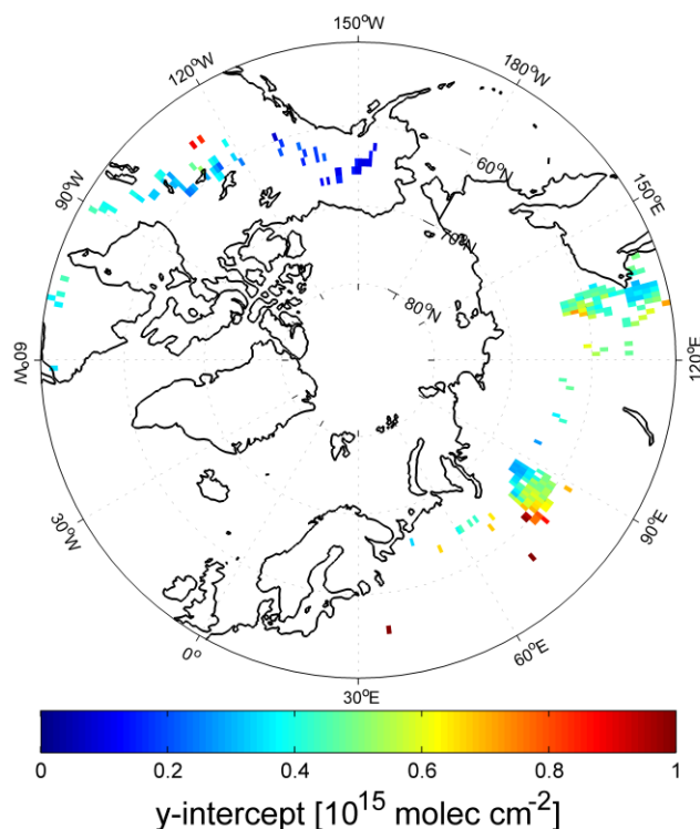
Fig. 3.3: Y-intercepts of the linear regression of TVC NO 2 against FRP for the six-year period (2007-2012). The y-intercepts representing the background levels in NO 2 columns are subtracted from the total tropospheric NO 2 columns (see Sect. 3.2.6). All pixels with a p-value < 0.05 and r > 0.3 are shown in the figure and used as a selection criterion for the estimation of FERs and EFs of NO x .
