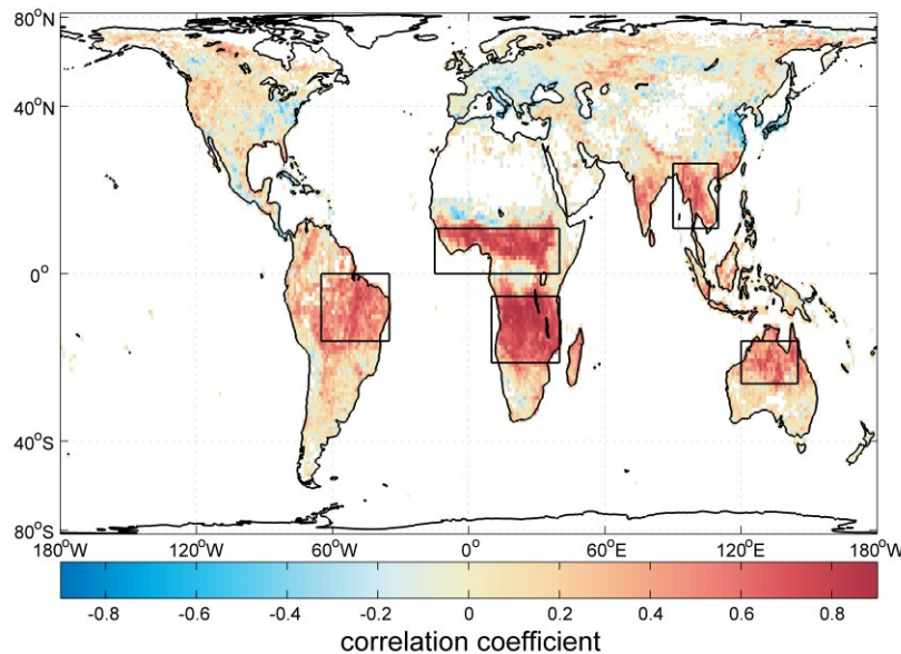
Fig. 2.2: Correlation coefficients ( r ) of the local temporal relationship between FRP and TVC NO 2 based on monthly averages from 2007-2011 on a 1° x 1° grid. Data are shown for the linear relationship observed between GOME-2 TVC NO 2 and MODIS Terra FRP.
