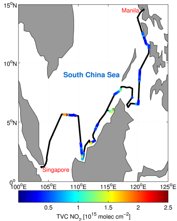
Fig. 6.12: Geographical map of color-coded TVC NO 2 as obtained from BREAM.
