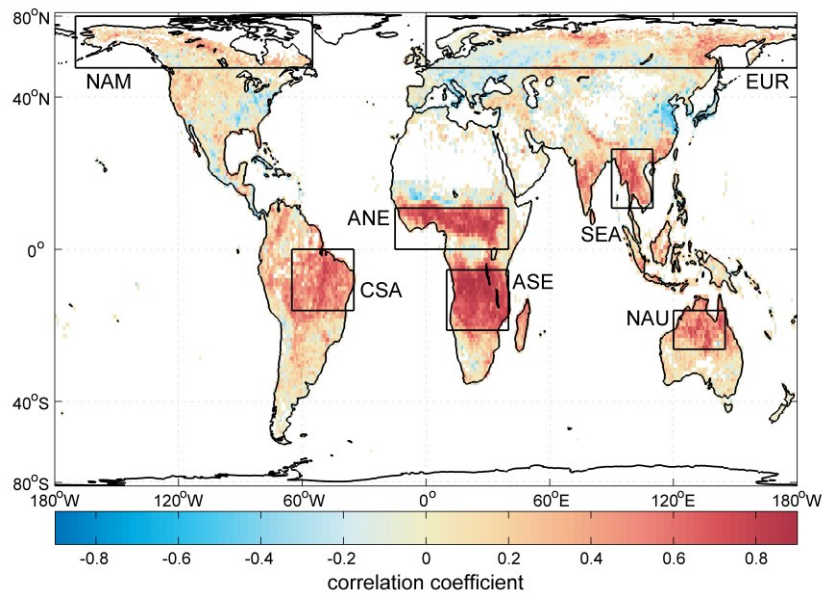
Fig. 4.1: Correlation coefficients ( r ) of the temporal relationship between TVC NO 2 and FRP based on monthly averages from 2007-2012 on a 1° x 1 grid. FERs of NO x are derived for the tropical and subtropical regions Africa north of Equator (ANE), Africa south of Equator (ASE), central South America (CSA), northern Australia (NAU), and Southeast Asia (SEA) (see Table 2.1). The boreal regions Eurasia (EUR) and North America (NAM) are defined in Table 3.1.
