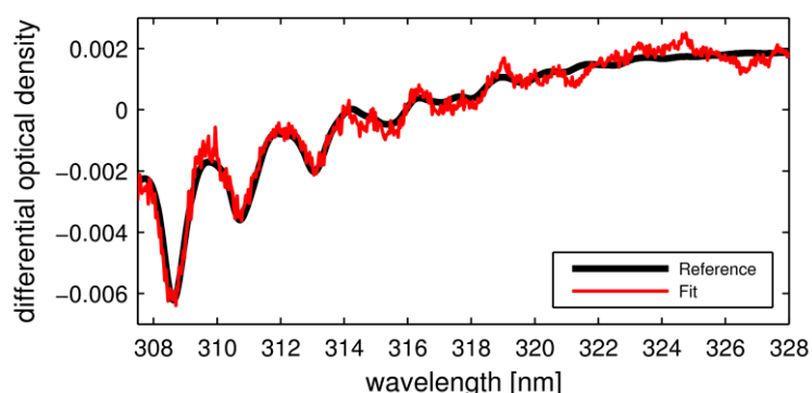
Fig. 6.8: Fit results of the SO 2 fit for a single measured spectrum taken in the morning of 17th November 2011 (01:20 UT) under elevated SO 2 pollution (SCD = 1.84 x 10 16 molec cm -2 ). The RMS of the residuals is 5 x 10 -4 . Here, the optical density of the reference (black line) and fit (red line) are retrieved at 2° elevation angle and at 53.33° solar zenith angle. Further explanations and definitions are given in the text.
