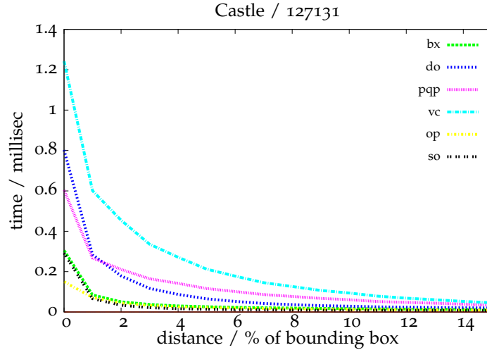
Figure 6.21: The results of the benchmark for the castle scenario in resolutions with 127131 vertices. The x -axis denotes the relative distance between the objects, where 1.0 is the size of the object. Distance 0.0 means that the objects are almost touching but do not collide. The abbreviations for the libraries are as follows: bx=BoxTree, do=Dop-Tree, pqp=PQP, vc=V-Collide, op=Opcode, so=FreeSOLID. The ABB-based algorithms perform best in this kind of scenarios.
