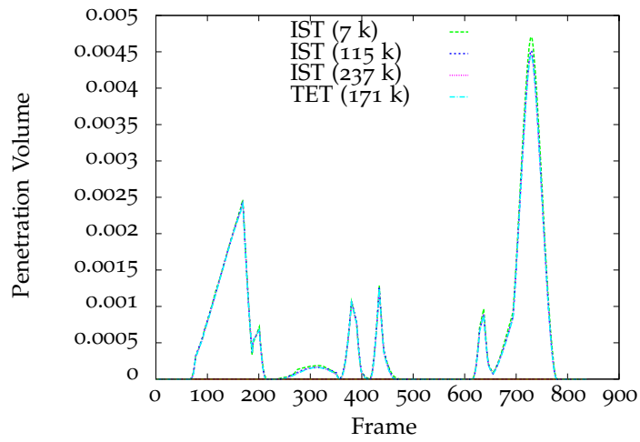
Figure 5.25: Penetration volume per frame in the bolt scene.
