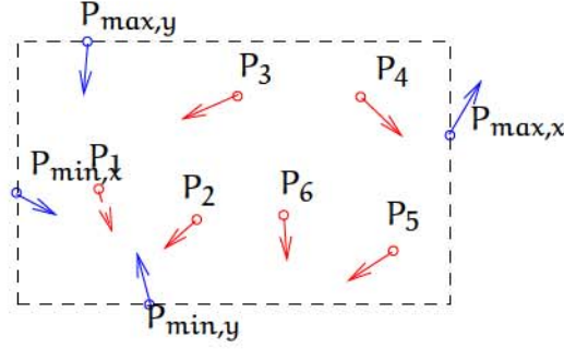
Figure 3.1: Assume a set of moving points in the plane. P_{\{\max,\min\},\{x,y\}} for the current bounding volume of this points. At some time, P_5 will become smaller than P_{\min,y} , this causes an event.
