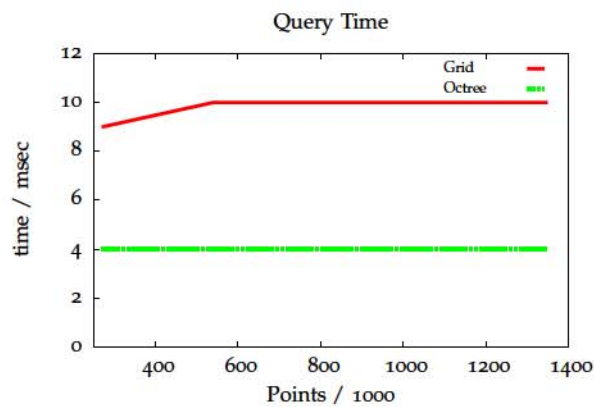
Figure 7.15: Average query time for point clouds with respect to the size of the point cloud. The cell size was set to 8 cm.
