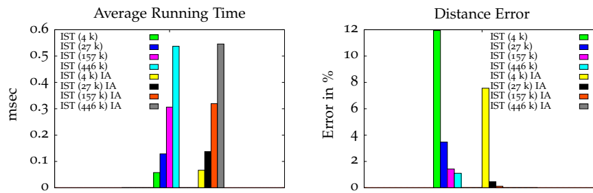
Figure 5.26: Pig scene: average and maximum time/frame (Left), relative error compared to accurate penetration volume (Right).
