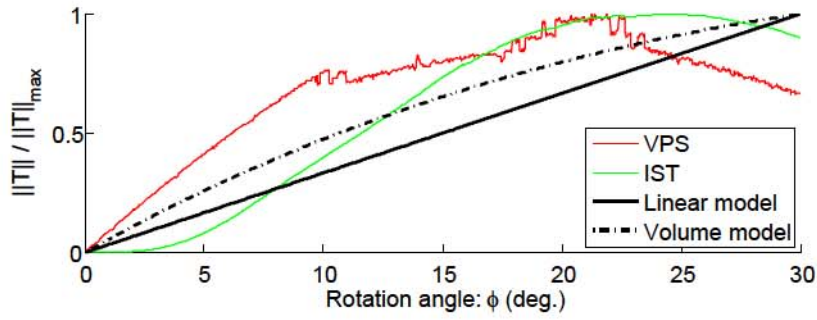
Figure 6.40: Torques in Scenario III.
