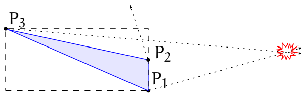
Figure 3.4: To keep the hierarchy valid when a leaf event happens, we have to replace the old maximum P_2 by the new maximum P_1 , and compute the time, when one of the other vertices of the polygon, P_2 or P_3 will become larger than P_1 . In this example this will be P_3 .
