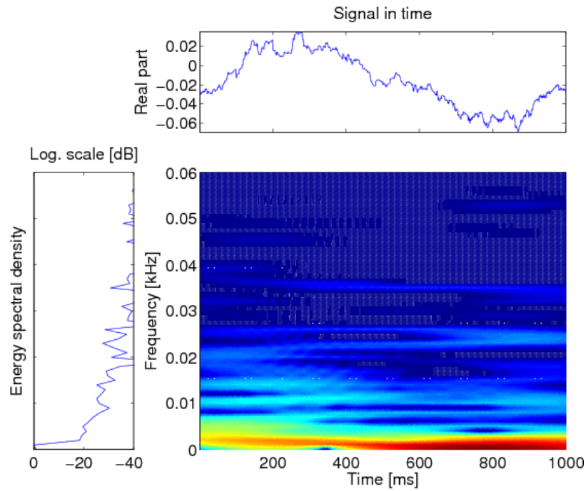
Figure 6.43: Noise in the force signal of the VPS algorithm. The colored picture shows the time frequency domain: the colors decode the intensity of the frequency, where dark blue remarks an intensity of zero.
