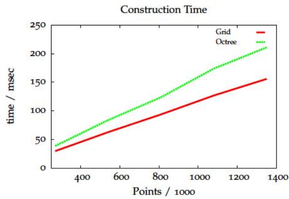
Figure 7.14: Average construction time for point clouds with respect to the size of the point cloud. The cell size was set to 8 cm.
