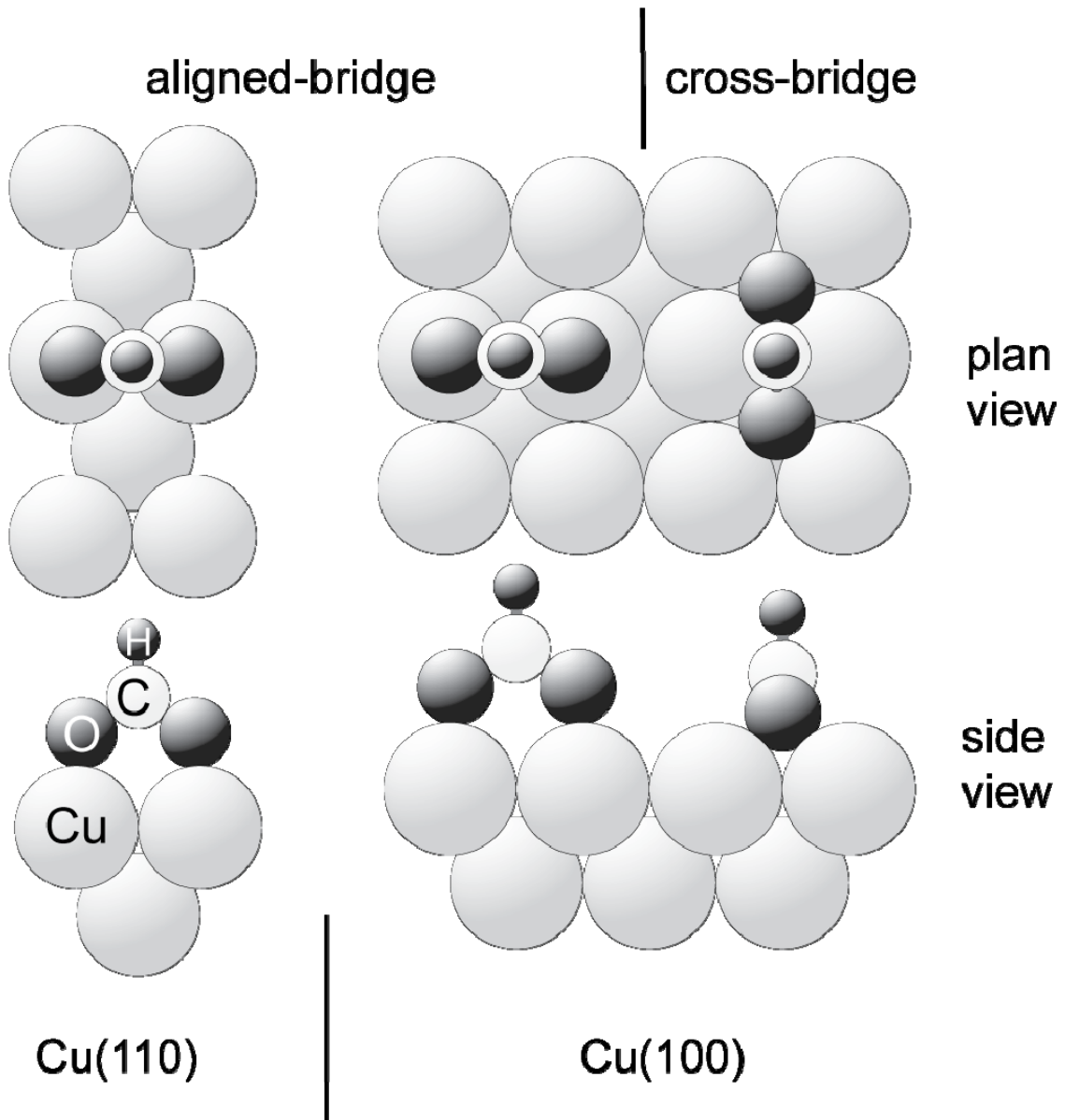
Fig. 1 The local aligned-bridge adsorption sites of the formate ( \text{HCOO}^- ) species on Cu(110) and Cu(100). Also shown is the cross-bridge site on Cu(100) originally proposed as a 'new type of surface bond' but subsequently shown to be incorrect.
