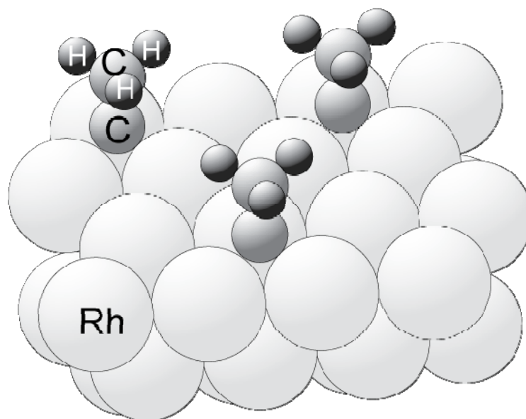
Fig. 6. The structure of the Rh(111)(2x2)-CCH 3 surface phase
