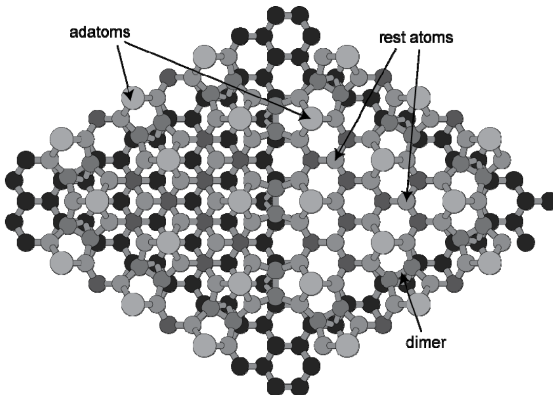
Fig. 8 Plan view of the Si(111)(7x7) 'DAS' clean surface structure. The different atomic radii and levels of grey shading correspond to different layers in the near-surface region.
