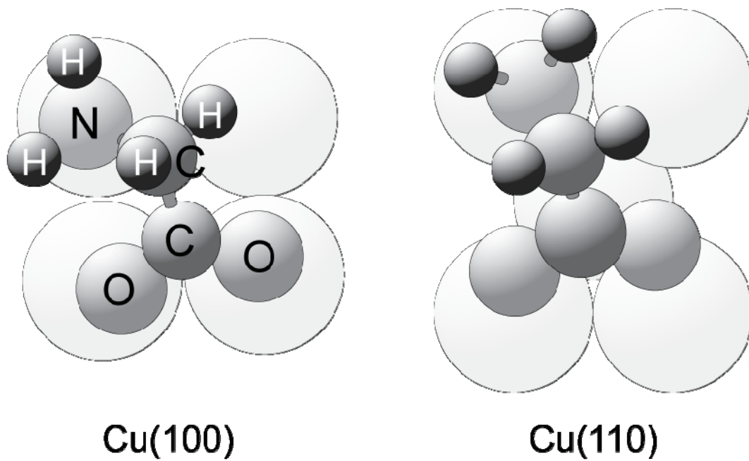
Fig. 3 Plan views of the local geometry of glycinate (deprotonated glycine, NH 2 CH 2 COO) on Cu(100) and Cu(110).
