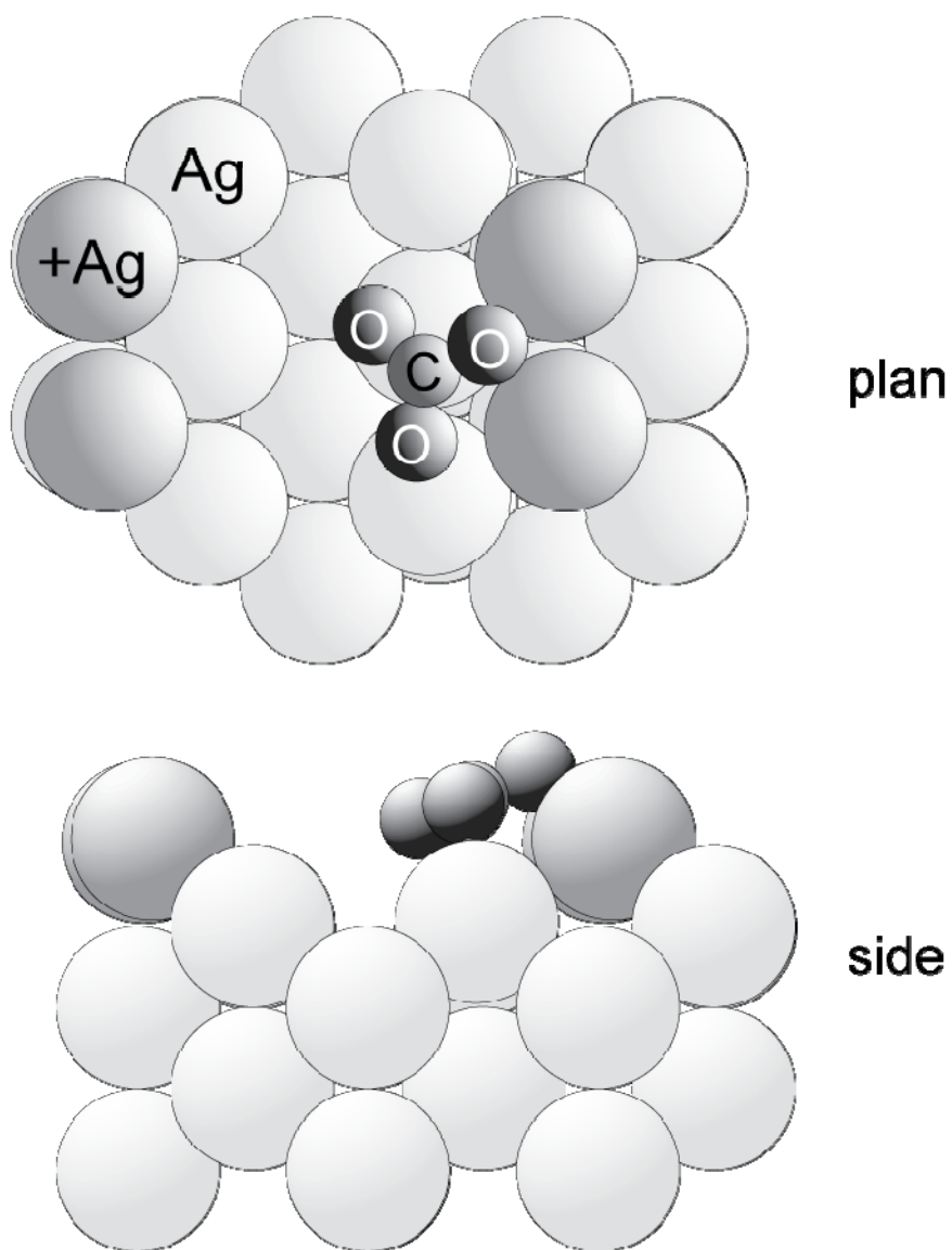
Fig. 4 The local structure of the carbonate, \text{CO}_3 , species on \text{Ag}(110) . Atoms labelled '+Ag' are in rows of Ag adatoms on the bulk-terminated \text{Ag}(110) structure.
