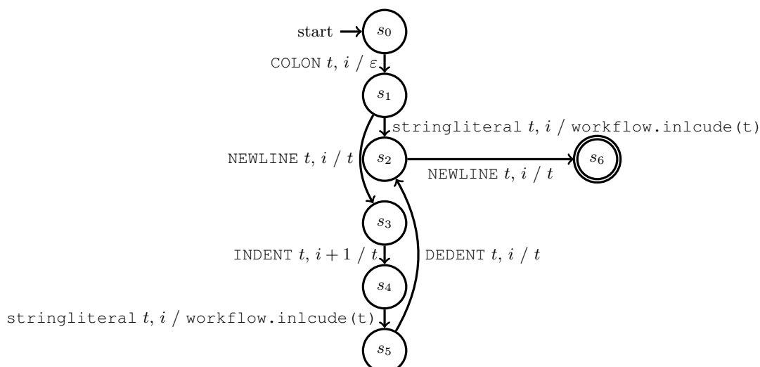
Figure 4.2: Keyword automaton for the include keyword. Input and output are denoted separated by a slash beside the transition. Input consists of a token with its type (e.g., COLON , NEWLINE , stringliteral ) and the current indentation level. For simplicity, the output may refer to the input token given as t . Unexpected input shall lead to an error.
