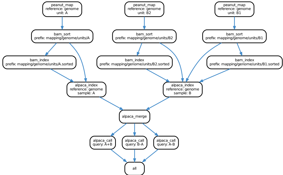
Figure 4.4: Example Job-DAG automatically generated with Snakemake and Graphviz.
