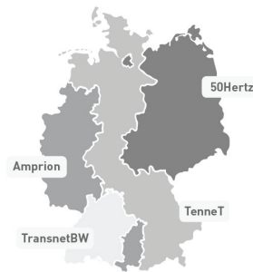
Fig. 5: control areas in Germany[www.netzregelverbund.de]
