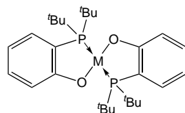
Abbildung 3.4: Bis-(2-(di-tert.-butyl-phosphanyl)-phenolato)-[O,P]-metall(II)
