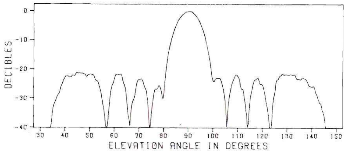
Figure 21. The Measured Principal Plane Far-Field Elevation Pattern of the Test Antenna
