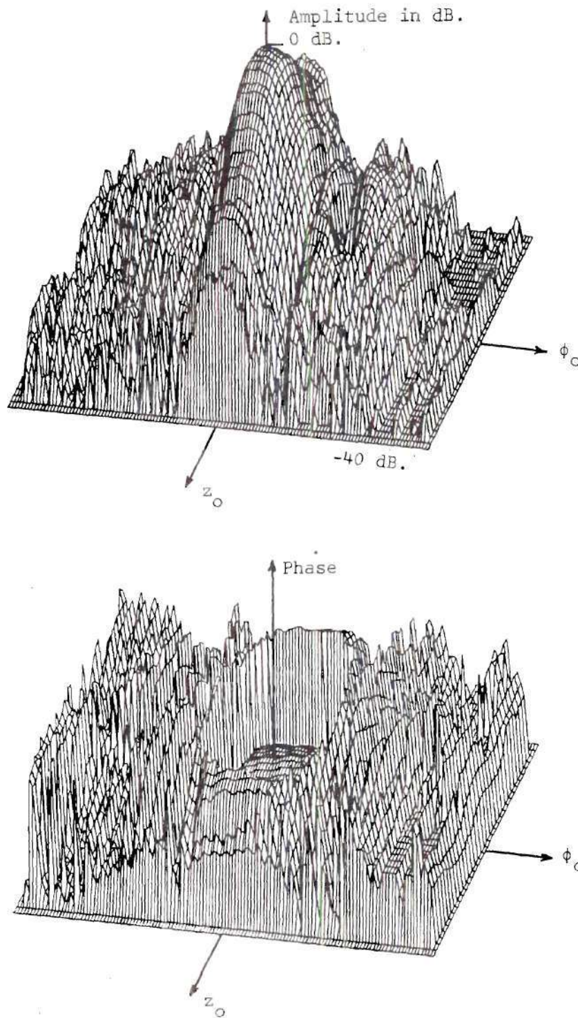
Figure 13. Near-Field Amplitude and Phase Patterns of E_\phi for Measurement Case One, Measured with the Open-End Waveguide Probe with the Antenna Mounted Vertically in the Cylinder
