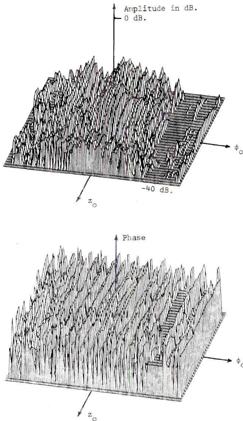
Figure 18. Near-Field Amplitude and Phase Patterns of E_z for Measurement Case Three, Measured with the Small Horn Probe with the Test Antenna Mounted Vertically in the Cylinder
