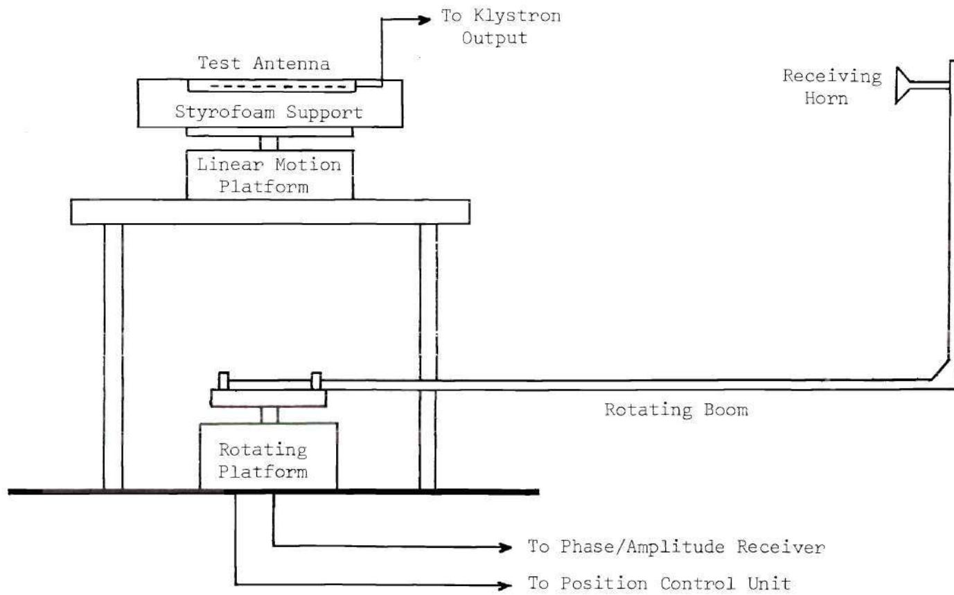
Figure 12. Diagram of the Phase Center Range
