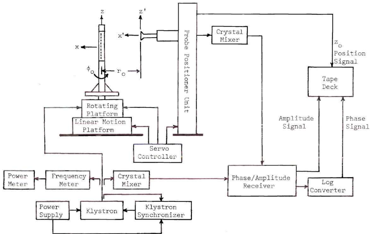
Figure 11. Diagram of the Near-Field Measurement System
