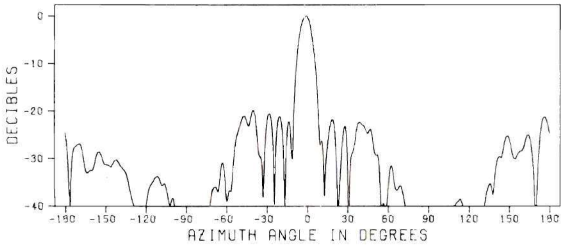
Figure 26. The Calculated Far-Field Amplitude Pattern of E_\theta for Measurement Case Four
