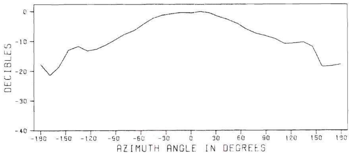
Figure 22. The Measured Principal Plane Far-Field Azimuth Pattern of the Test Antenna
