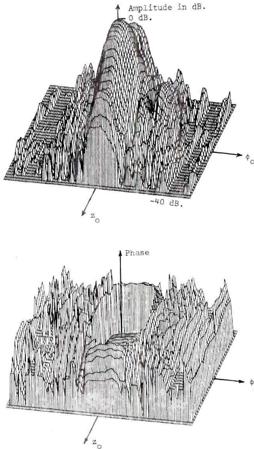
Figure 17. Near-Field Amplitude and Phase Patterns of E_\phi for Measurement Case Three, Measured with the Small Horn Probe with the Test Antenna Mounted Vertically in the Cylinder
