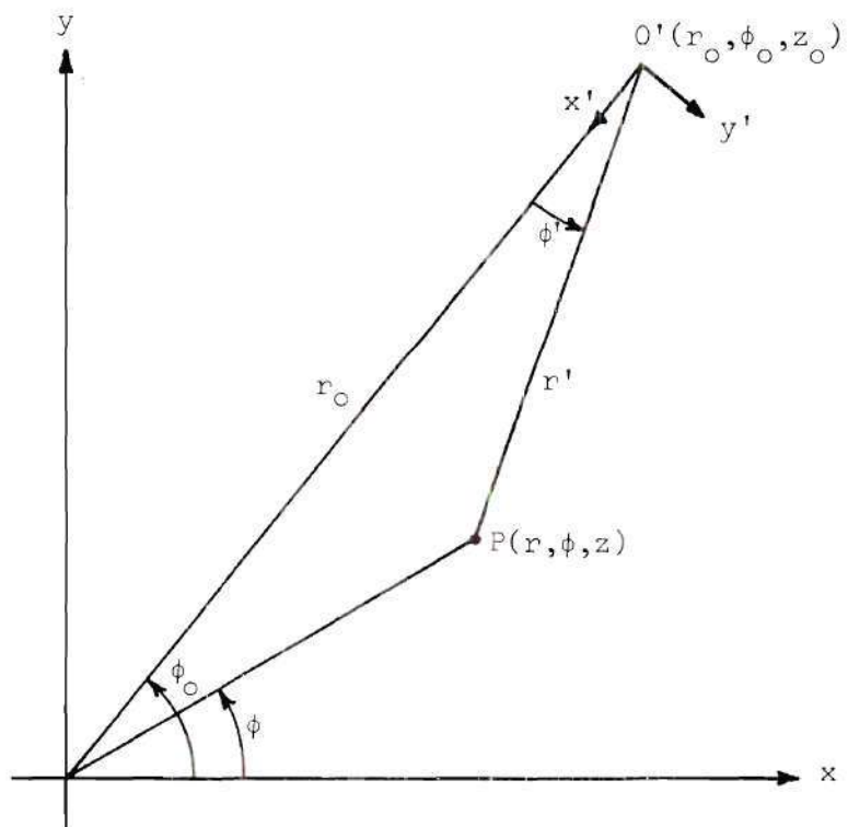
Figure 31. Coordinate System for the Cylindrical Wave Translation Theorems
