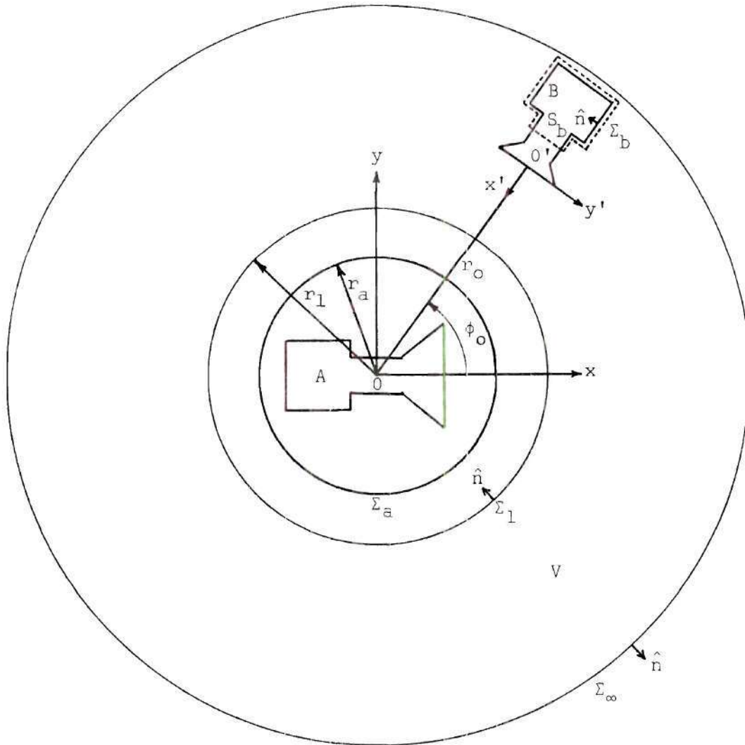
Figure 3. Geometry for the Probe Compensation Derivation
