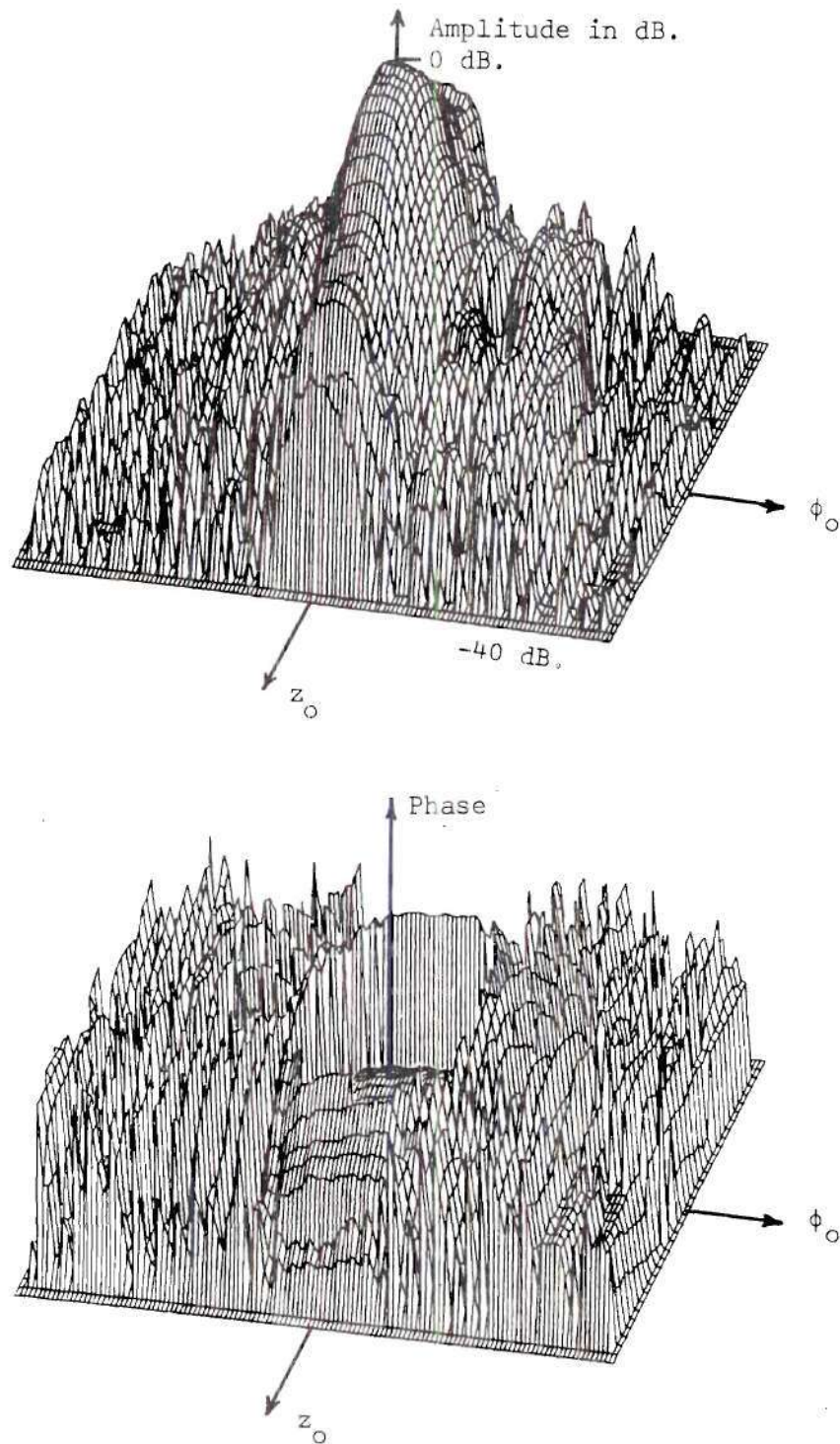
Figure 15. Near-Field Amplitude and Phase Patterns of E_\phi for Measurement Case Two, Measured with the Open-End Waveguide Probe with the Antenna Mounted Vertically in the Cylinder
