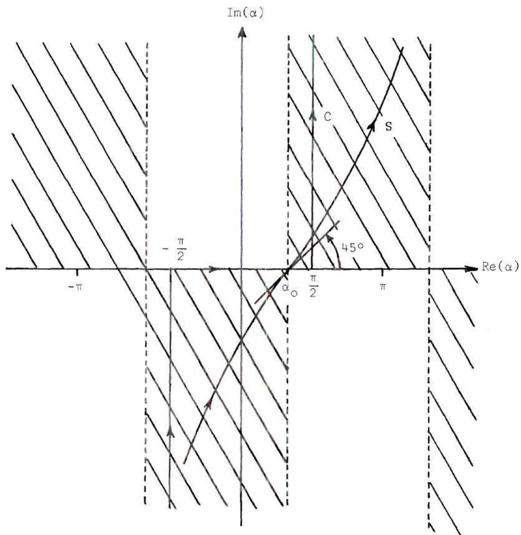
Figure 30. The Path of Steepest Descent
