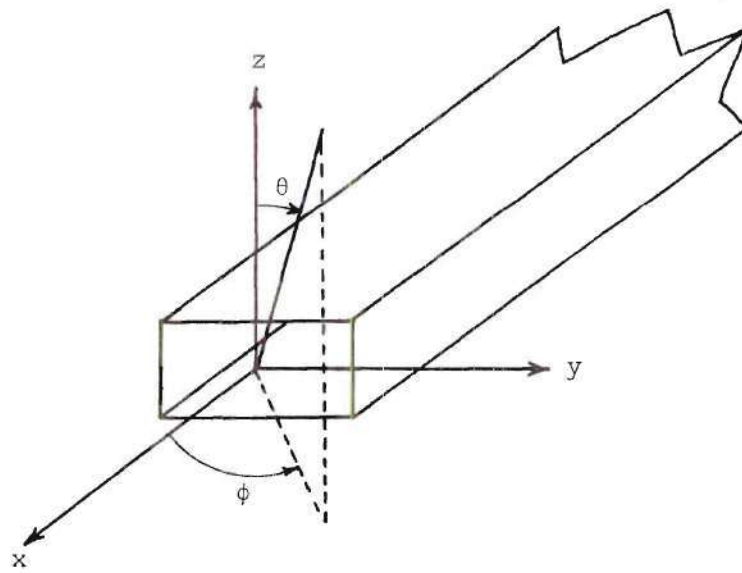
Figure 5. Coordinate System for the Probe Antenna
