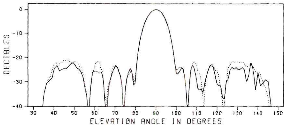
(a) Elevation Pattern of E_\phi — Calculated, ..... Measured
