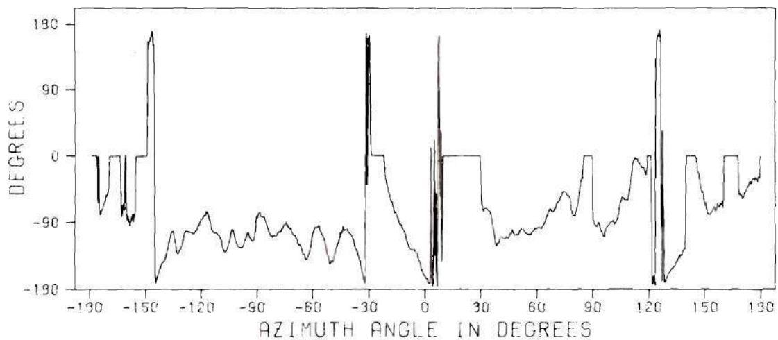
Figure 19. Near-Field Amplitude and Phase Patterns of E_\phi for Measurement Case Four, Measured with the Open-End Waveguide Probe with the Antenna Mounted Horizontally in the Cylinder
