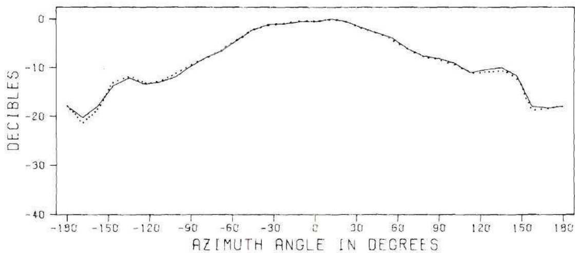
(b) Azimuth Pattern of E_\phi — Calculated, ..... Measured
