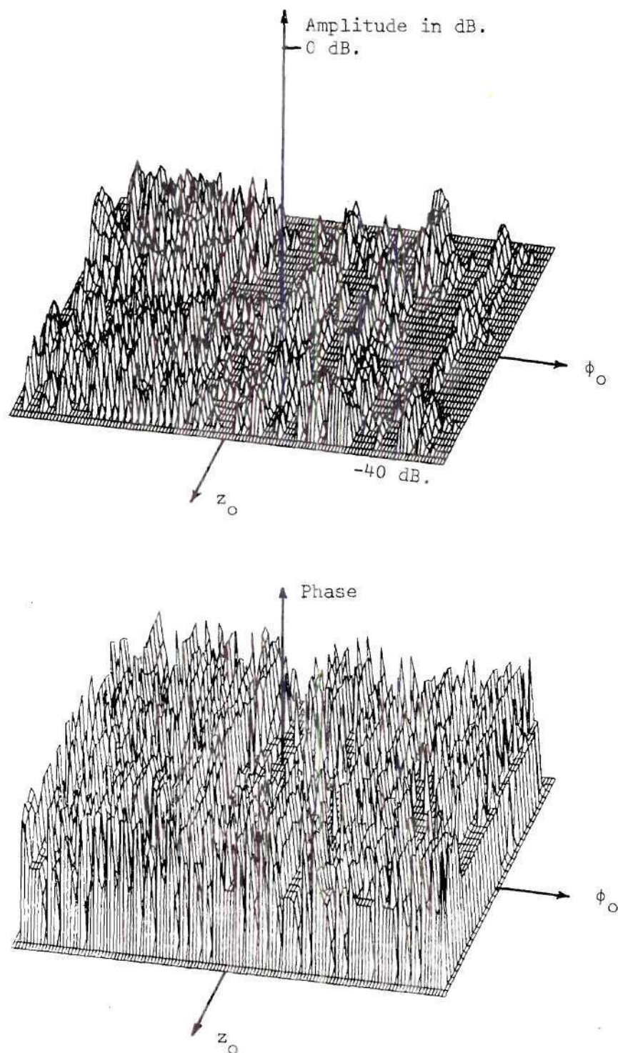
Figure 16. Near-Field Amplitude and Phase Patterns of E_z for Measurement Case Two, Measured with the Open-End Waveguide Probe with the Test Antenna Mounted Vertically in the Cylinder.
