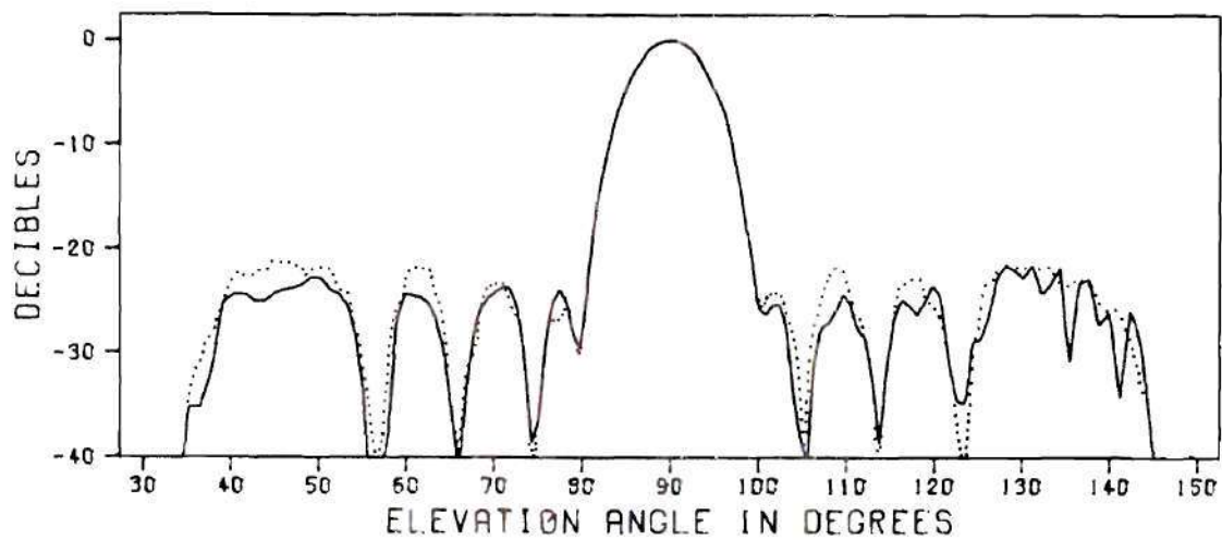
(a) Elevation Pattern of E_\phi — Calculated, ..... Measured
