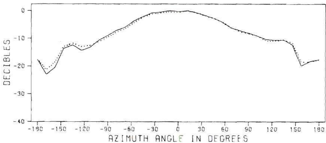
(b) Azimuth Pattern of E_\phi — Calculated, ..... Measured
