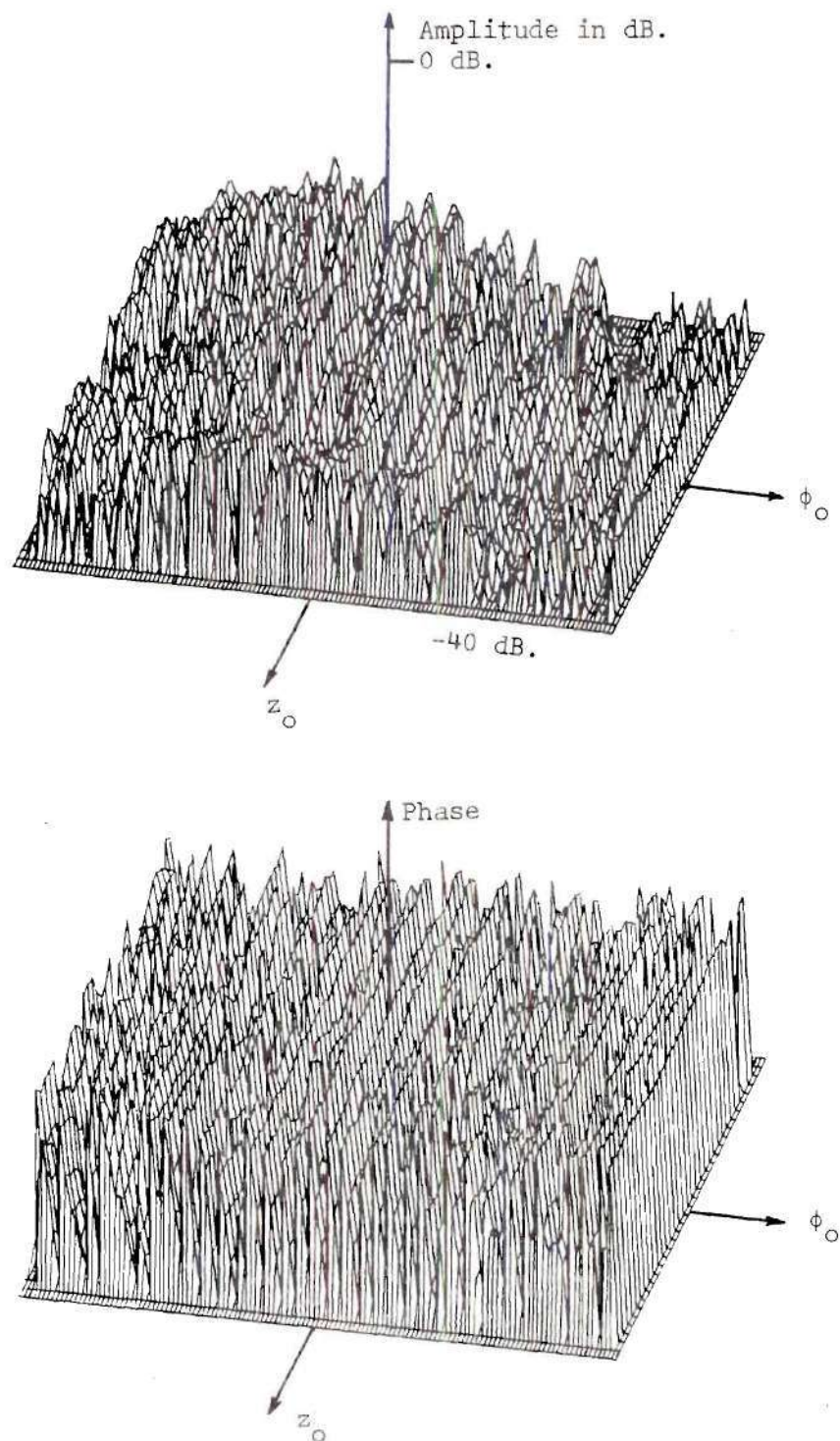
Figure 14. Near-Field Amplitude and Phase Patterns of E_z for Measurement Case One, Measured with the Open-End Waveguide Probe with the Antenna Mounted Vertically in the Cylinder
