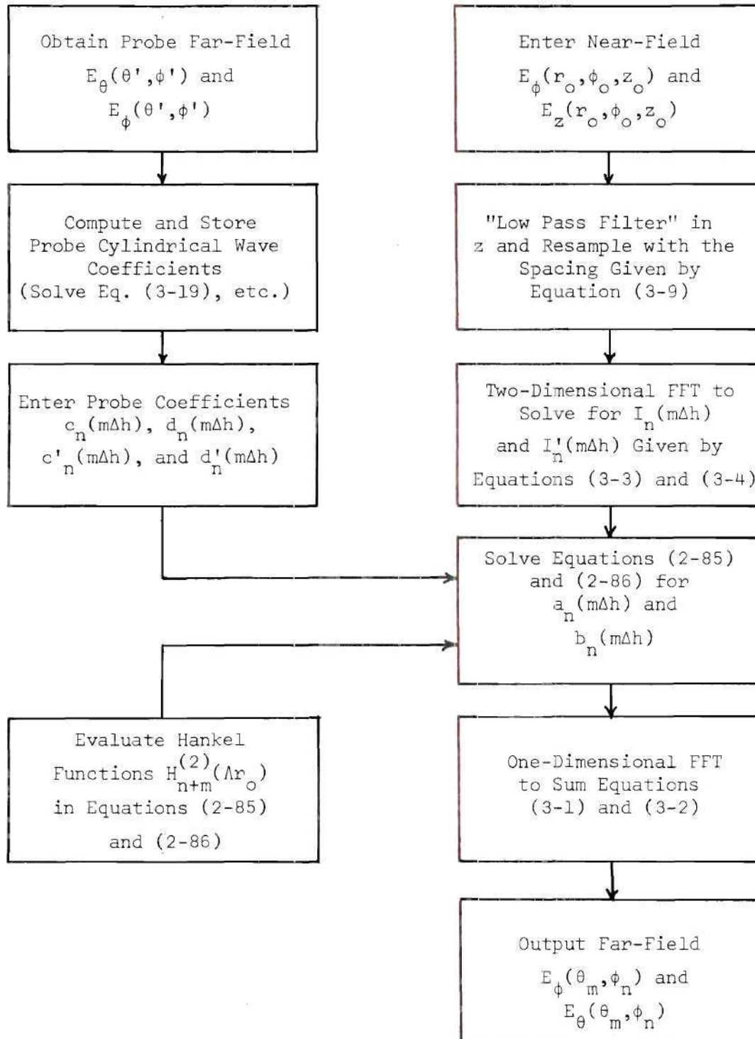
Figure 4. Flow-Diagram for the Far Field Evaluation
