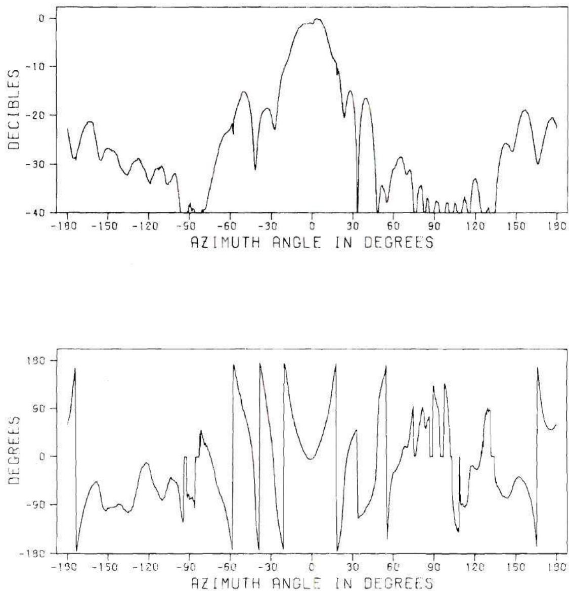
Figure 20. Near-Field Amplitude and Phase Patterns of E_z for Measurement Case Four, Measured with the Open-End Waveguide Probe with the Antenna Mounted Horizontally in the Cylinder
