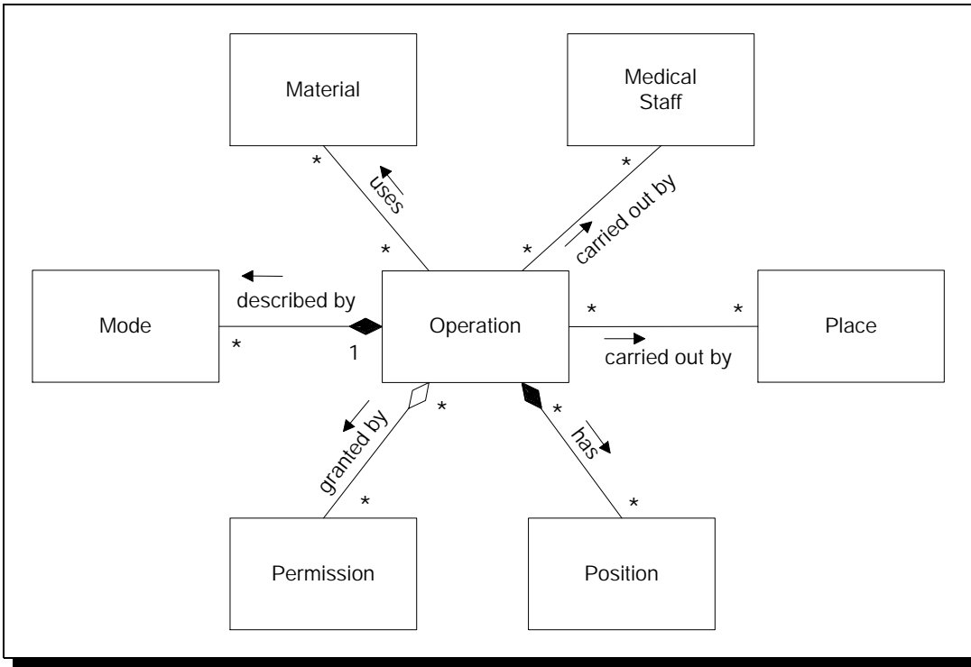
Figure 3: Associations of medical operations in angiopathy.
