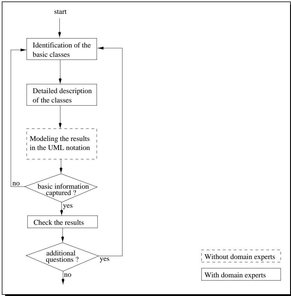
Figure 1: Our iterative process for domain analysis.
