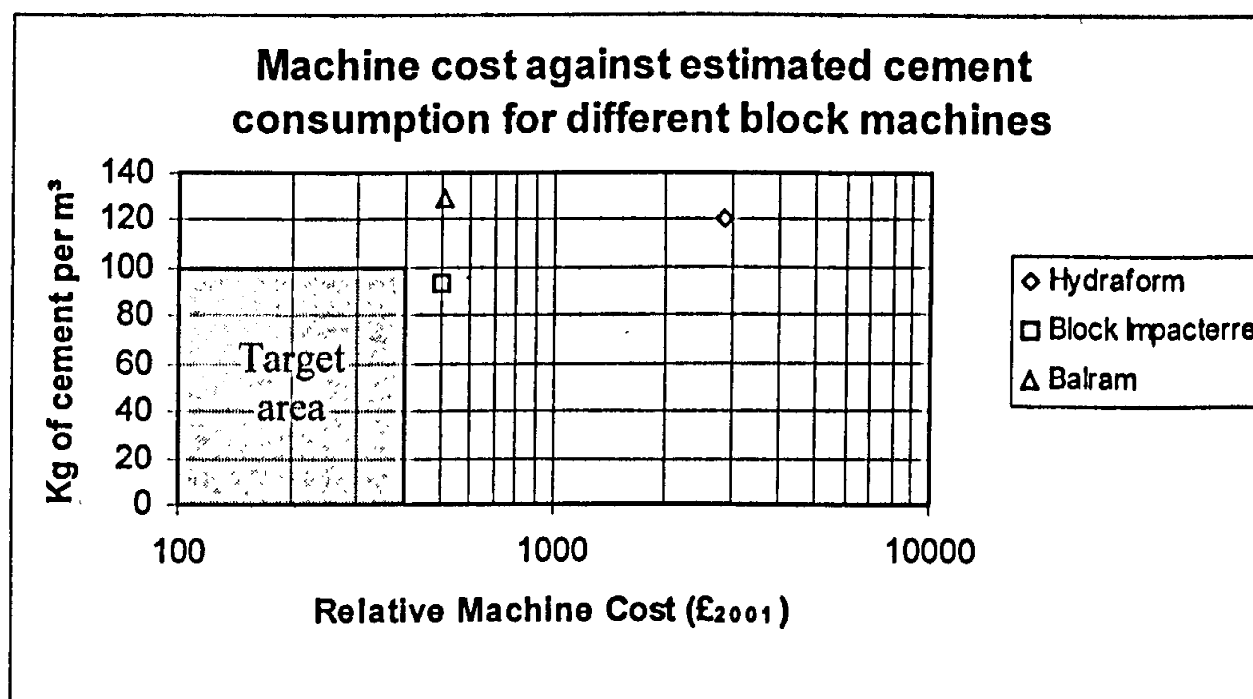
Figure 8.1 – Re assessment of CSSB machines using recent data
