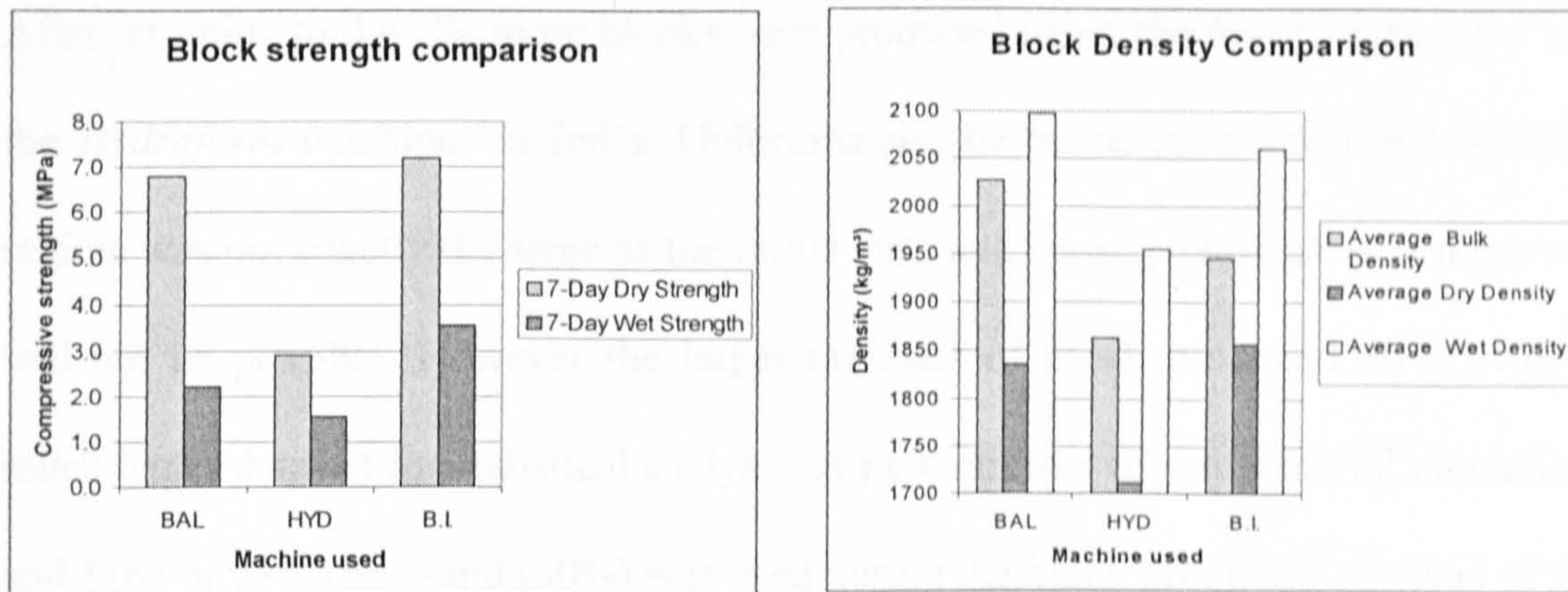
Figure 7.3 – Initial results for comparing block machines
