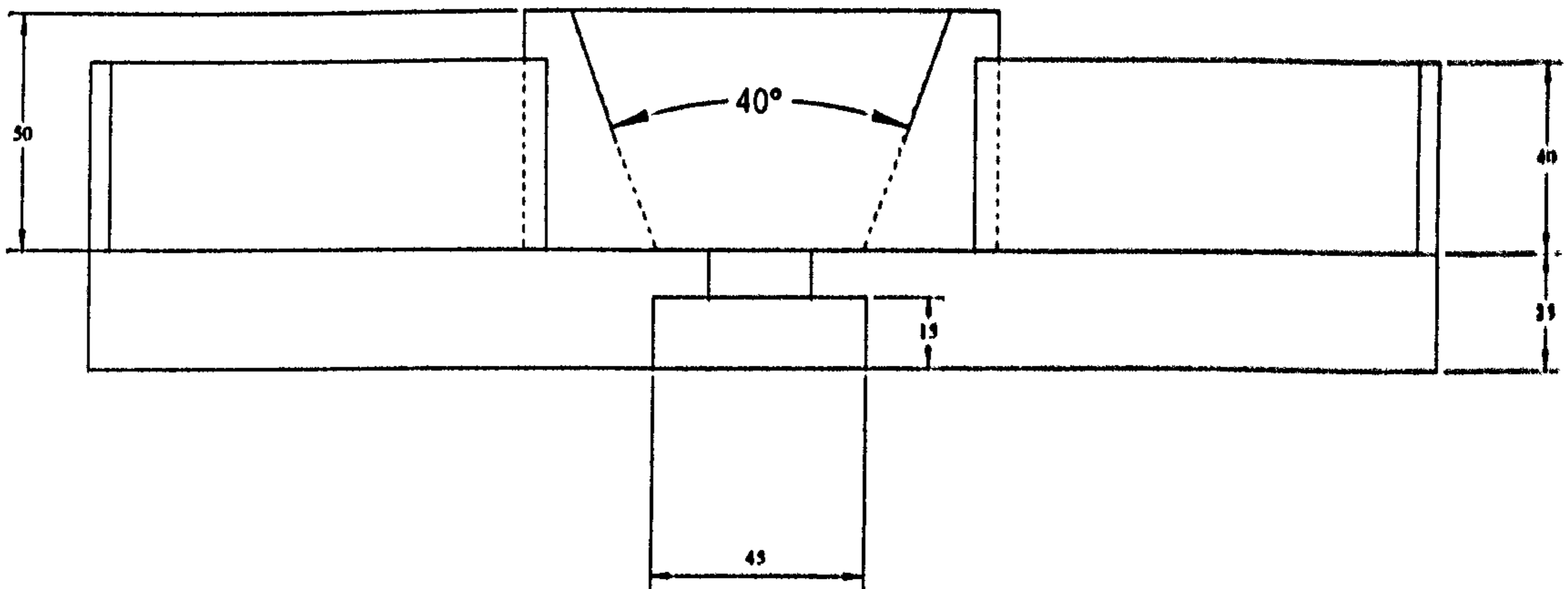
Metal impactor base details
