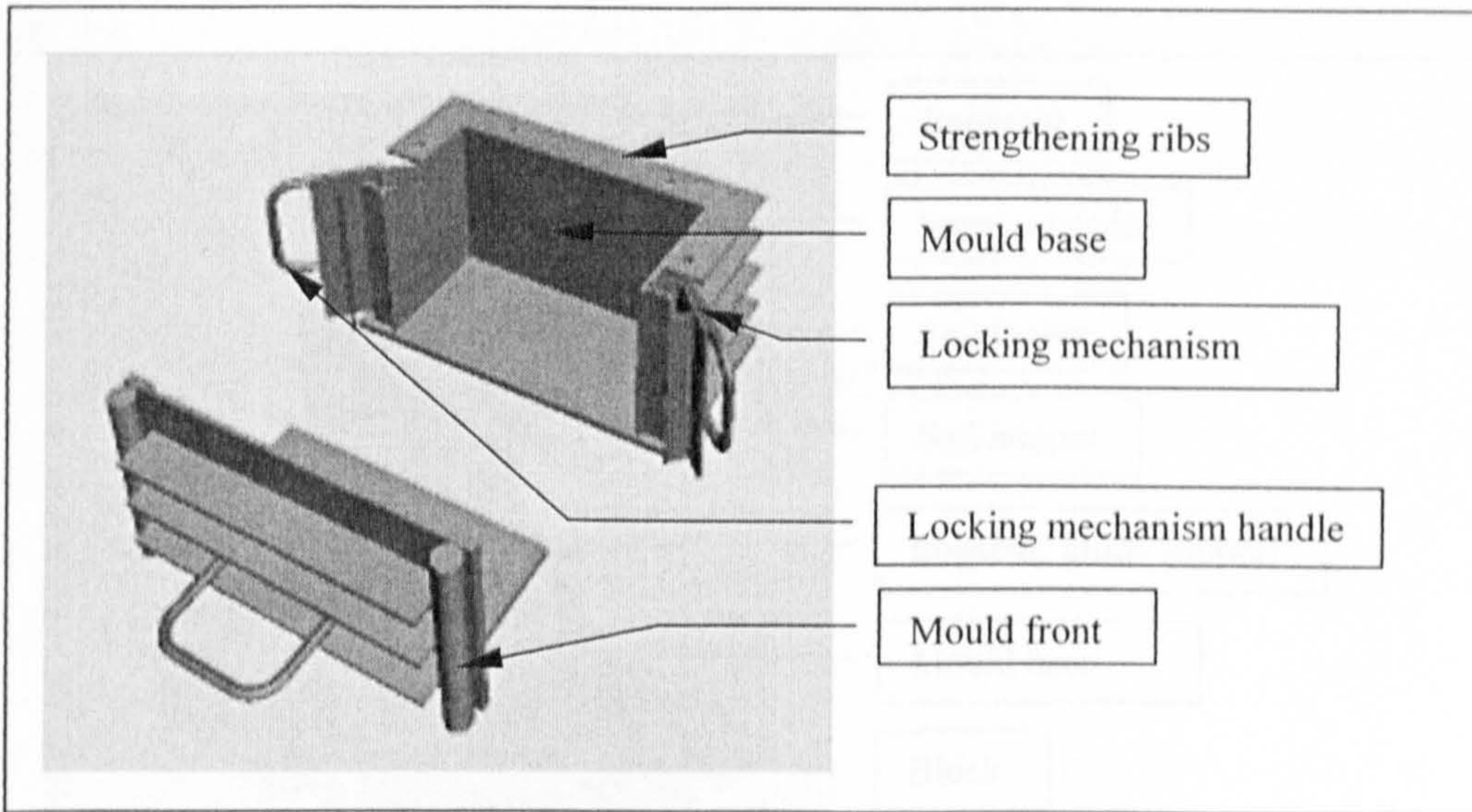
Figure 6.6a – CAD model of the mould
