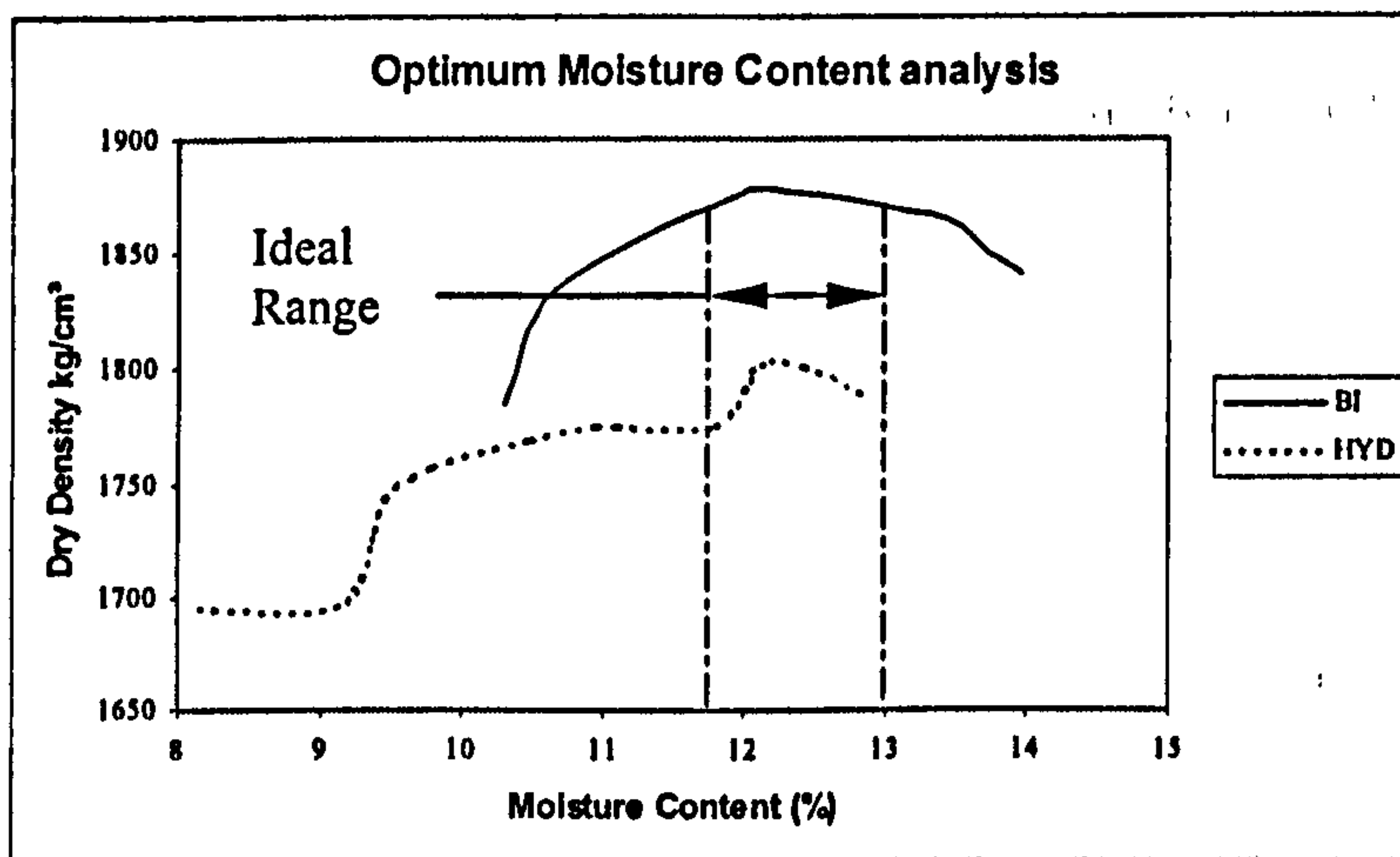
Figure 7.4 – OMC analysis of two machines
