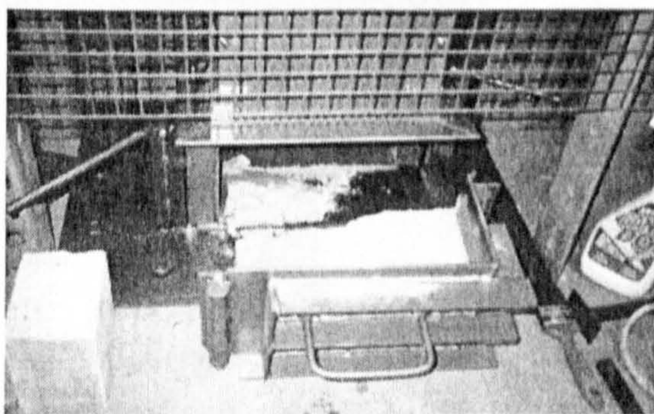
Two part mould in use, illustrating the problem with block ejection
