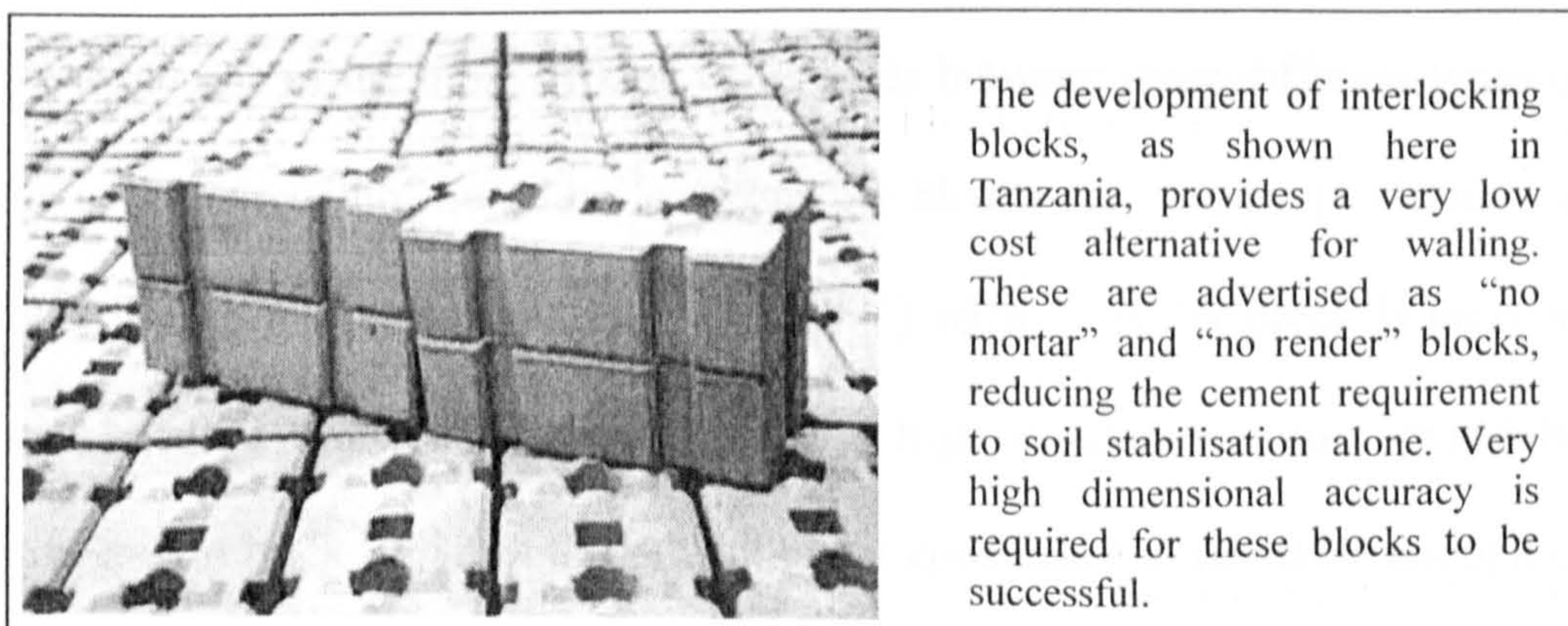
Figure 2.4 – Interlocking CSSB
