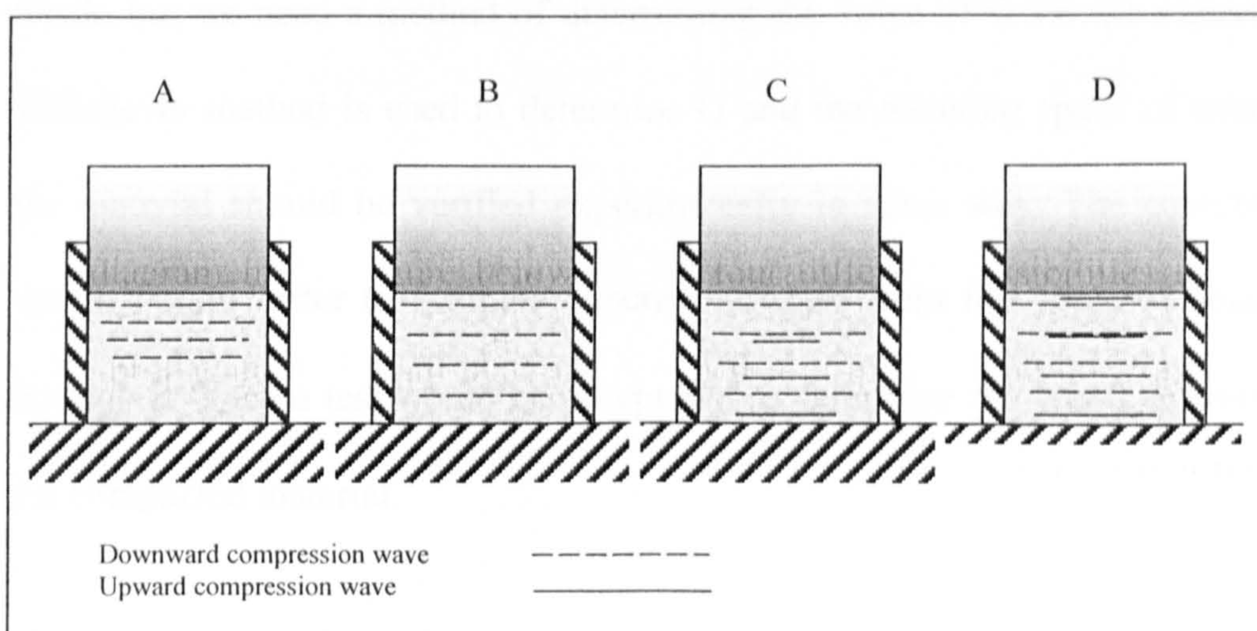
Figure 5.1 – Compression wave propagation during compaction
