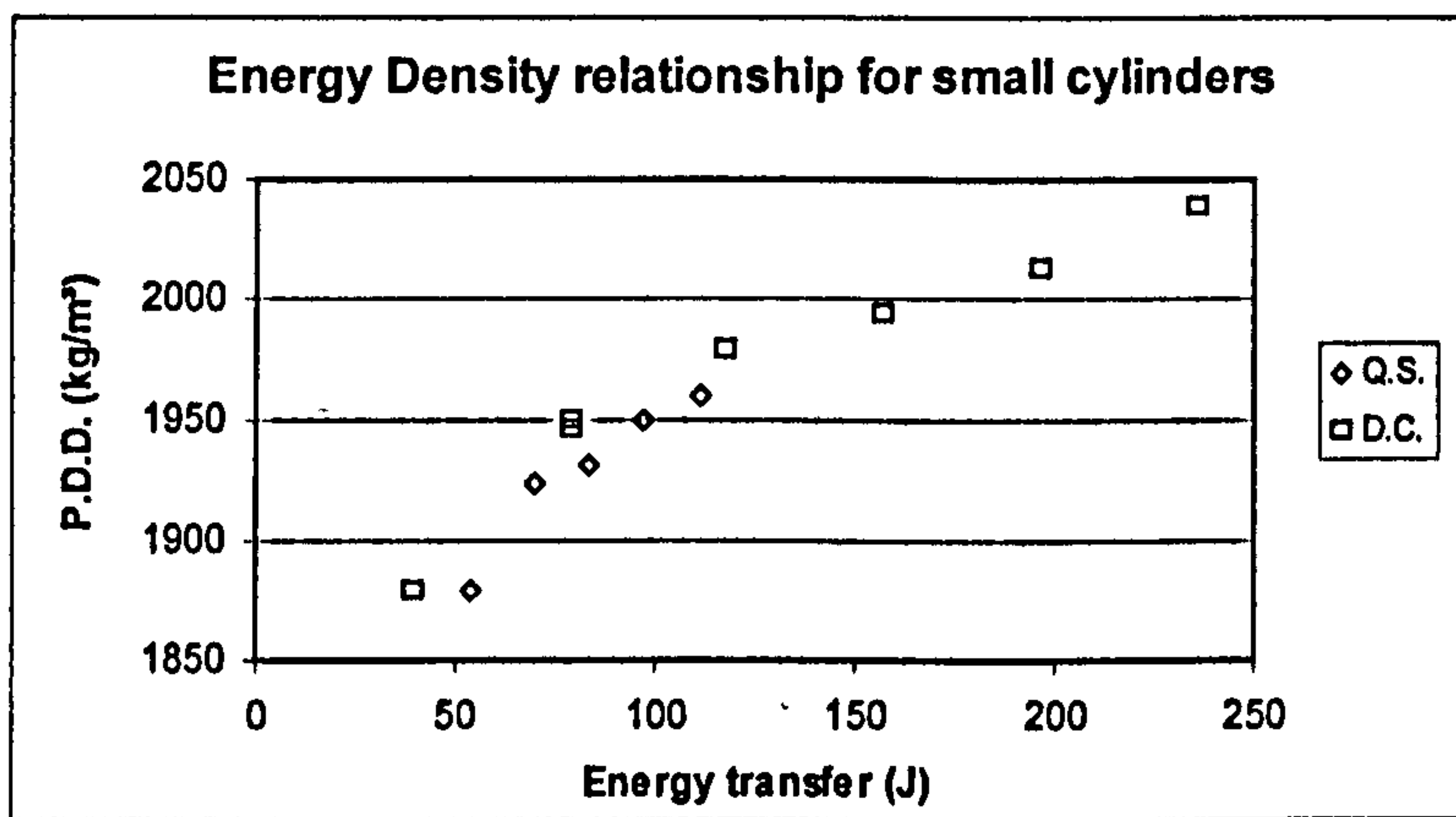
Figure 4.16 – Comparison of energy transfer for small cylinder production
