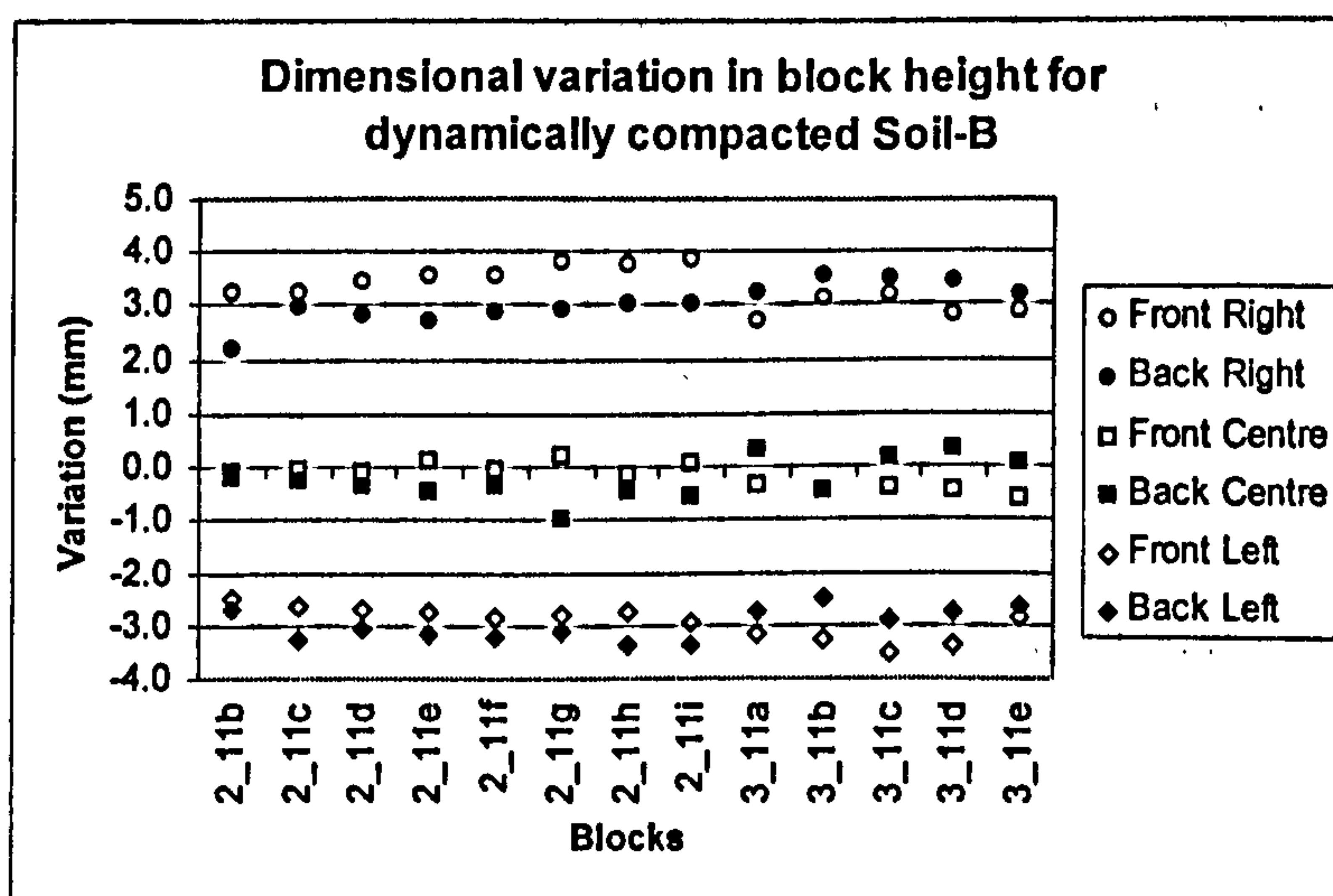
Figure 4.13 – Height variation of dynamically compacted blocks
