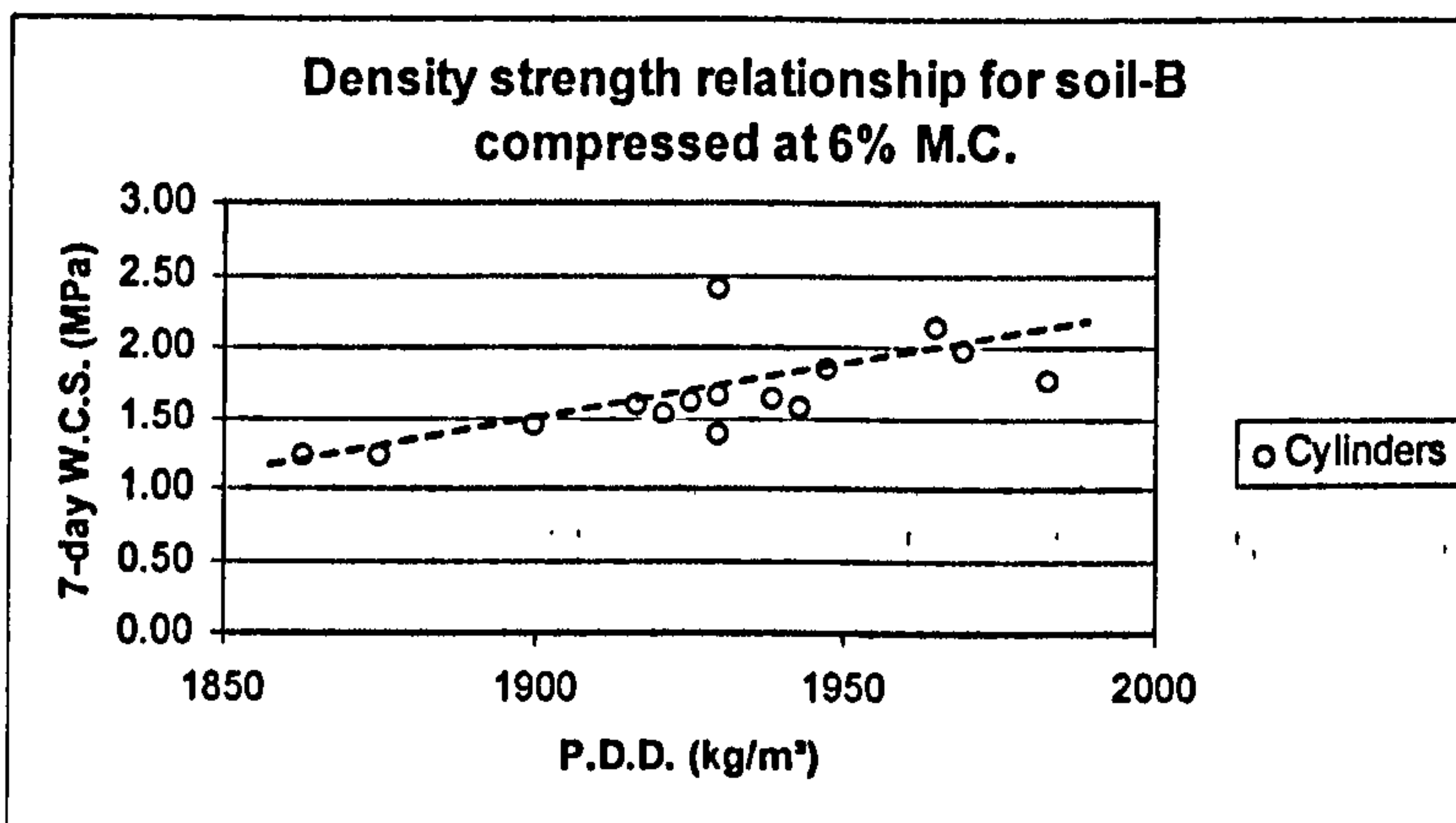
Figure 3.7 – Strength density relationship for soil-B at 6% M.C.
