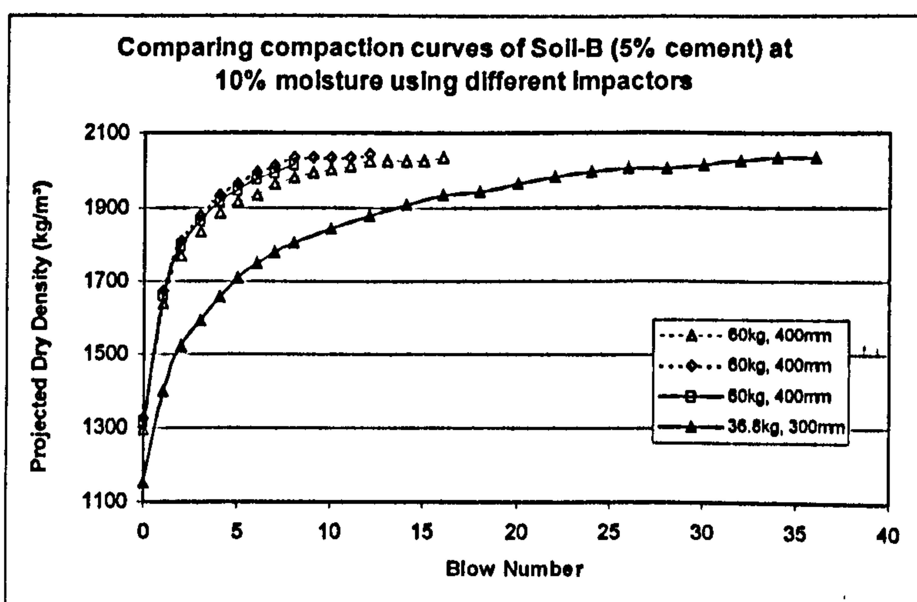
Figure 4.10a – Compaction curves for different impactors
