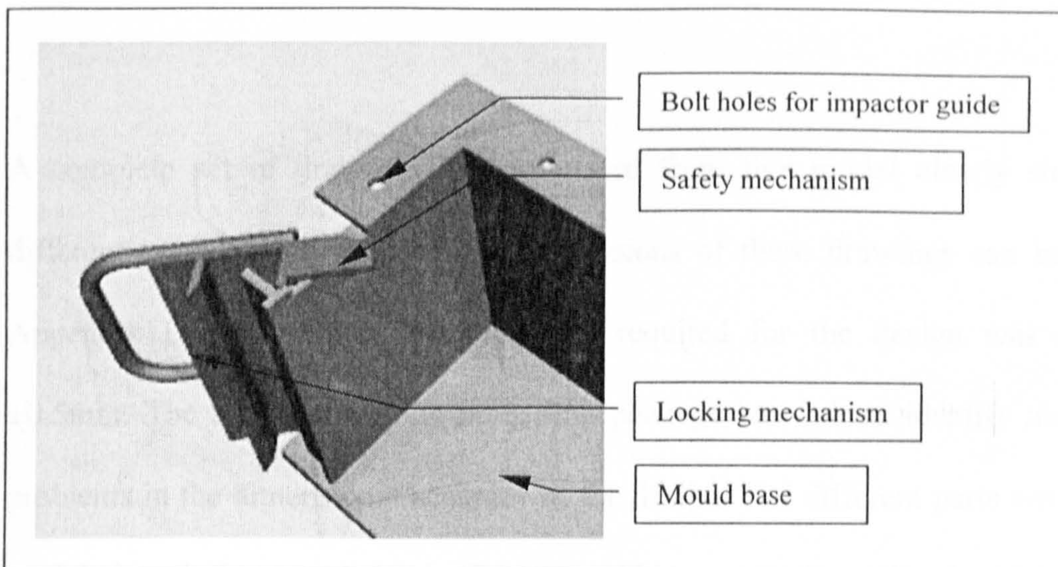
Figure 6.6b – CAD model of the mould safety mechanism
