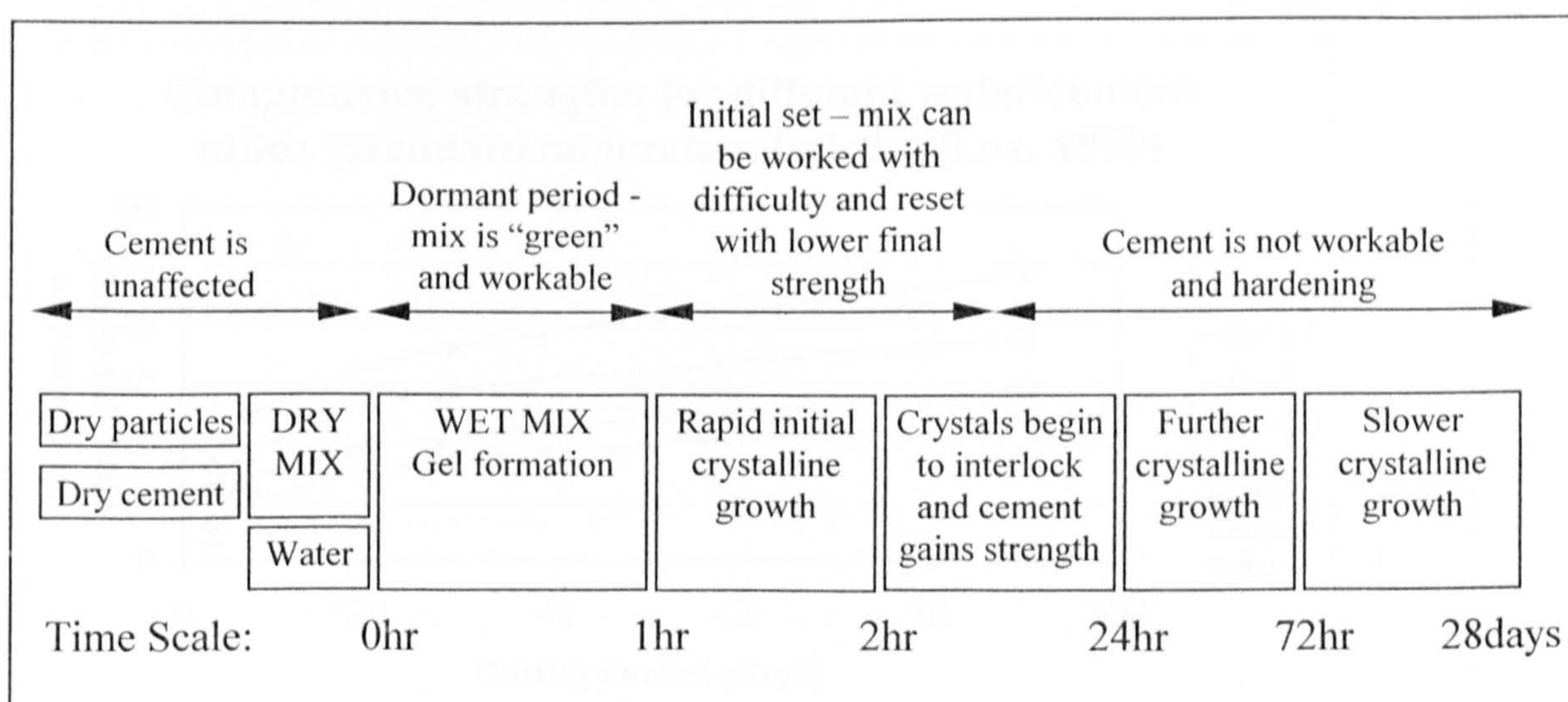
Figure 2.7 – Flow chart of the cement hardening process
