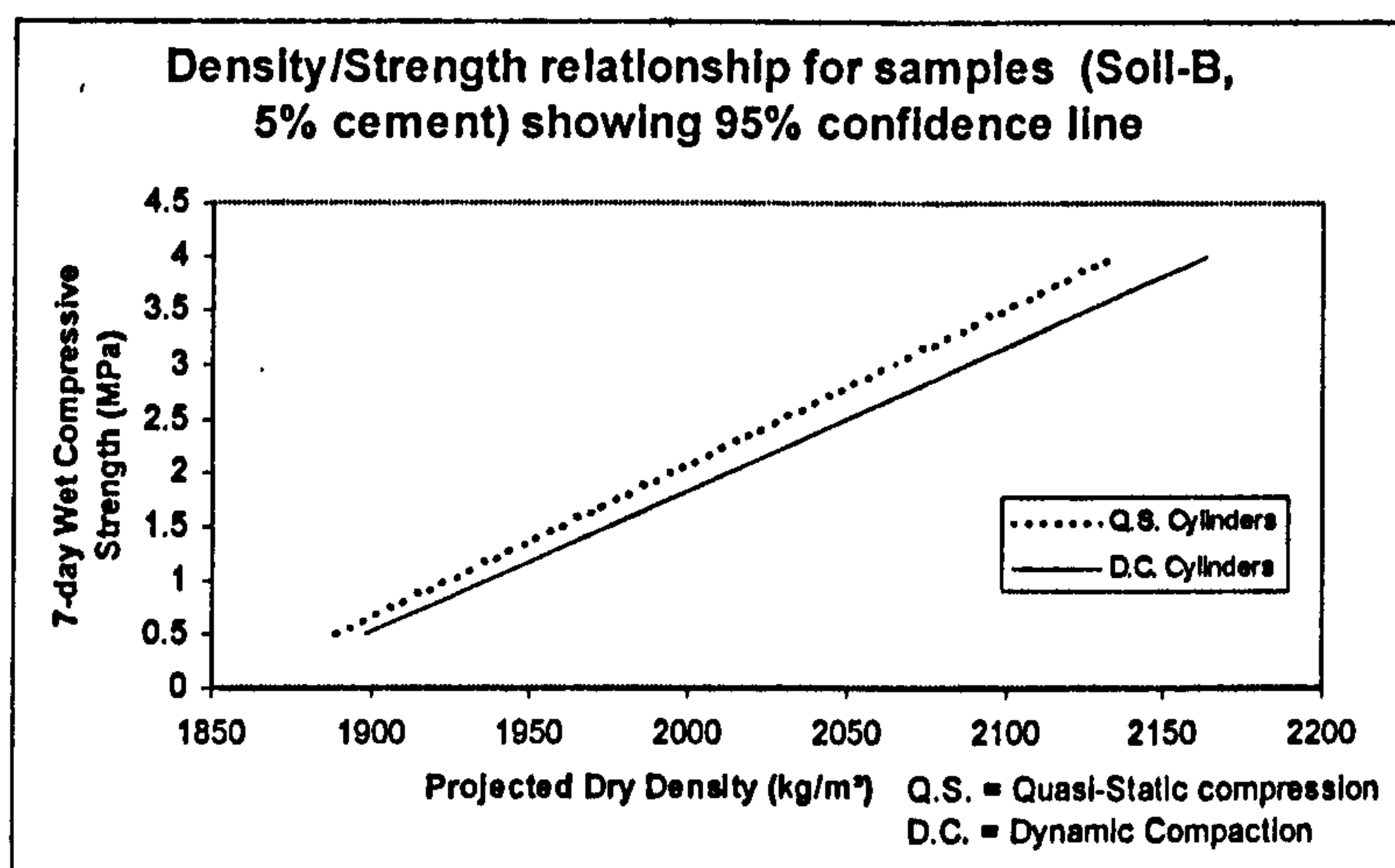
Figure 4.7 – 95% Confidence lines for density/strength relationship for cylinders
