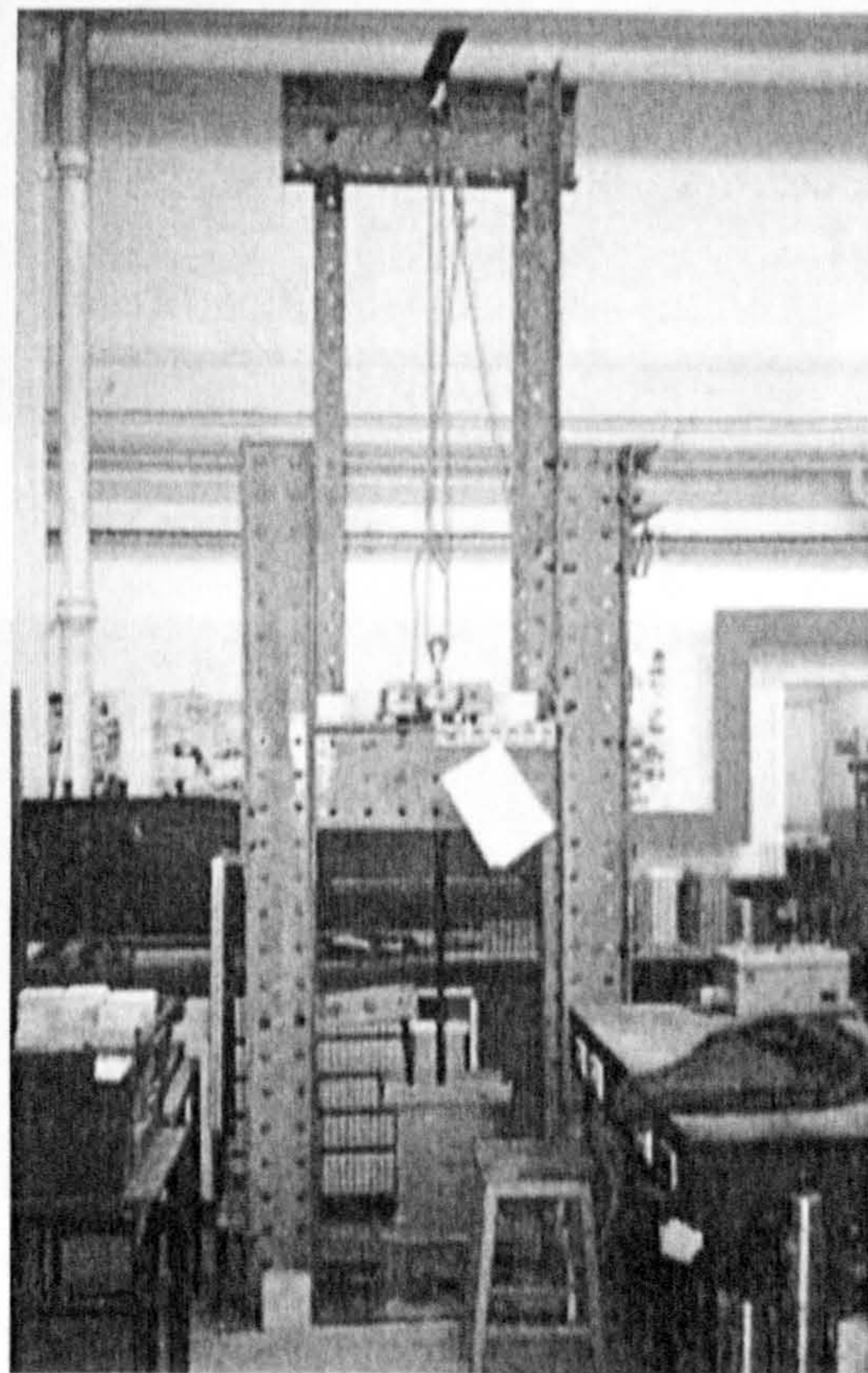
Modified test rig (steel impactor)
