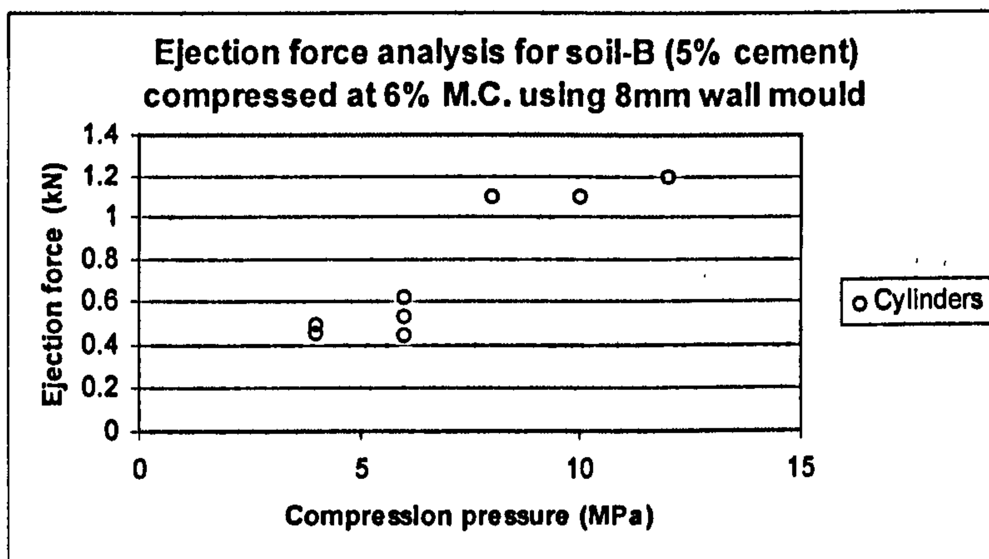
Figure 3.9 – Ejection force analysis for different compression forces
