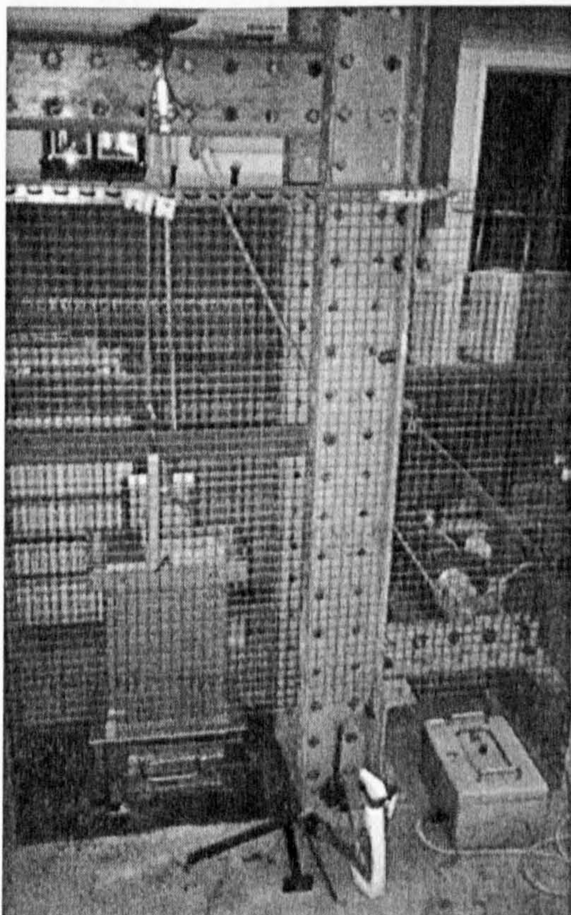
Original test rig (cement impactor)
