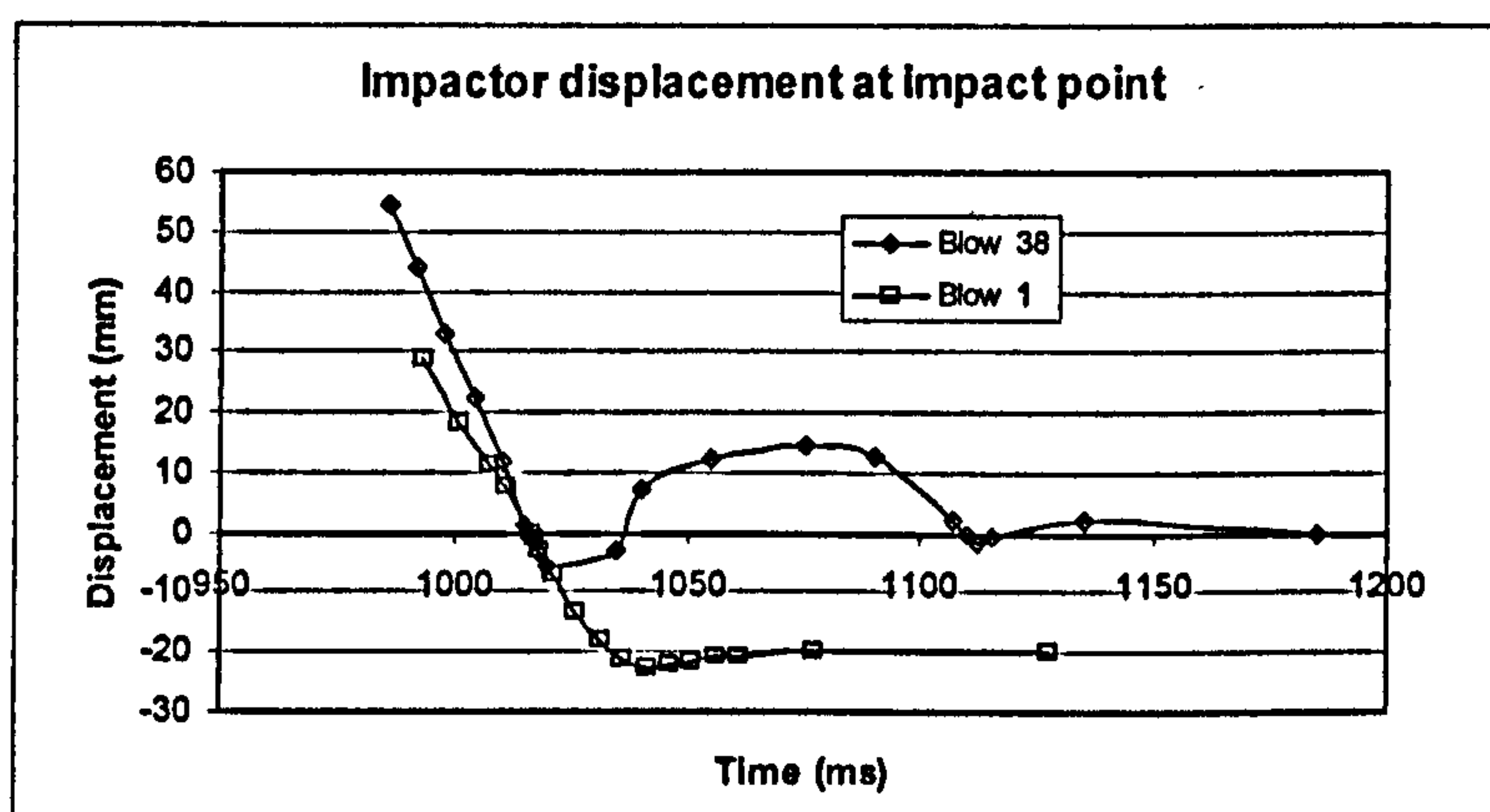
Figure 5.5 – Graphical representation of impactor displacement
