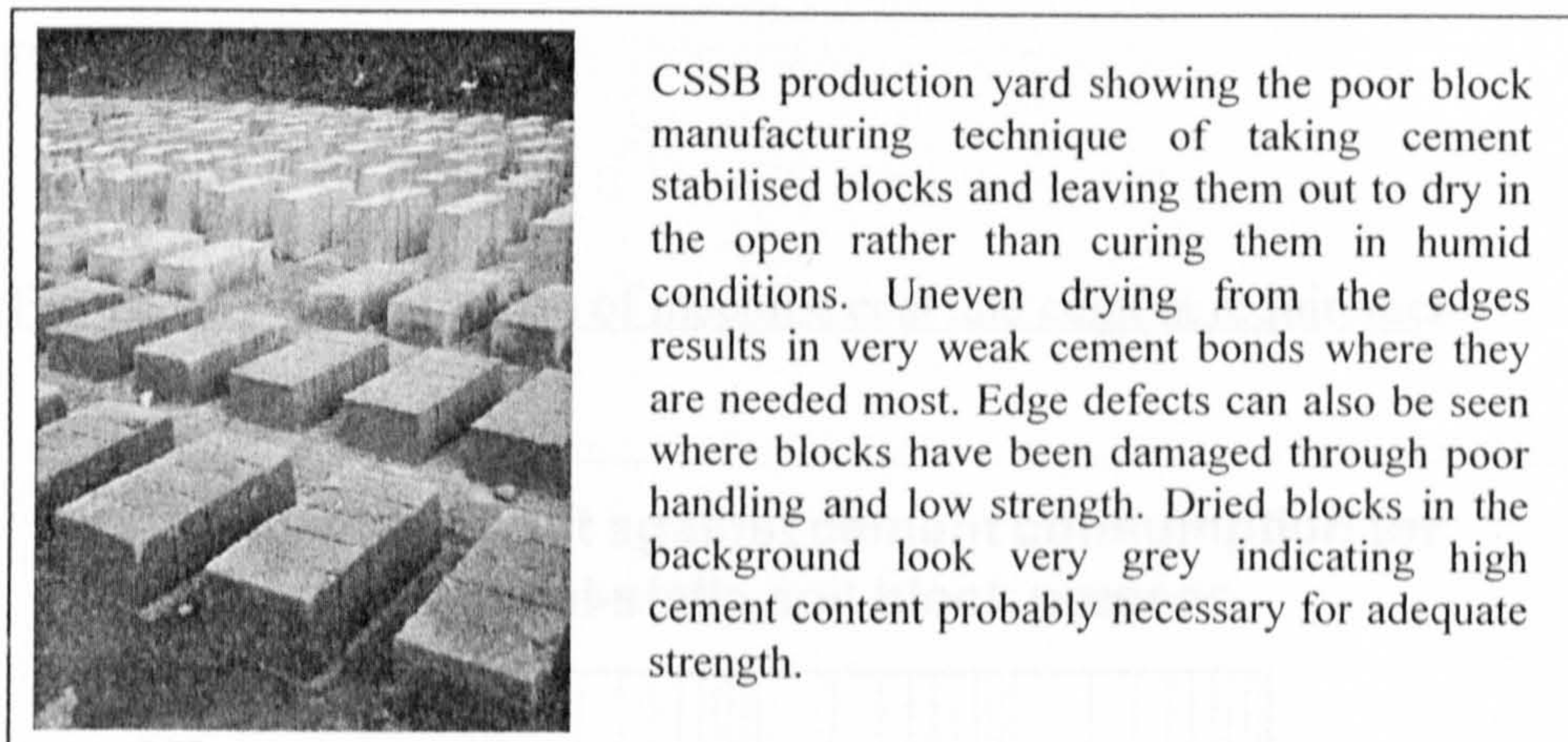
Figure 2.14 – CSSB production yard showing poor curing practice
