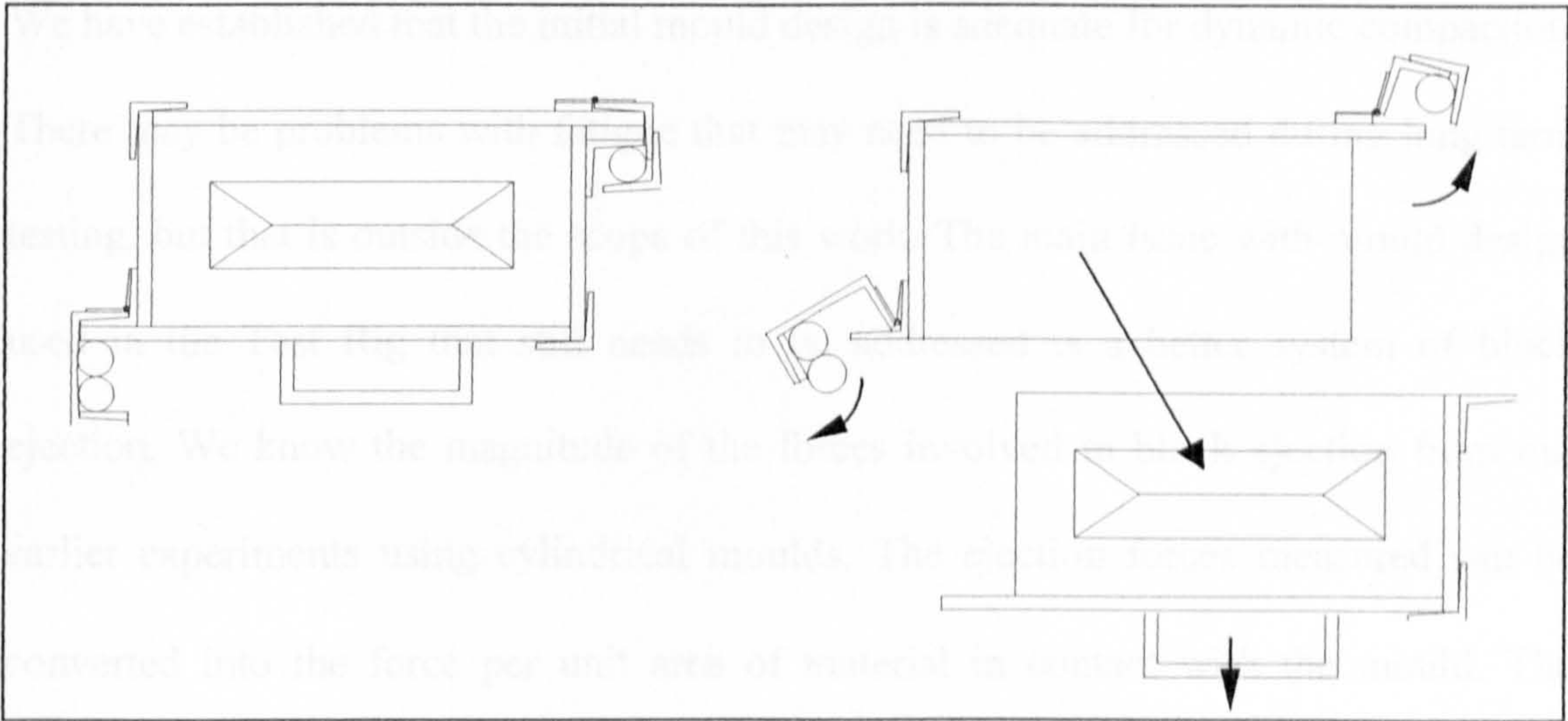
Figure 6.3 – Plan view of the two-part mould design
