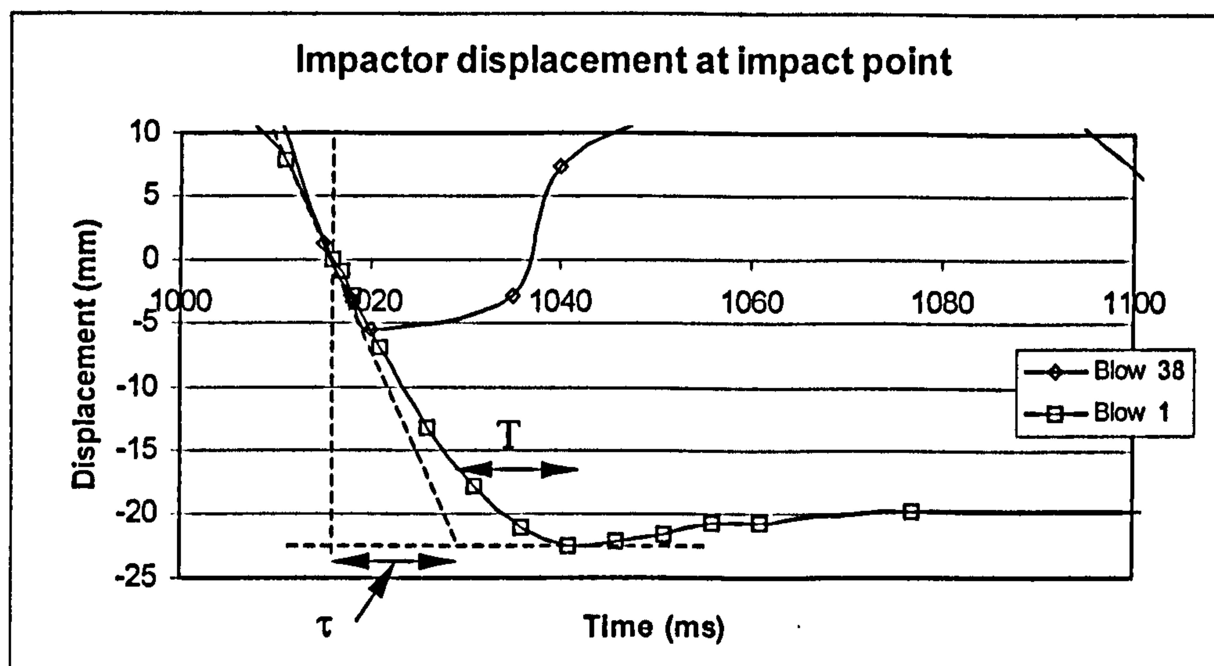
Figure 5.6 – Close up of impact point
