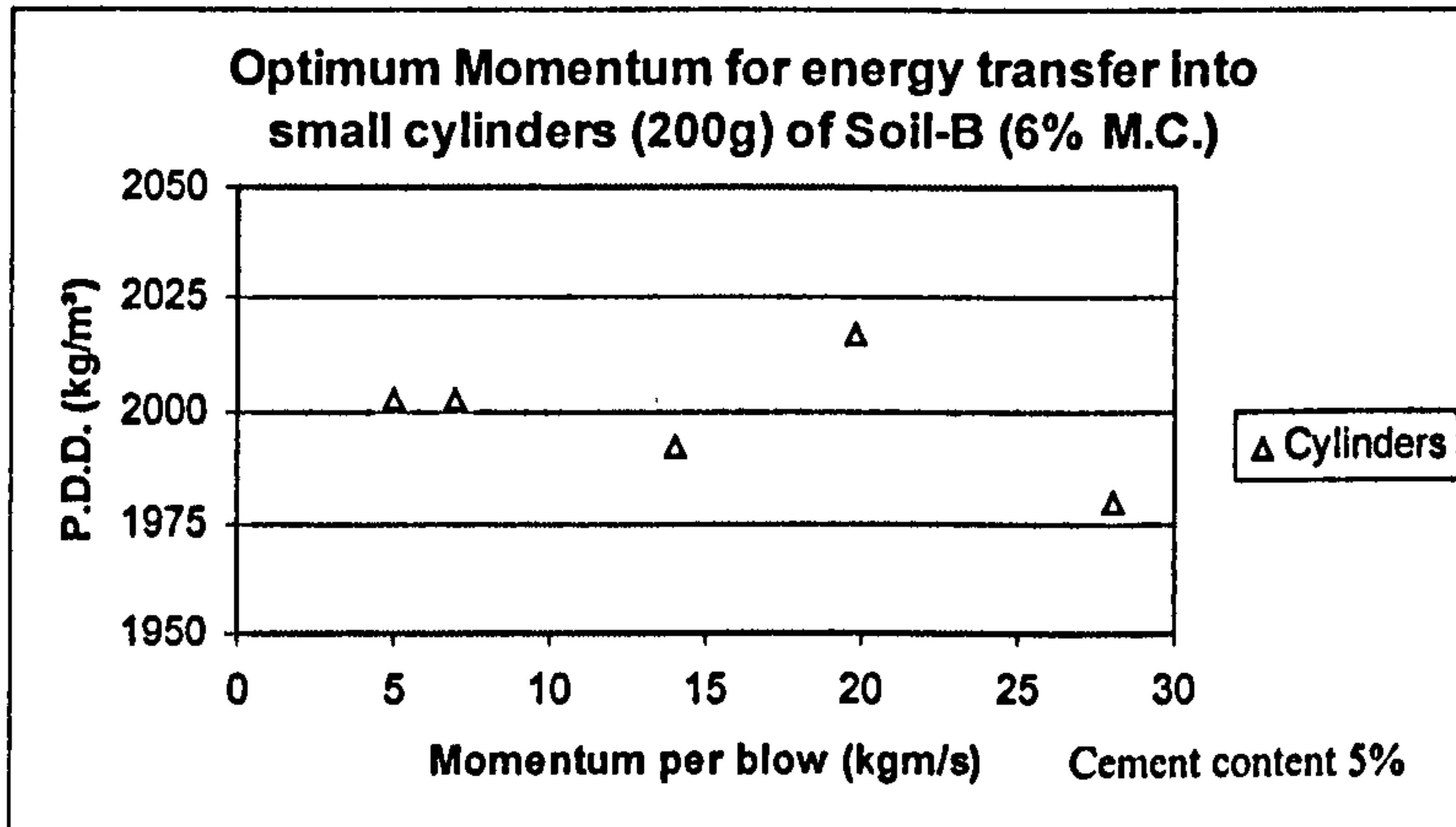
Figure 4.5 – Optimisation of momentum transfer for small cylinders
