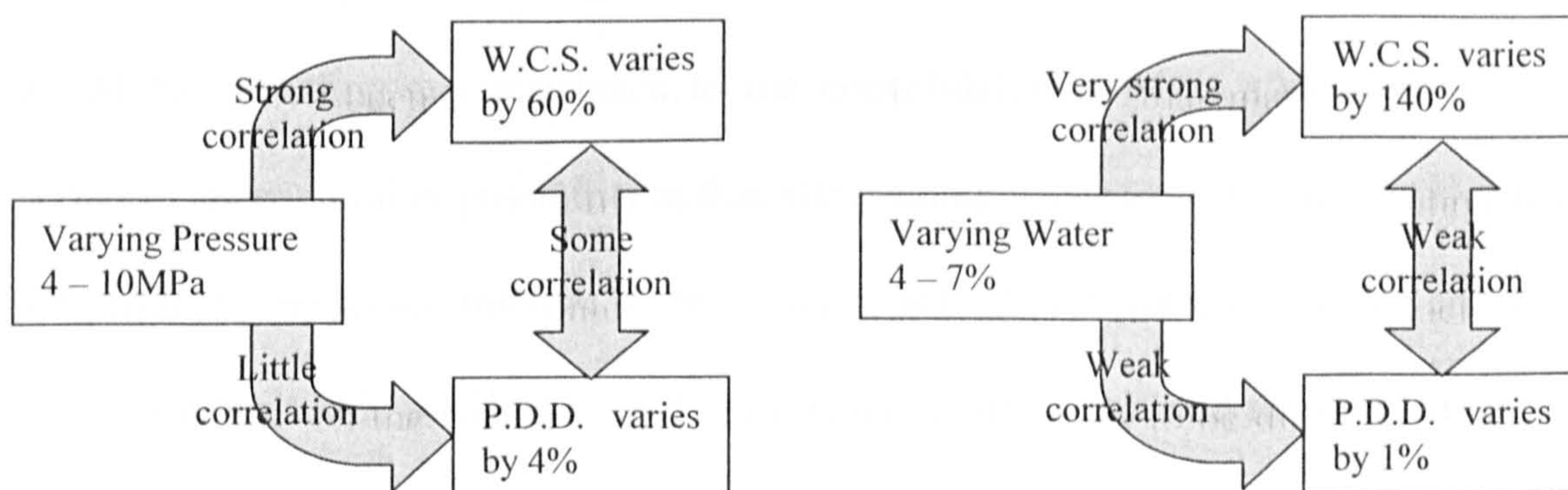
Figure 3.10 – Revised inter-relationships between pressure and water with outputs
