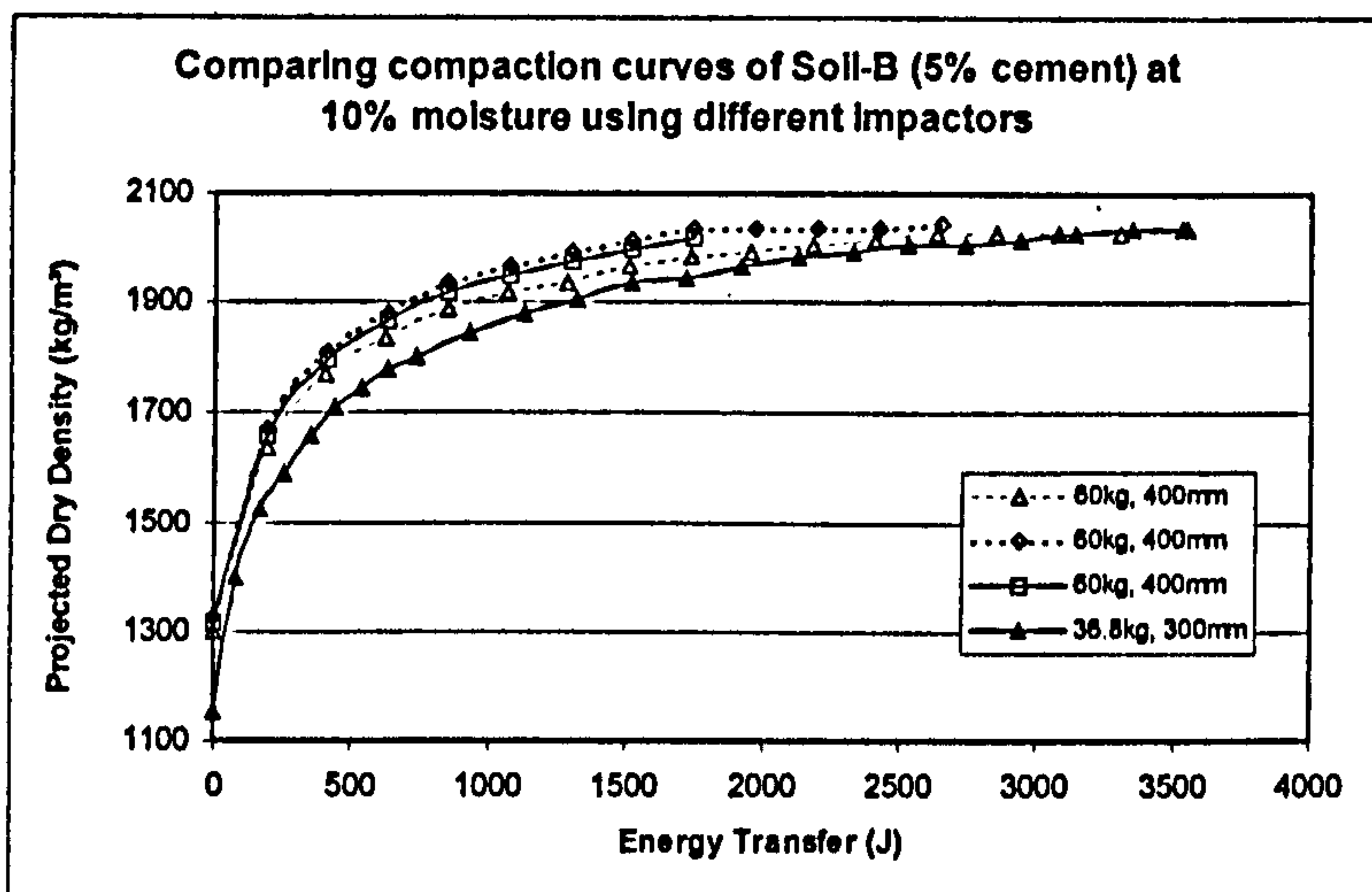
Figure 4.10b – Compaction curves for different impactors
