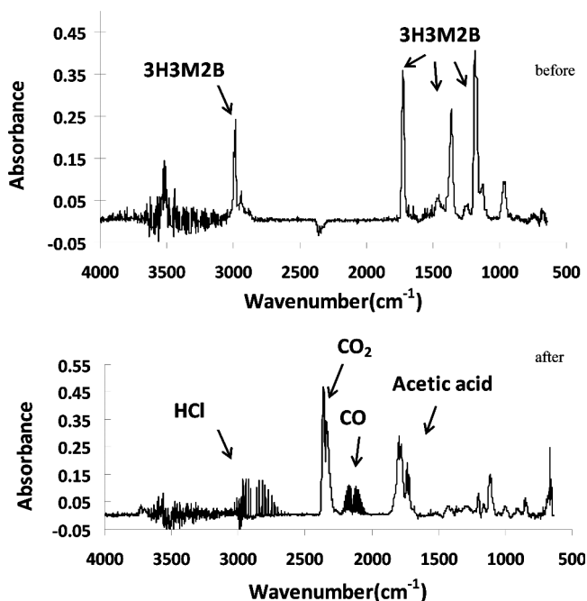
Figure 2. Example of infrared absorption spectra recorded in this work. The upper trace shows the infrared spectrum of the \text{Cl}_2/3\text{H3M2B} mixture in 720 Torr of synthetic air in the FTIR cell before irradiation, and the lower trace shows the spectrum 60 min after the start of irradiation.
