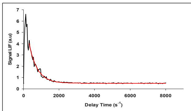
Figure 2. Kinetic decay as a function of the delay time between the pulses from the photolysis and probe lasers. P=40 Torr, T=297\text{K} , [\text{OH}]_0=5.7\times 10^{11} radicals \text{cm}^{-3} , buffer gas: He.
