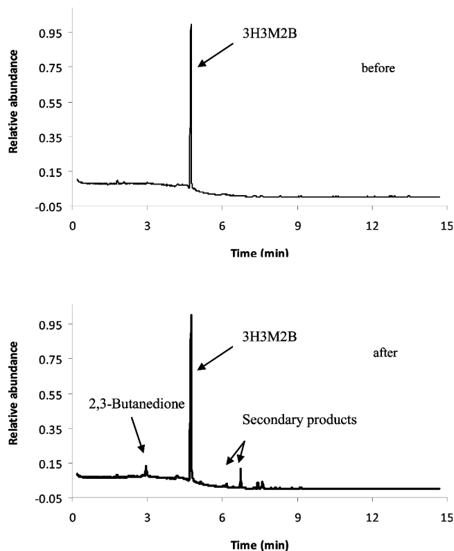
Figure 3. Gas chromatograms of samples from a \text{Cl}_2/3\text{H3M2B} mixture in 720 Torr of synthetic air in the Teflon bag before and 60 min after the start of irradiation.
