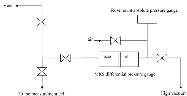
Figure 1. Static apparatus used for vapor pressure measurements.
