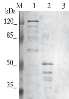
Figure 52: Western blot pET28-IgTeCe / Rosetta™ 2
