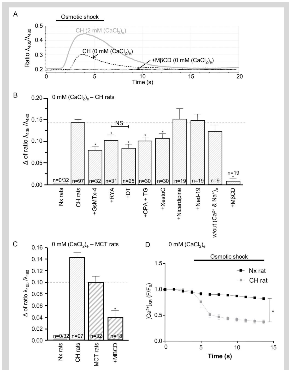
Figure 6. [\text{Ca}^{2+}]_i responses to osmotic shocks in PASMC from PH rats in absence of extracellular calcium. A. [\text{Ca}^{2+}]_i responses measured by indo-1 recorded in a CH rat PASMC following an osmotic shock of 225 mOsmol in absence of extracellular calcium + 1 mM EGTA and with methyl- \beta cyclodextrin (M \beta CD). B. and C. Summary of the amplitude of the calcium peak observed after an osmotic shock in PASMC from CH (B: N=3-10; C: N= 4-10). D. Curve representing the [\text{Ca}^{2+}]_{\text{SR}} as the ratio F/F 0 during time after an osmotic shock. [\text{Ca}^{2+}]_{\text{SR}} is measured by confocal microscope with the fluo-5N probe. The [\text{Ca}^{2+}]_{\text{SR}} decrease after an osmotic shock in CH-PASMC (n=6, N=3) but not in Nx-PASMC (n=6, N=3).
