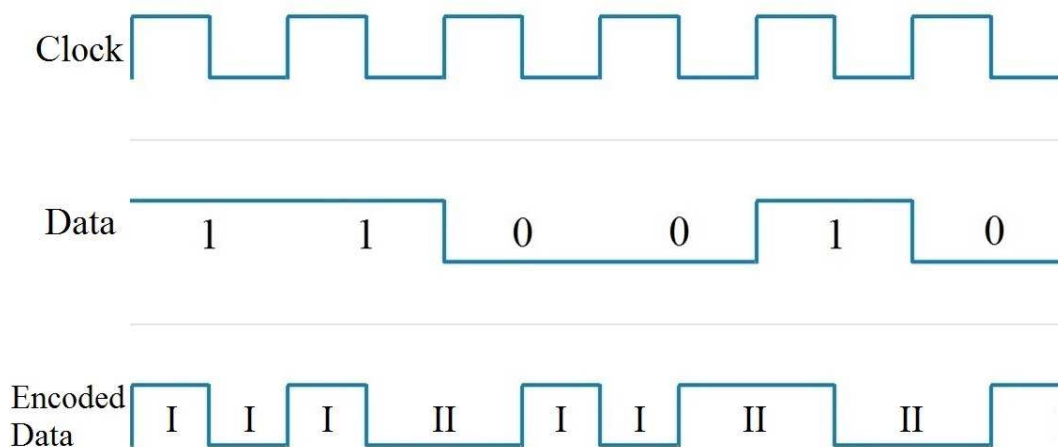
Figure 4.3: Manchester pulse widths.
