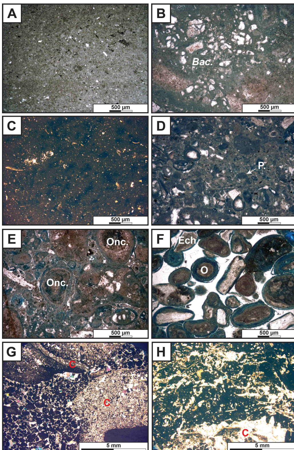
FIGURE 42 – Petrographic character of different textures from the Oxfordian limestone of the eastern part of the Paris Basin. A - Bioclastic mudstone (183.80 m). B - Bioclastic wackestone (bivalves and echinoderms) with cyanobacteria bacinella irregularis ( Bac. ) (235.65 m). C - Bivalves and echinoderms wackestone (329.10 m). D - Peloidal packstone (peloid = white arrow, 237.82 m). E - Oncoïd-bioclaster packstone with foraminifera ( Onc. ) (181.41 m). F - Micritic ooids ( O. ) grainstone with echinoderms ( Ech. ) (240.50 m). G - Coral boundstone ( C. ) with micritic ooid matrix (199.37 m). H - Encrusted corals ( C. ) with thrombolytic encrustation (357.75 m).
