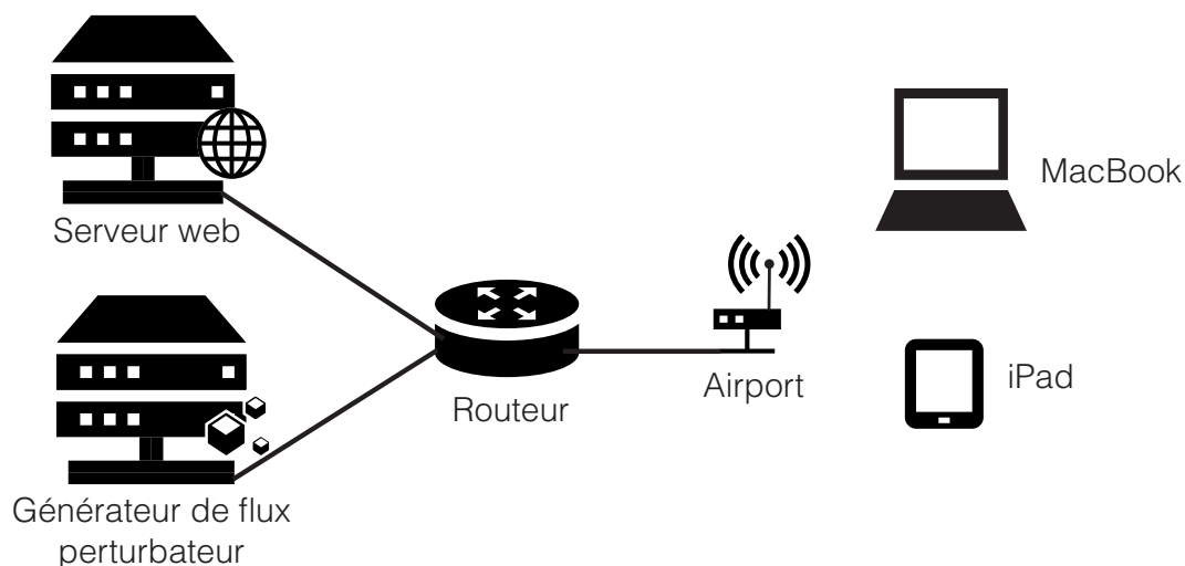
Figure 43: Plateforme de test HTTP Live Streaming
