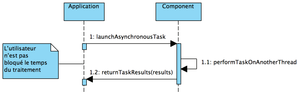
FIGURE 6.3 – Processus asynchrone
