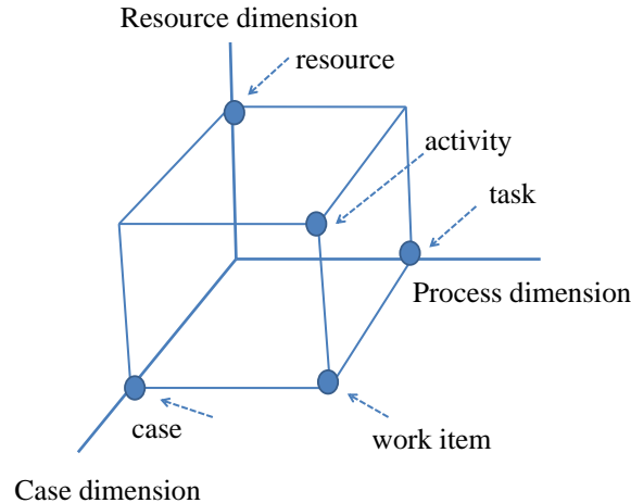
Figure 2.4: A three dimensional view of a workflow [van der Aalst 1998]
