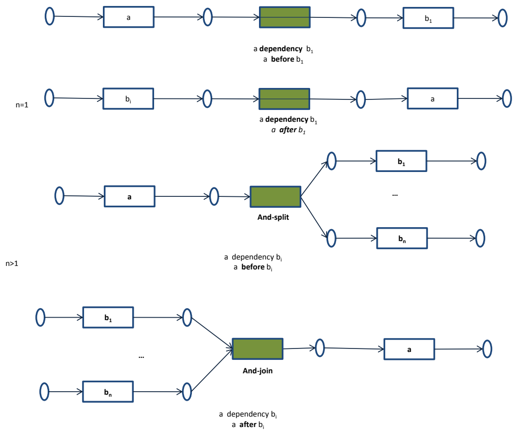
Figure 4.3: Representation of the set of semantic constraints SCD_{dep} in CPNs (Algorithm 3)
