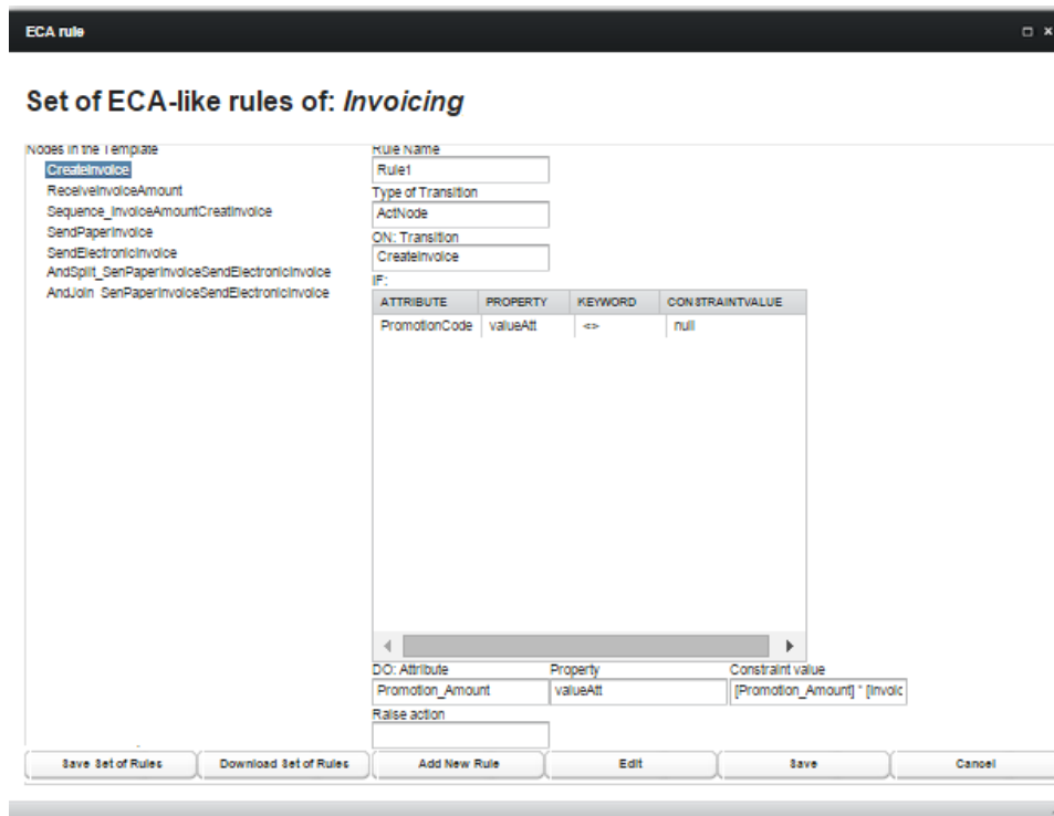
Figure 7.3: Interface used to browse and update ECA-like rules
