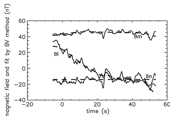
Figure 4. Three components of the magnetic field data measured by FGM and fit (dashed line) by the BV method in the magnetic field rotation region for Cluster C1 crossing of 15 April 2008.
