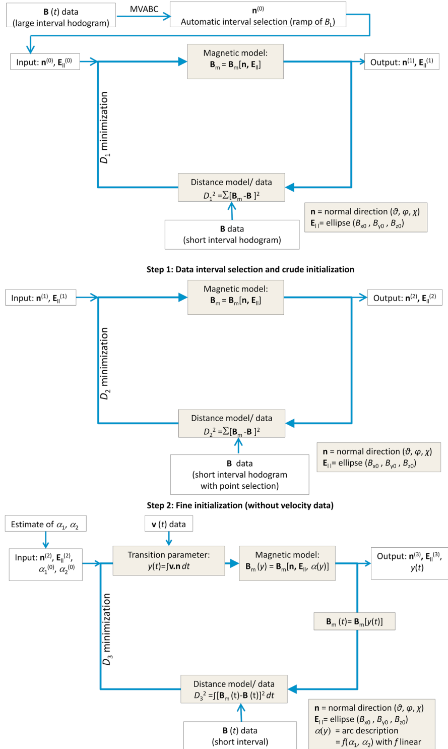
Figure B1. Algorithm used for the initialization of the BV method and the BV method itself. E || stands here for the elliptical form that is determined at each step (characterized by B x0 , B y0 , and B z0 ).
