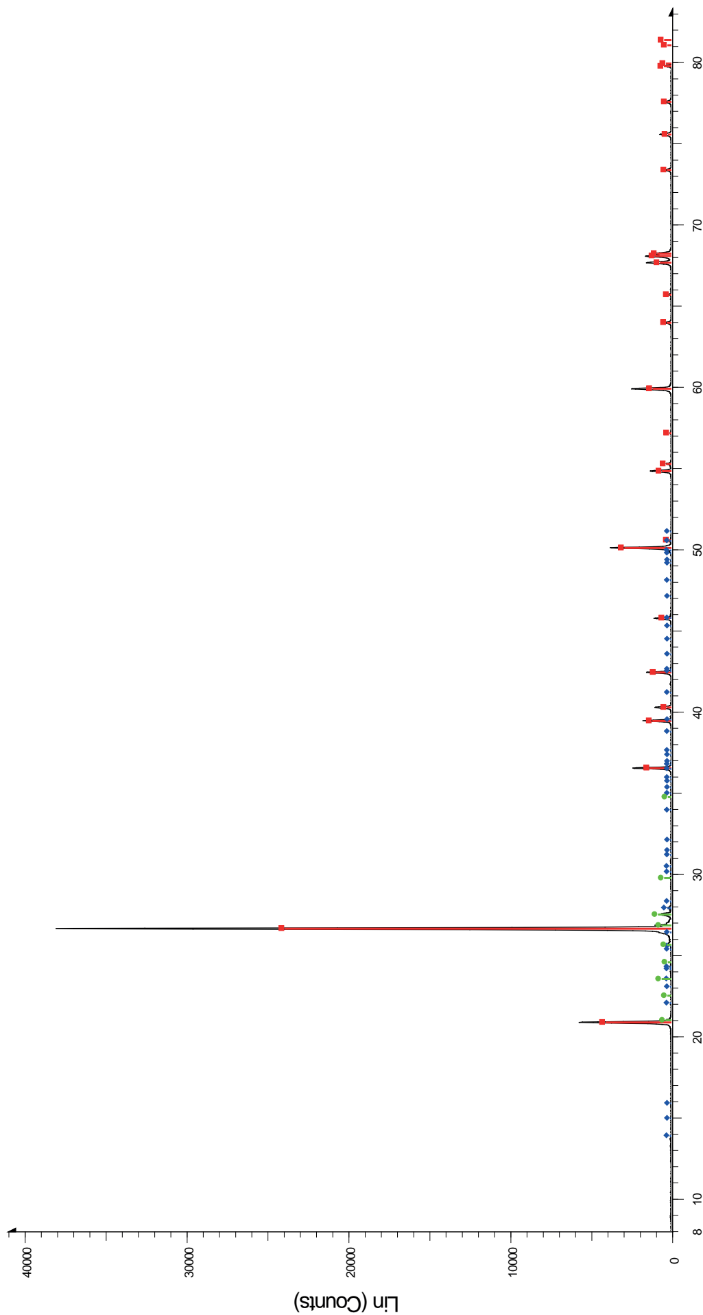
2-Theta - Scale
