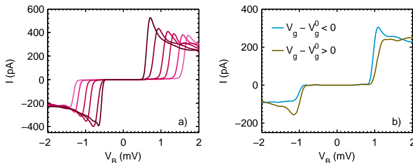
Figure 4.7: The peak shape is strongly dependent on the gate detuning from the charge degeneracy point. a) In device D, which has a rather symmetric tunnel coupling, the peak deforms symmetrically on the reversal of source-drain bias as the gate is detuned from the charge degeneracy point. b) In device C, which has a rather strong tunnel coupling asymmetry, the peak deforms asymmetrically upon the reversal of the bias.
