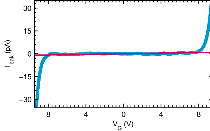
Figure 1.5: The quality of the gate insulation layer can be visualized by gate leakage current as function of the applied voltage (blue circles). The red line corresponds to a 10\text{ T}\Omega resistance. This shows that the ALD process allows us to create thin and high quality gate insulation layers with a high break-through voltage (8 V) and negligible gate leakage.
