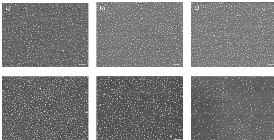
Figure 1.14: Scanning electron microscope images of gold nanoparticles (12 nm) deposited using a self assembling monolayer created with varying silanization parameters. The oxygen plasma time (a, b, c) (APTES dose = 4 sccm) plasma time has little significant effect on the particle density. However with increasing APTES dose (d, e, f) (plasma time = 30 s) their appears to be a little decrease in particle density. The scale bars represent 100 nm.
