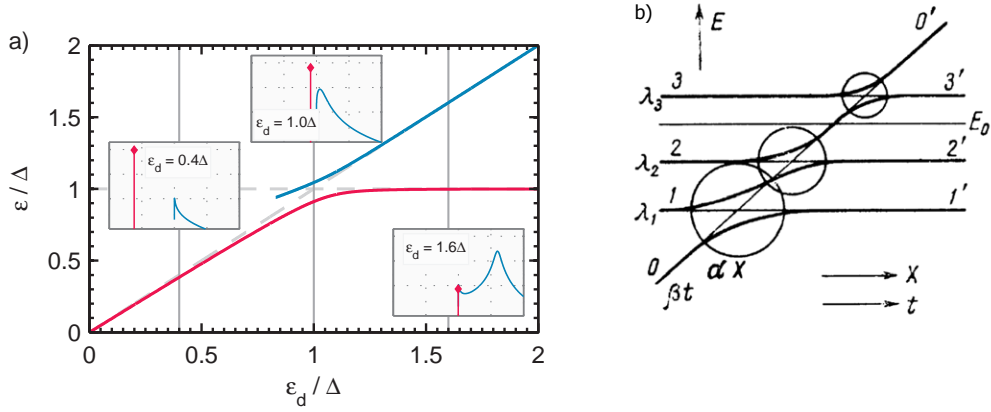
Figure 5.6: a) Spectral properties single level coupled to a superconductor ( \gamma = 0.04\Delta , \Delta = 265 \mu\text{eV} ). For \epsilon_d < \Delta there only exists one discrete solution |A\rangle (magenta), while above \epsilon_d \approx \Delta there exists a second quasi-particle state |qp\rangle (blue) with \epsilon_{qp} \approx \epsilon_d . Insets display the spectral density and weight of the states at \epsilon_d/\Delta = 0.4, 1.0, 1.6 , as function of \epsilon on a log scale. b) Avoided crossings of a single discrete level with multiple close lying discrete states used by Demkov and Osherov [26] to explain the avoided crossing of a single discrete with a semi-continuum density of states ( \delta \rightarrow 0 ).
