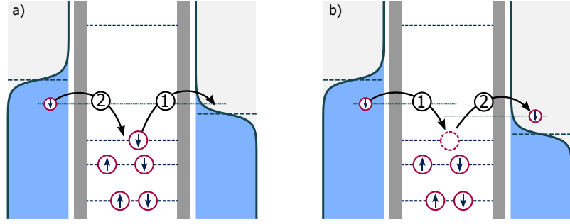
Figure 3.11: Higher order tunnel processes are leading when sequential tunneling is blocked by the charging energy. In second order processes, known as cotunneling, electrons can tunnel to and from the quantum dot, even if energy conservation is temporarily violated, provided that a second event 'restores' the quantum dot state. Cotunneling can be both elastic (a) or inelastic (b).
