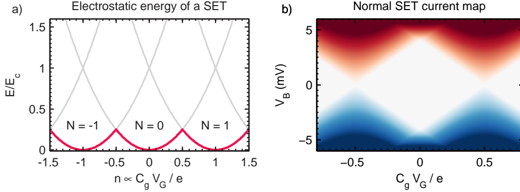
Figure 3.2: a) The electrostatic energy of the island depends on the number of additional charges on the island. For each value of the additional charge, the electrostatic energy is a parabolic function of the gate induced charge. The red curve denotes the island ground state. b) The current map, i.e. I(V_B, V_G) , of a single electron transistor shows diamond shaped areas in which the current is zero. ( T = 100 mK, E_C = 2.0 meV)
