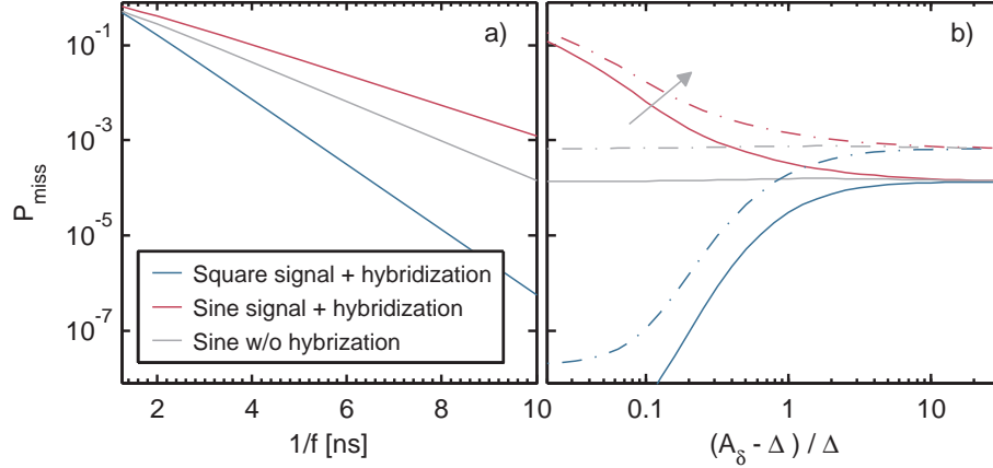
Figure 5.4: Probability of missed tunnel events in a single level turnstile as function of (a) signal frequency ( A_\delta = 1.1\Delta ) and (b) amplitude ( f = 100, 120 MHz). Calculated rates are obtained with the 1) first order model (grey curves) and 2) the hybridized model (blue and red curves). The arrow in (b) points to increasing frequency. ( \Delta = 265\mu\text{eV} , \gamma = 0.03\Delta )
