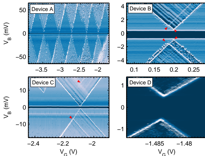
Figure 4.3: Color maps of the differential conductance measurement in four devices (A, B, C, D) at base temperature ( T \approx 80 mK). Coulomb diamonds measured in most devices (denoted by an asterisk in table 4.1), e.g. (b-d), extend beyond the scope of the measurements. Additional slanted lines (indicated by red arrows) outside the Coulomb diamonds observed in some devices indicate single quantum dot levels (excitations) with an energy spacing that varies between 2 and 10 meV.
