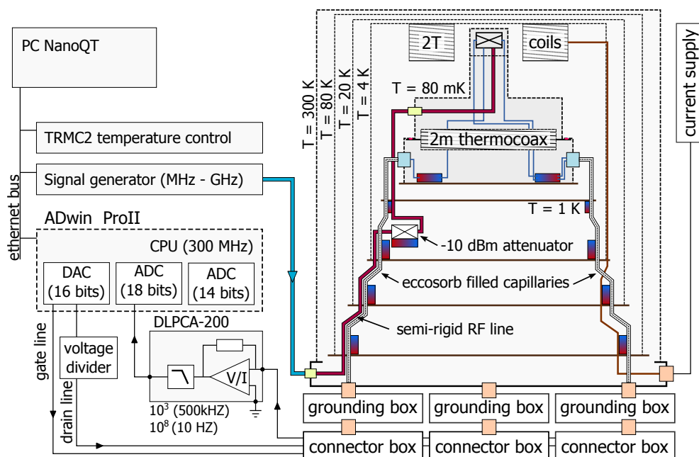
Figure 2.4: A schematic of our measurement setup including the wires in the cryostat.
