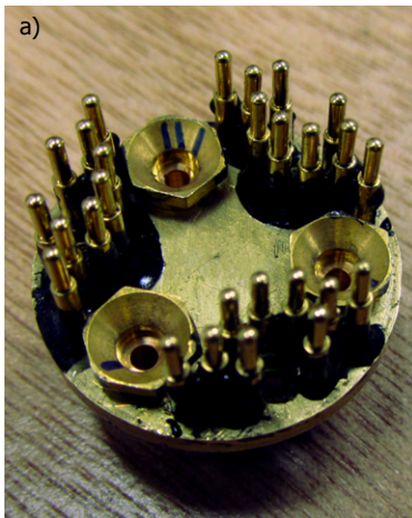
Figure 2.6: The sample stage (a) is made of a thick brass disk on which 27 spring-pin connectors and 3 SMP receptacles are mounted. The three SMP connectors ensure a good alignment of the 27 spring-pins with respect to the sample carrier (b).
