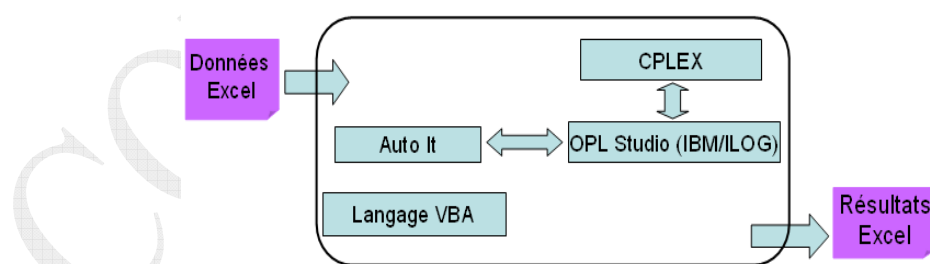
Figure V-2: Architecture technique de l'application
