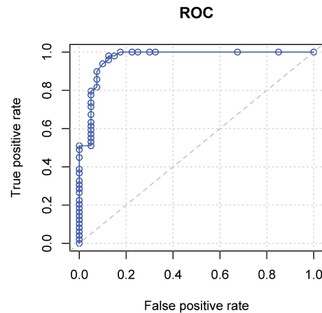
Figure 4.3: ROC curve for the logistic regression that predicts whether an item is a trend or not.
