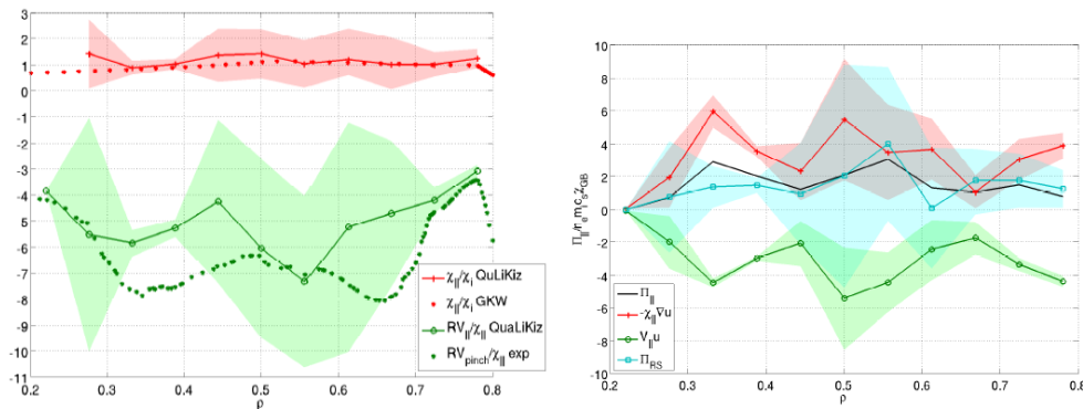
Figure 5.11: Left panel: Prandtl number (red crosses) and pinch number (green circles) calculated by a 3-point method. Right panel: Details of the different contributions to the parallel momentum flux. From [42].
