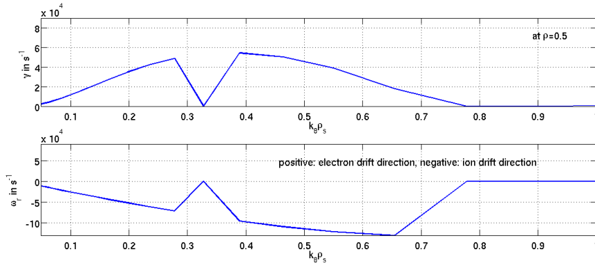
Figure 3.19: JET pulse 79698 at 13 s without collisions. At a given radius, here \rho = 0.5 , the spectrum of the growth rate \gamma is plotted as a function of k_{\theta}\rho_s , top panel. Bottom panel: the spectrum of the frequency is illustrated.
