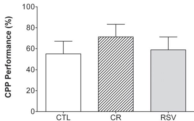
Figure 3. Effects of CR and RSV treatments on percentage of reversal in a conditioned placed preference (CPP) task. Data of control (CTL, n=8 ), caloric restricted (CR, n=8 ) or resveratrol supplemented (RSV, n=9 ) mouse lemurs after 18 months of dietary interventions are reported. Values are mean \pm SEM. doi:10.1371/journal.pone.0016581.g003
