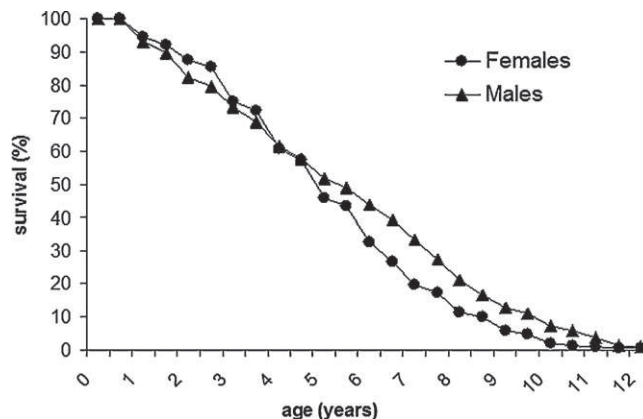
Fig. 1. Survival curve from 643 mouse lemurs (361 females and 282 males) of the Brunoy colony.
