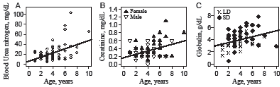
Figure 4. Statistical analysis was performed with Pearson correlation. A: Simple linear regression between blood urea nitrogen levels and age (n=77, r=0.46 , p<0.001 ). B: Simple linear regression between creatinine levels and age (n=75, r=0.28 , p<0.01 ). C: Simple linear regression between total blood globulin concentration and age (n=73, r=0.20 , p<0.05 ), LD: long-day season; SD: short-day season.
