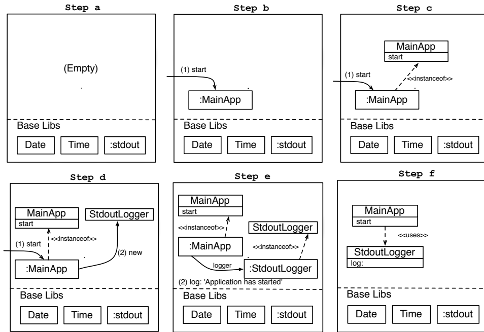
Figure 8.4: The nurtured runtime at different steps of tailoring.
