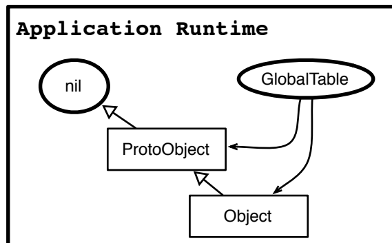
Figure 6.5: Step 3: Create classes. Classes are created by the class builder and installed inside the global table.
