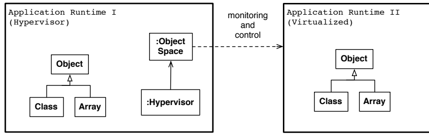
Figure 4.2: Espell Coexistence. The hypervisor controls the virtualized runtime through an object space.
