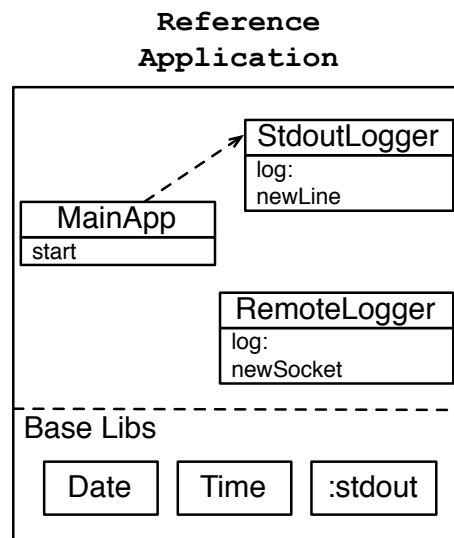
Figure 8.3: Reference runtime with all code units.
