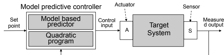
Figure 3.4 – The Model predictive control process [102]
