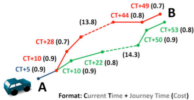
Figure 6.2 – A trajectory selection mechanism based predictive analysis
