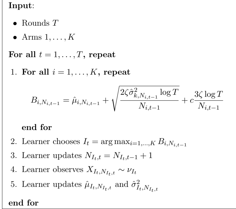
Figure 3.2: UCB-V
