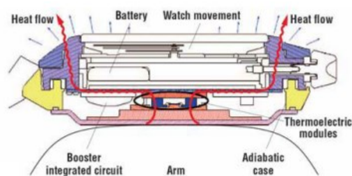
Figure 1-16 Montre Seiko [KNHY99].
