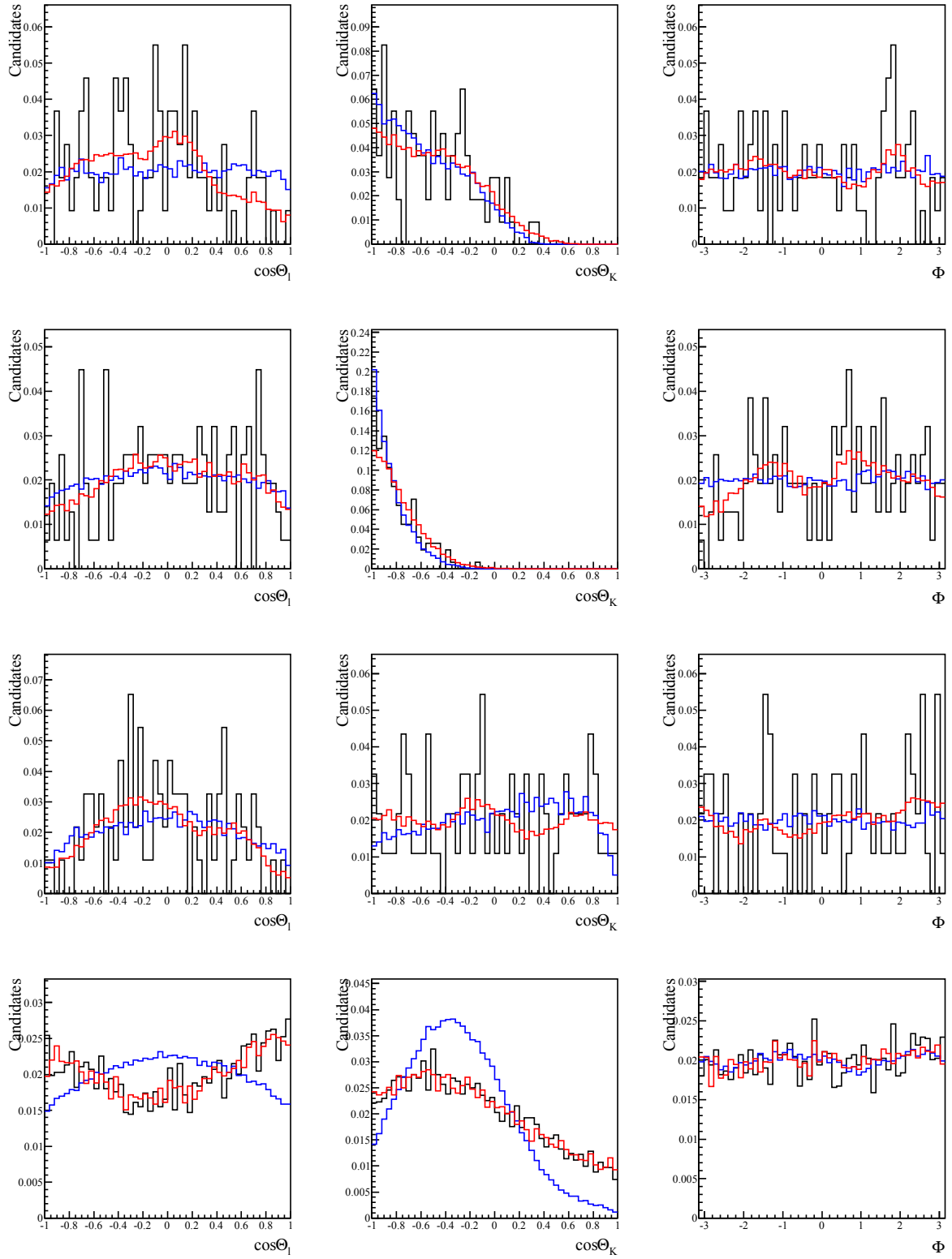
Figure D.3: The decay angles (left) \cos\theta_l , (middle) \cos\theta_k , and (right) \phi for (black) b \rightarrow X\mu^+\mu^- decays, (blue) b \rightarrow J/\psi X decays, and (red) from the kernel method described in the text. The three peaking backgrounds studied are (first row) \Lambda_b^0 \rightarrow pK\mu^+\mu^- , (second row) B_s^0 \rightarrow \phi\mu^+\mu^- , (third row) B^0 \rightarrow \pi^+\pi^-\mu^+\mu^- and (fourth row) B^0 \rightarrow K^+\pi^-\mu^+\mu^- swaps.
