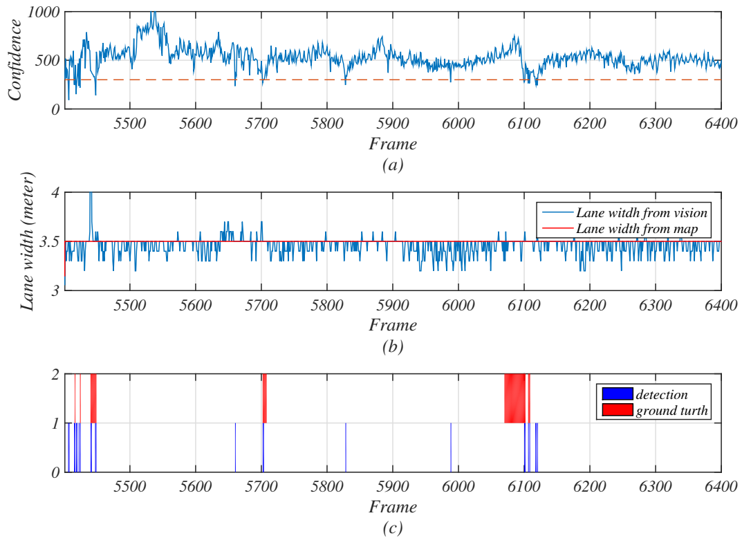
Figure 5.21: Lane detection error of scenario B. (a) Lane detection confidence, blue curve is the confidence curve, red curve is the threshold; (b) lane width curve; (c) detected error.
