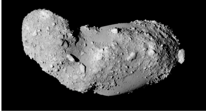
Fig. 1: Image of the small S-type NEO Itokawa (about 500 m) observed by the Japanese spacecraft Hayabusa in 2005.
