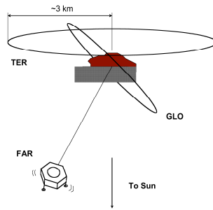
Fig. 2: Orbit configuration for the first mission phases.
