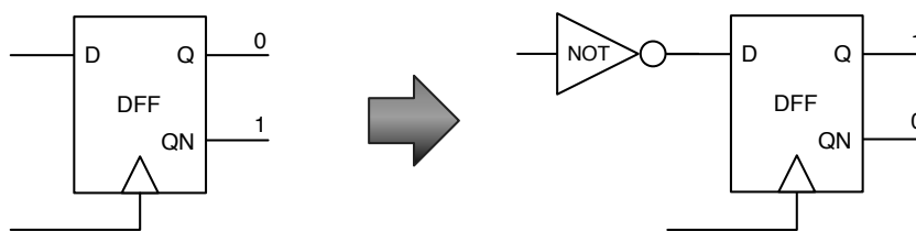
Figure 4.5: Optimisation through state reversal
