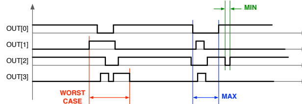
Figure 3.9: Output SET evaluation
