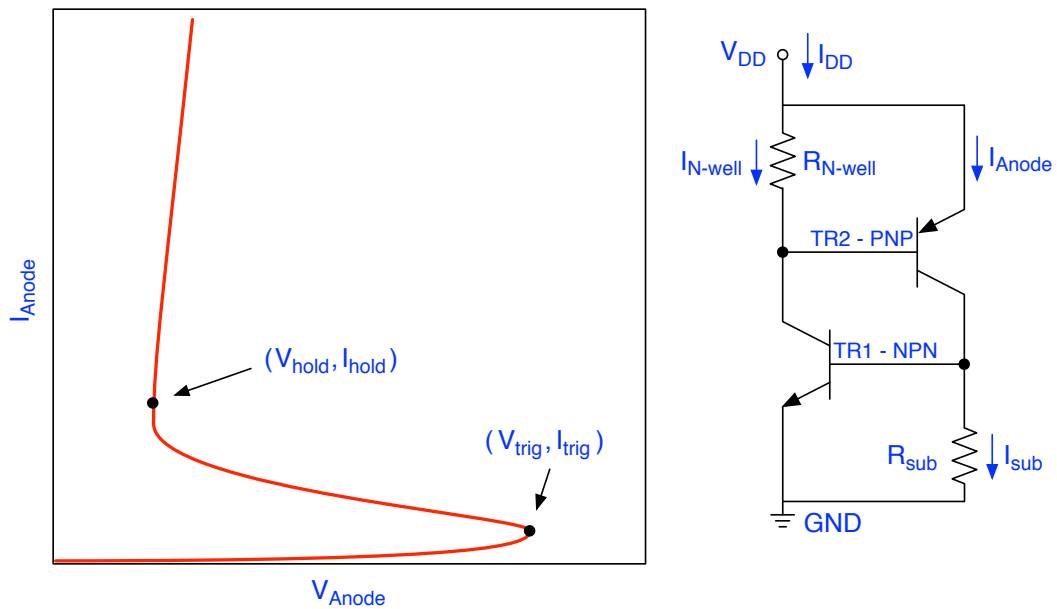
Figure 1.30: I-V Characteristic of a Latchup and Thyristor Formed by PNPJ Junction.
