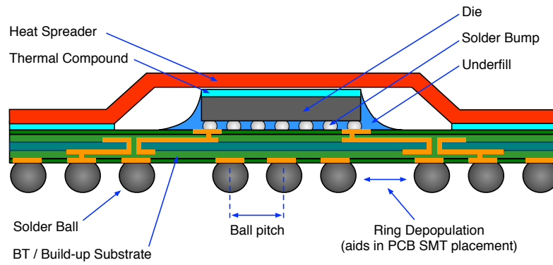
Figure 1.15: Cross Section of Typical Flip-Chip Package.
