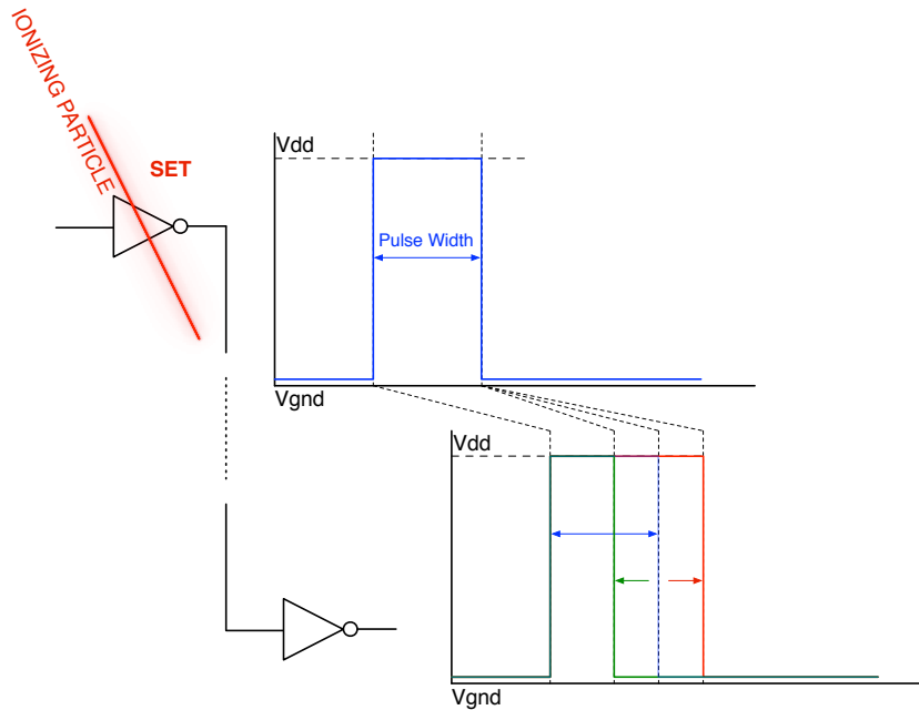
Figure 2.6: Propagation Induced Pulse Broadening - PIPB
