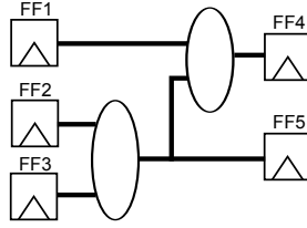
Figure A.7: Shared Timing Paths
