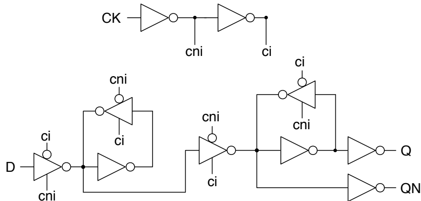
Figure 4.1: Flip-Flop Structure
