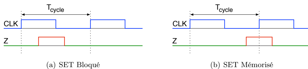
Figure 1.8: Blocage Temporel des SETs
