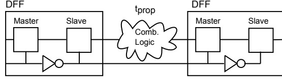
Figure A.1: Master-Slave Flip-Flops
