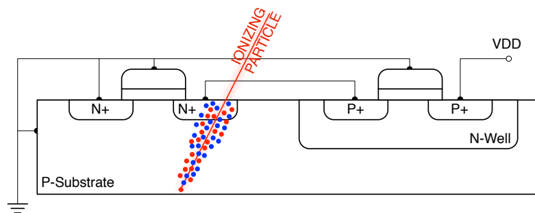
Figure 1.26: Single Event Transient production: interaction of an ionizing particle with an inverter.
