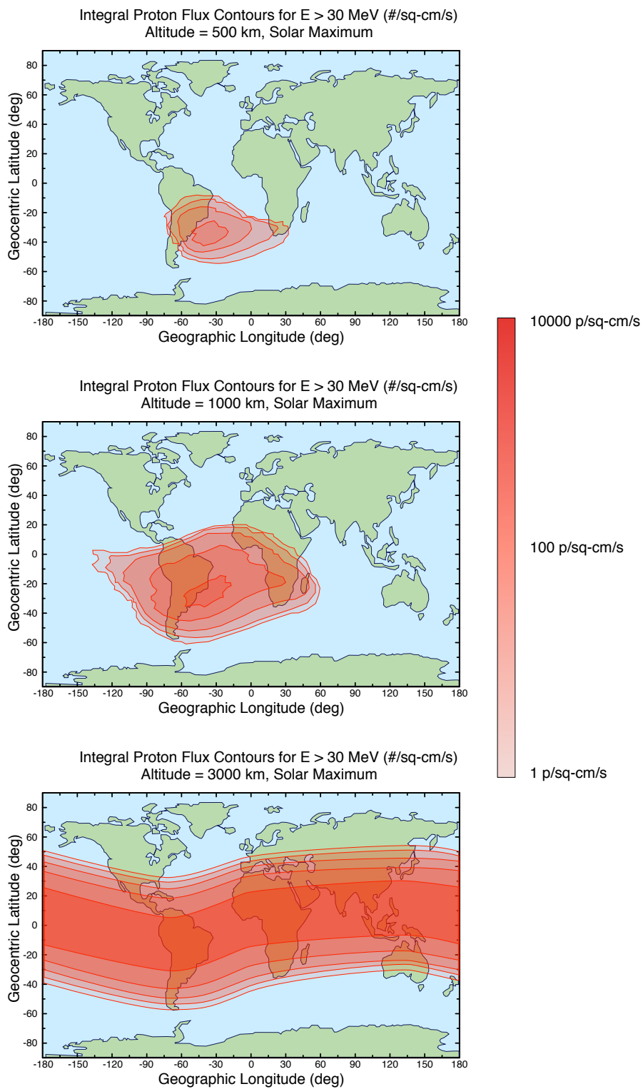
Figure 1.6: Integral proton flux contours as a function of latitude and longitude at 500 km, 1000 km, and 3000 km.
