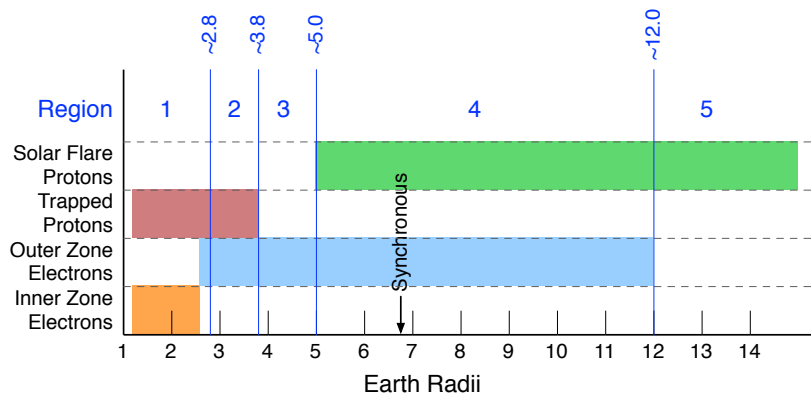
Figure 1.4: Boundaries of the domains for solar flare and trapped protons and outer and inner zone electrons [Faruk 2012].
