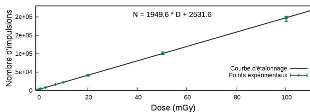
(e) Cobalt
