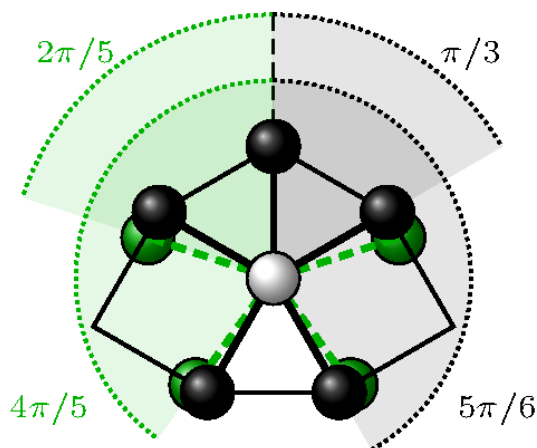
Figure 3.20.: Schematic view of the neighborhood of a particle in the snub square tiling. Going clockwise from the top, each vertex is formed by the following sequence of surrounding polygons: \triangle - \square - \triangle - \square - \triangle . The respective bond angles (indicated by dotted black lines) are close to the ones of a pentagonal arrangement (indicated by the green particles and the dotted green lines).
