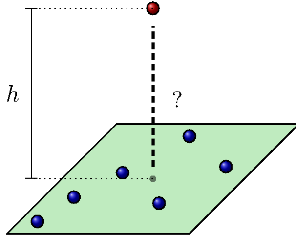
Figure 3.5.: Schematic view of the Wigner monolayer (blue spheres) when vertically displacing a single charge (denoted "tagged" charge; red sphere) by a distance h . This process is energetically unfavorable, leading to a positive energy of the defect. Charges in the layer rearrange to compensate for the displacement of the tagged charge.
