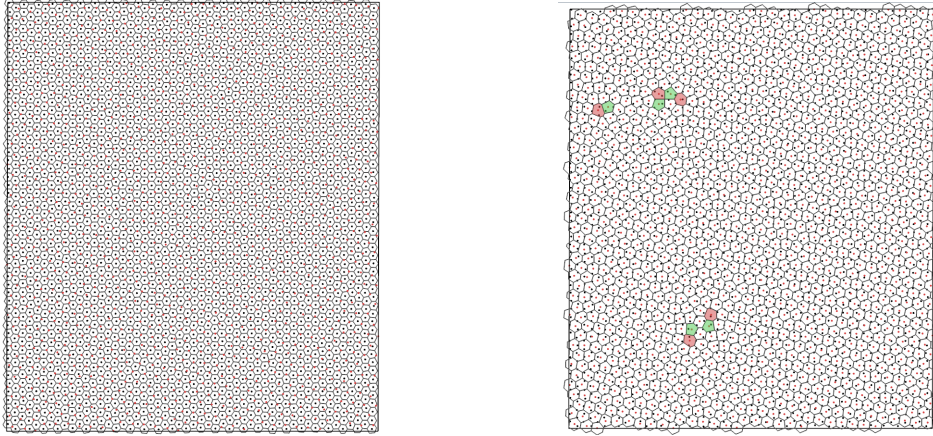
Figure 3.33.: Snapshots of MC simulations for \eta = 0.78 and A = 0.623 (where we predict structure V_x ). Particles in layer 1 and 2 are colored black and red, respectively. Voronoi polygons are colored according to their number of sides: three sides (black), four (yellow), five (green), six (white), seven (red), eight (blue). Left panel: Voronoi construction for layer 1. Right panel: Voronoi construction for layer 2. Note that both layers exhibit good hexagonal order.
