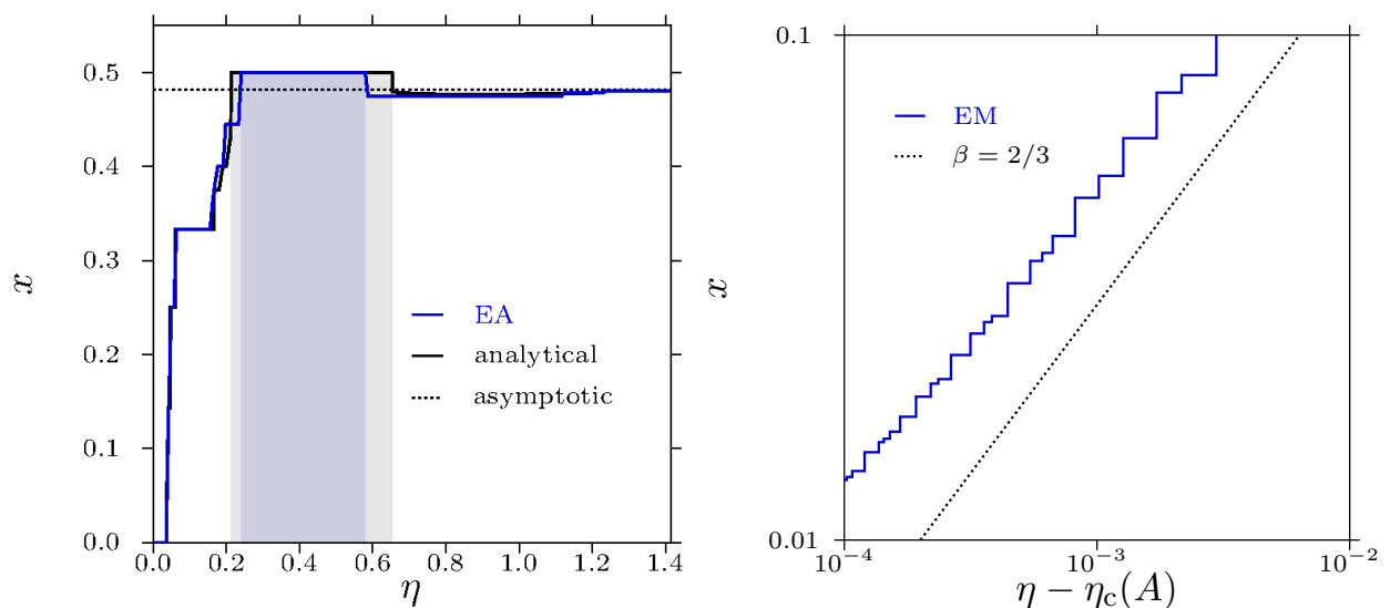
Figure 3.26.: x(\eta) for A = 0.93 . Left panel: curve over the entire considered range of \eta . EA results in blue, analytical results in black. In the region of stability of structure I_x (where x < 1/3 ), a discrete set of compatible x -values (see N_{\text{out}} in Equation 3.19) is preferred, evidenced by a staircase-like form of the curve; regions of constant x are very thin for A this close to unity. However, non-compatible values are also possible in the EA approach. Shaded areas indicate overcharging, i.e., where x > x_{\text{asy}} . Right panel: double-logarithmic plot of x(\eta - \eta_c) . The dotted black line is a guide to the eye, indicating a critical exponent \beta = 2/3 (see Equation 3.63).
