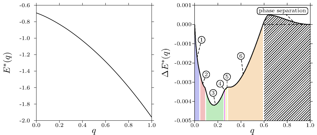
Figure 3.3.: Left panel: ground state energy E^*(q)/N of the equimolar binary mixture Wigner crystal as a function of q . The energy per particle is given in units of \sqrt{\rho}Q^2 . The curve exhibits no identifiable features to the naked eye. Both limiting cases q \rightarrow 1 and q \rightarrow 0 yield well-known results. Right panel: after subtraction of the phase separation reference energy E_{\text{ref}}^*(q) , a variety of features emerges in \Delta E^*(q)/N , indicating the occurrence of transitions between different structures (labelled 1 through 6 and indicated by colored regions). Note that relevant energy differences are by about three orders of magnitude smaller than the total energy per particle. For Q \geq 0.6 , we obtain energies larger than E_{\text{ref}}(q) , indicating the occurrence of phase separation (hatched region).
