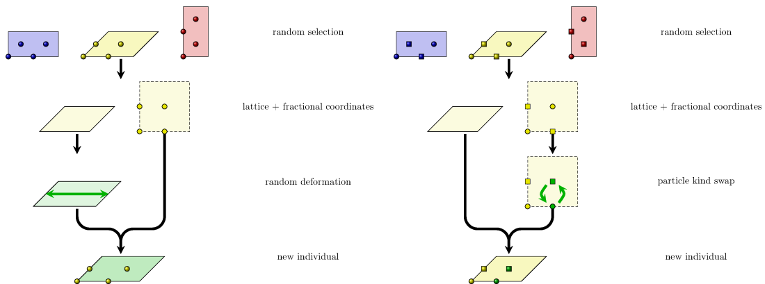
Figure 2.9.: Left panel: illustration of the strain mutation operator. A candidate is picked at random and its lattice vectors are randomly deformed. Right panel: illustration of the swap mutation operator. A candidate is picked at random and the species of two particles is interchanged.
