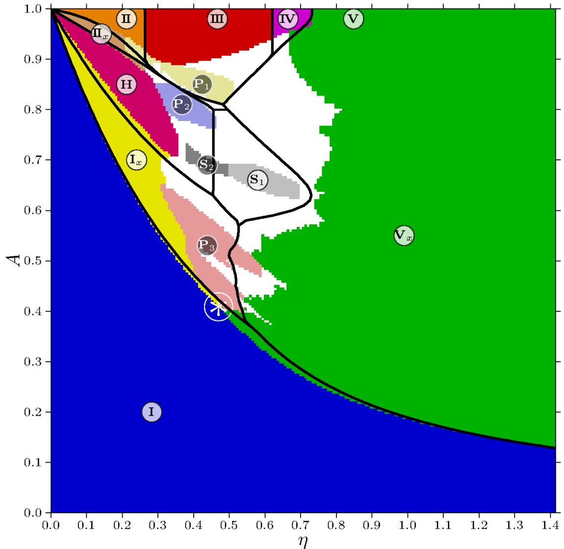
Figure 3.22.: Full phase diagram showing all structures identified in the preceding subsections (as labeled). Structures that could be treated within the analytical approach have light labels. Black lines mark the respective regions of stability determined with the analytical approach. Structures with dark labels are too complicated to be treated within the analytical approach. White regions indicate structures with more complicated geometric features, some of which may be characterized by specific color combinations in the \Psi RGB-phase diagrams (see Figure 3.25).
