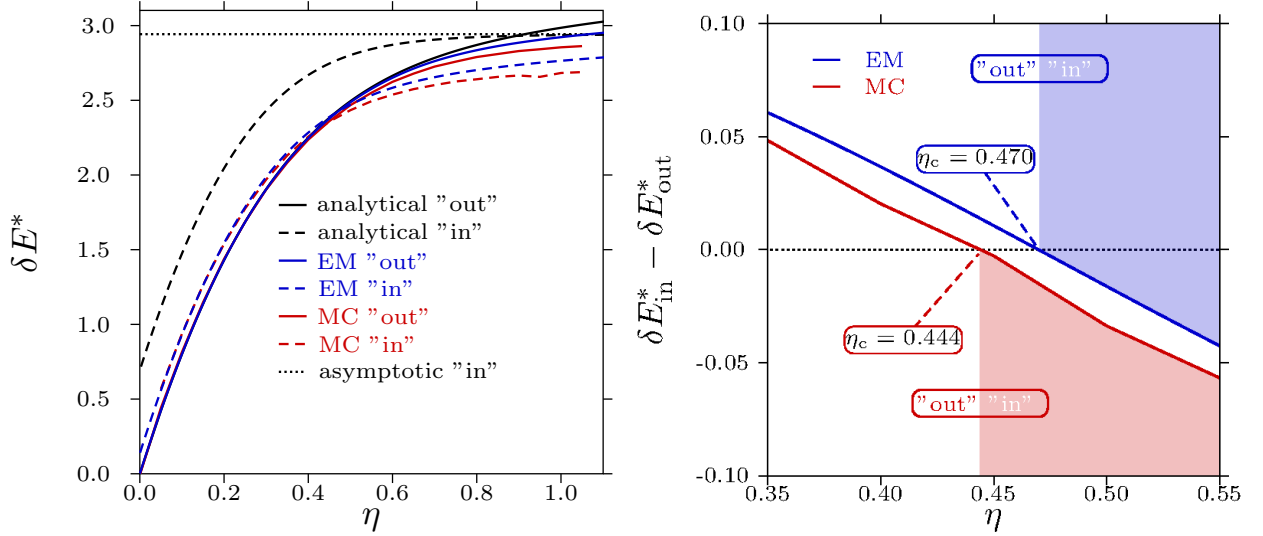
Figure 3.8.: Defect energies obtained with the three approaches: analytical calculations (black), energy minimization (blue), and MC simulations (red). Left panel: defect energies \delta E^*(\eta) obtained for the "out"-branch (solid lines) and the "in"-branch (dashed lines). The asymptotic limit for the "in"-branch E_{in}^*(\eta \rightarrow \infty) is indicated by a dotted black line. Right panel: energy difference between "out"- and "in"-branches, \delta E_{in}^* - \delta E_{out}^* , close to the transition. The \eta -range where the "in"-branch is favorable differs slightly between the EM and MC approaches (indicated by colored regions).
