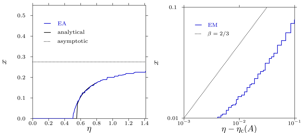
Figure 3.27.: x(\eta) for A = 0.38 . Left panel: curve over the entire considered range of \eta (compare Figure 3.26). EA results in blue, analytical results in black. As \eta_c is rather large, the two layers are not strongly correlated, leading to a smooth curve x(\eta) . The asymptotic value x_{\text{asy}} is indicated by a dotted line. Note the visible difference in \eta_c between the two approaches; this difference is due to deformations, which are rather strongly pronounced in structure V_x this close to the tricritical point (see also Figure 3.22). Right panel: double-logarithmic plot of x(\eta - \eta_c) . The dotted black line is a guide to the eye, indicating a critical exponent \beta = 2/3 .
