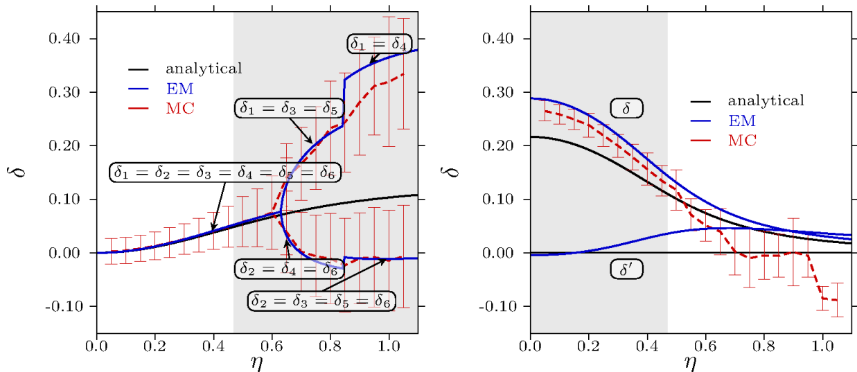
Figure 3.9.: Deformations of the lattice surrounding the tagged charge (displacement of the six nearest neighbors from their equilibrium positions at \eta = 0 ) obtained using the following three approaches: analytical calculations (black), EM (blue), and MC simulations (red). In the MC approach, a Gaussian fit is used to determine the peak positions in g(r) and thus the deformations [151, 156]. Error bars indicate the width of the peaks. Left panel: "out"-branch, where we measure displacement of the six particles in the first ring. In the stable region \eta \lesssim 0.47 , the ring of nearest neighbors contracts isotropically. In parts of the metastable region (area shaded gray), more complicated contractions occur (see text). These are not observed in the analytical approach. Right panel: "in"-branch, where we measure displacement of three particles in the first and second rings each ( \delta and \delta' , respectively).
