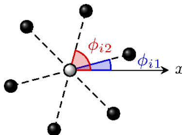
Figure 2.11.: Schematic view of the definition of the bond angles for a hexagonal lattice. Note that the crystal may be rotated with respect to the reference axis.
