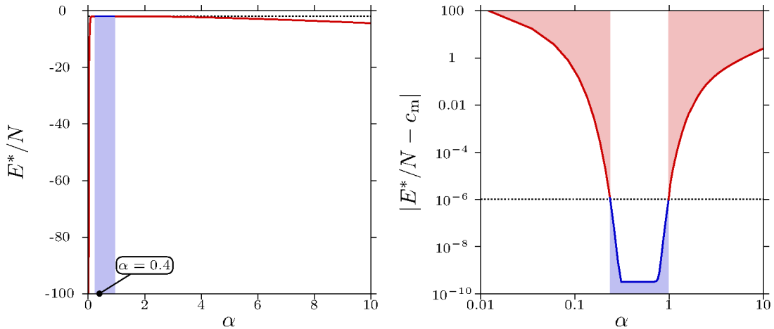
Figure 2.4.: \alpha -dependence of the Ewald summation for the hexagonal Wigner monolayer, i.e., a hexagonal (equilateral triangular) arrangement of point charges on a uniform neutralizing background (see text). The exact energy is known to be E_{\text{hex}}^*/N = c_{\text{m}} = -1.960515789 . Left panel: the energy calculation E^*/N diverges for small and large values of \alpha (indicated by red line color). If \alpha is chosen in a plateau region (shaded blue), E^*/N is constant for a certain interval. The correct energy c_{\text{m}} is indicated by a dotted line. The size of the interval increases with increasing cutoff distances R_{\text{cut}} and G_{\text{cut}} . Right panel: double-logarithmic plot of the error |E^*/N - c_{\text{m}}| giving an estimate of the attainable accuracy. The desired accuracy \delta \approx 10^{-6} is indicated by a dotted line.
