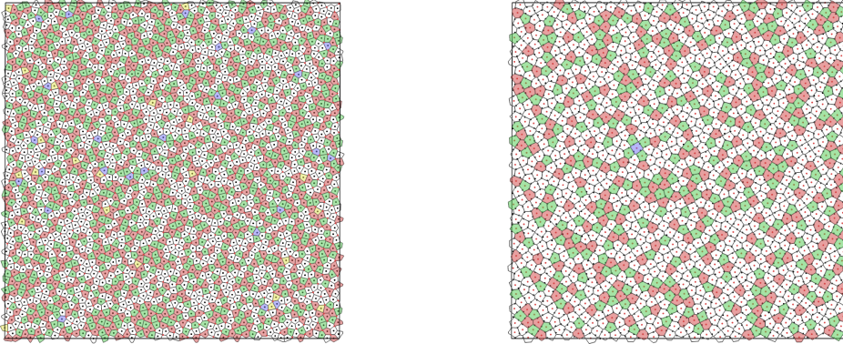
Figure 3.31.: Snapshots of MC simulations for \eta = 0.45 and A = 0.703 (where we predict structure S_2 ). Particles in layer 1 and 2 are colored black and red, respectively. Voronoi polygons are colored according to their number of sides: three sides (black), four (yellow), five (green), six (white), seven (red), eight (blue). Left panel: Voronoi construction for layer 1. Right panel: Voronoi construction for layer 2.
