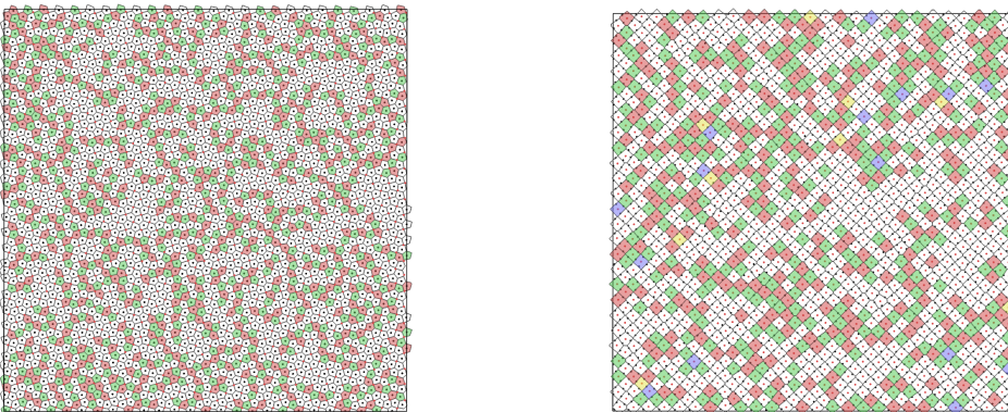
Figure 3.32.: Snapshots of MC simulations for \eta = 0.60 and A = 0.657 (where we predict structure S_1 ). Particles in layer 1 and 2 are colored black and red, respectively. Voronoi polygons are colored according to their number of sides: three sides (black), four (yellow), five (green), six (white), seven (red), eight (blue). Left panel: Voronoi construction for layer 1. Right panel: Voronoi construction for layer 2. Note the excellent square order.
