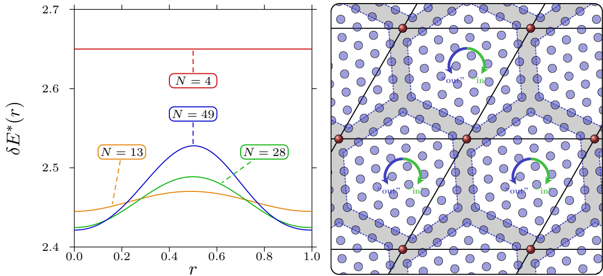
Figure 3.11.: Left panel: energy barriers calculated for the four considered system sizes N = 4, 13, 28, 49 . The reaction coordinate r describes the transition from start-configuration ("out"; r = 0 ) to end-configuration ("in"; r = 1 ). There is no barrier for N = 4 , since start- and end-configuration (after local relaxation) are identical in this case. For the other values of N , we observe an increase in barrier height as N increases. Right panel: snapshot of the saddle point configuration for N = 49 . Hexagonal crystallites are indicated by dashed blue lines; arrows indicate how the rotation of these crystallites leads towards "out"- and "in"-branch configurations, respectively. At the saddle point, lanes (shaded gray) connecting the periodic images of the tagged charge appear.
