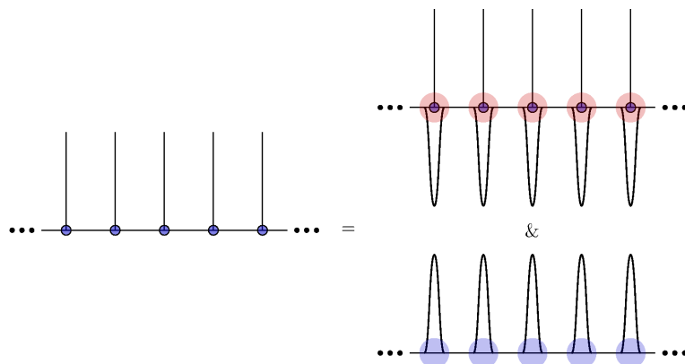
Figure 2.3.: Schematic view of the physical interpretation of Ewald summation used in some textbooks. Left panel: actual physical system, which consists of an infinite arrangement of point-like interaction sites, i.e., the distribution is delta-like. Right panel: introduction and consequent subtraction of a screening distribution, which makes the interaction manageable. The interactions in the top panel are calculated in real space while those in the bottom panel is treated in reciprocal space. This may be significantly easier to accomplish if the shape of the screening distribution is convenient, e.g., if its Fourier transform decays quickly with increasing k .
