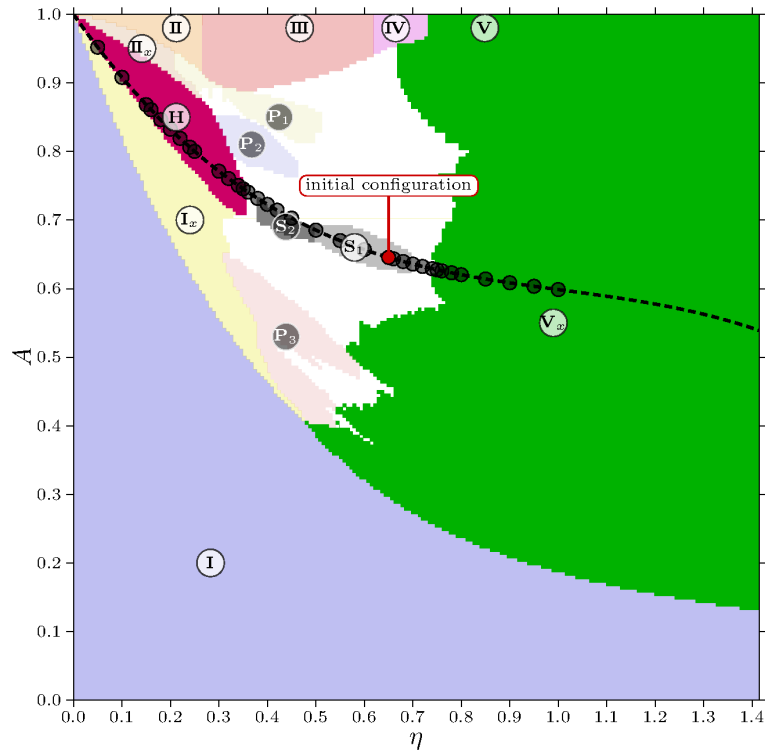
Figure 3.28.: State points investigated with MC simulations (indicated by black dots). We use a rough interpolation line [ A(\eta) = 1 - 1.00749\eta + 0.905807\eta^2 - 0.299731\eta^3 ] (dashed line), along which x \approx 1/3 . The red dot indicates the S_1 -configuration obtained with the EA used for initialization of the simulation. Note that along a small section of this line, the EA predicts x \neq 1/3 , a feature which is confirmed by the MC simulations.
