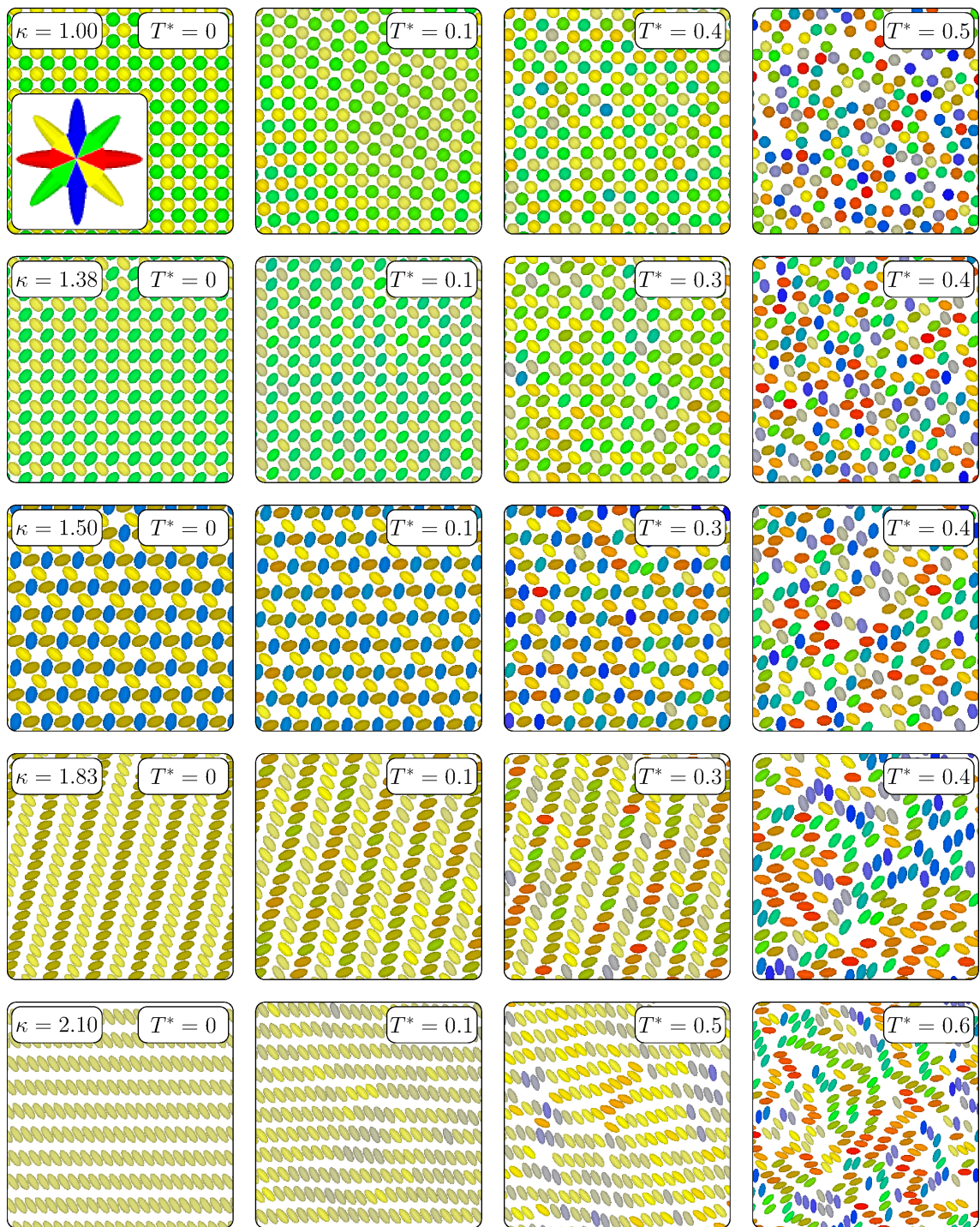
Figure 3.42.: Snapshots of MD simulations (courtesy of Thomas Heinemann [185]) for different values of \kappa = \sigma_{\parallel}/\sigma_{\perp} (as labeled) and T^* = k_{\text{B}}T/\epsilon_0 (as labeled). Different colors indicate different particle orientations (see inset in the top left panel). First row: \kappa = 1 ( T_{\text{sq}} -configuration). Second row: \kappa = 1.38 ( \text{HB}_{\text{dense}} -configuration). Third row: \kappa = 1.5 (TH-configuration). Fourth row: \kappa = 1.83 ( \text{HB}_{\text{loose}} -configuration). Fifth row: \kappa = 2.1 (PD-configuration).
