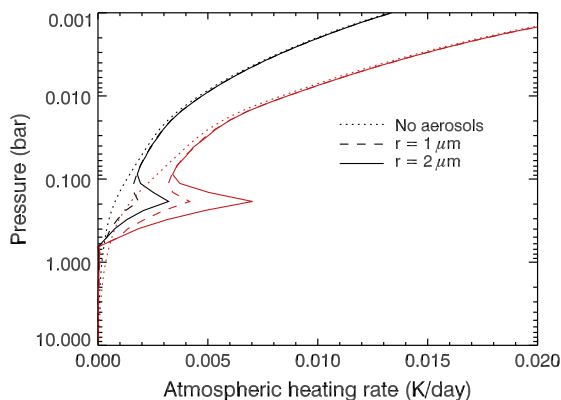
Fig. 9. Atmospheric heating rates profiles obtained with aerosols (solid and dashed lines) or for a clear atmosphere (dotted lines) at 20^{\circ}\text{S} for L_s = 120^{\circ} (winter, in black) and L_s = 300^{\circ} (summer, in red). Integrated aerosol opacity is set to 15, and two different particle sizes r are used. (For interpretation of the references to color in this figure legend, the reader is referred to the web version of this article.)
