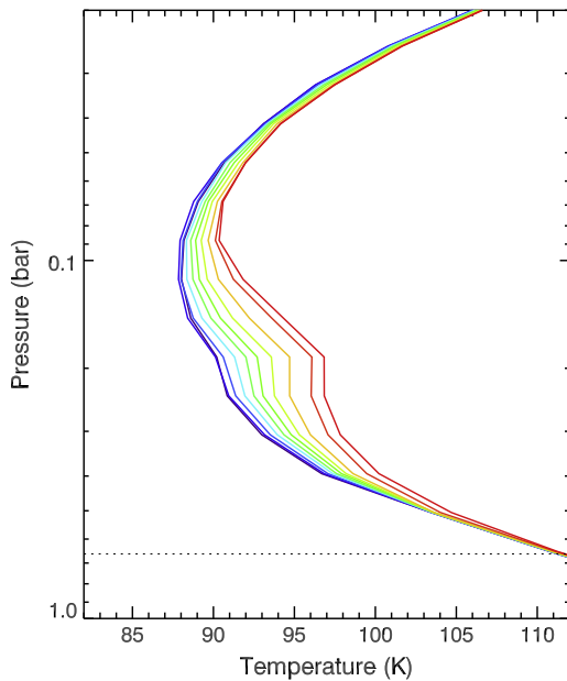
Fig. 8. Temperature profiles modeled at 20^{\circ}\text{S} , L_s = 300^{\circ} with \tau_{\text{tropo}} = 15 and various tropospheric particle sizes (0.2, 0.4, 0.6, 0.8, 1, 1.2, 1.5, 2, 3 and 4\ \mu\text{m} , from blue to red). (For interpretation of the references to color in this figure legend, the reader is referred to the web version of this article.)
