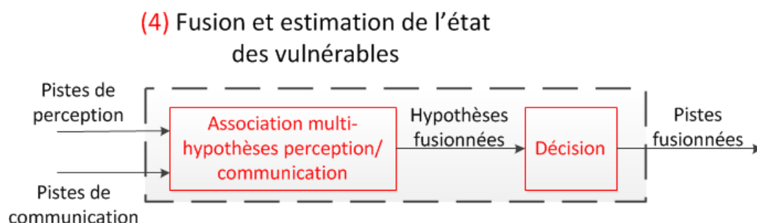
FIGURE 5.4: Architecture de la fusion d'information perception/communication
