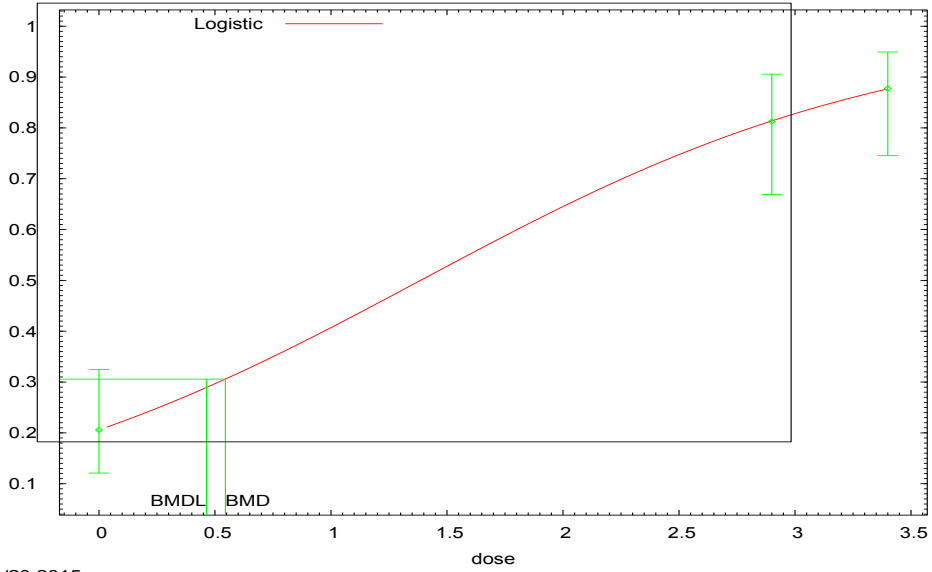
Logistic Model, with BMR of 10% Added Risk for the BMD and 0.95 Lower Confidence Limit for the BMDL
