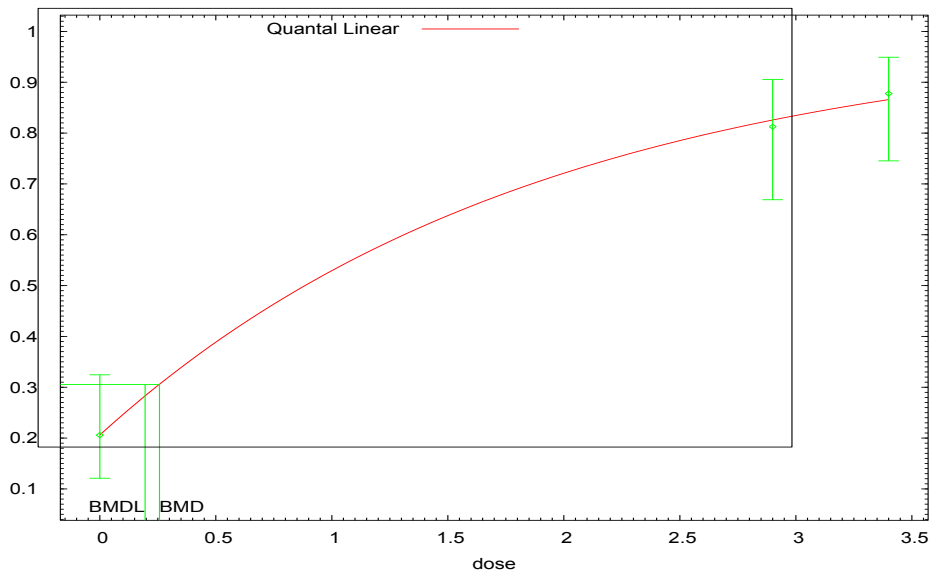
Quantal Linear Model, with BMR of 10% Added Risk for the BMD and 0.95 Lower Confidence Limit for the BMD
