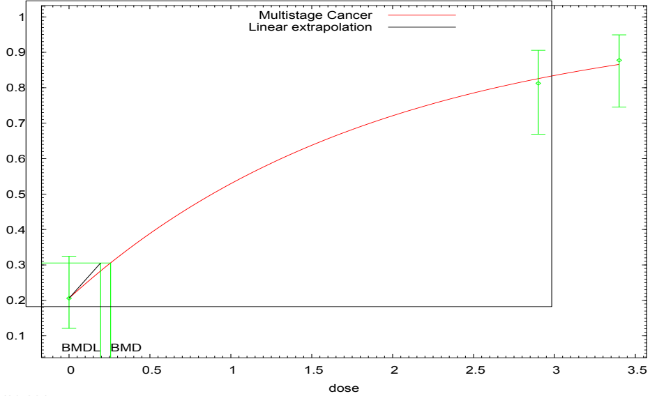
Multistage Cancer Model, with BMR of 10% Added Risk for the BMD and 0.95 Lower Confidence Limit for the BM
