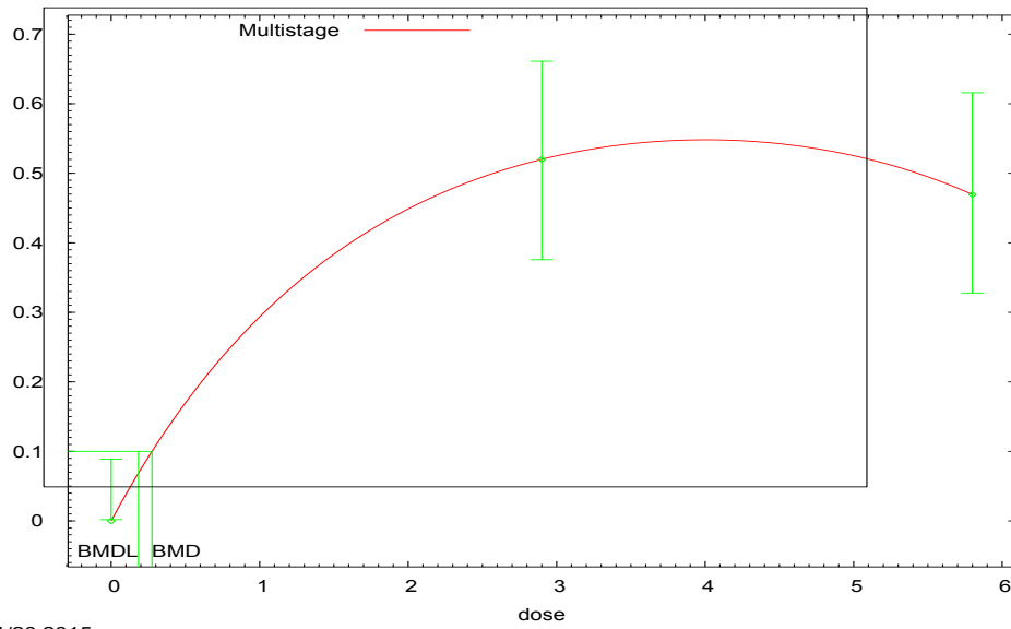
Multistage Model, with BMR of 10% Added Risk for the BMD and 0.95 Lower Confidence Limit for the BMDL
