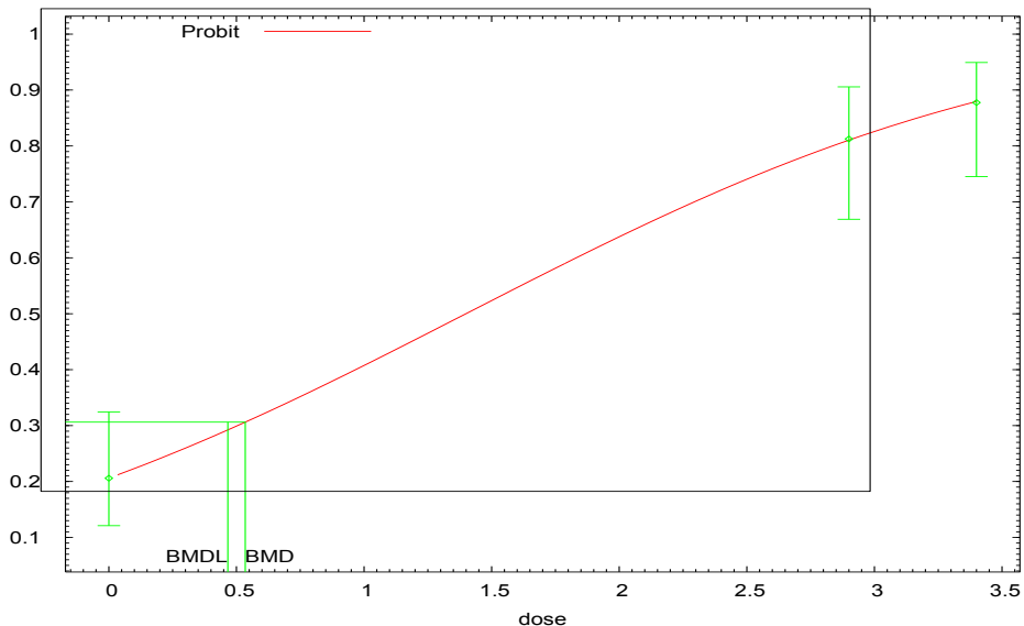
Probit Model, with BMR of 10% Added Risk for the BMD and 0.95 Lower Confidence Limit for the BMDL
