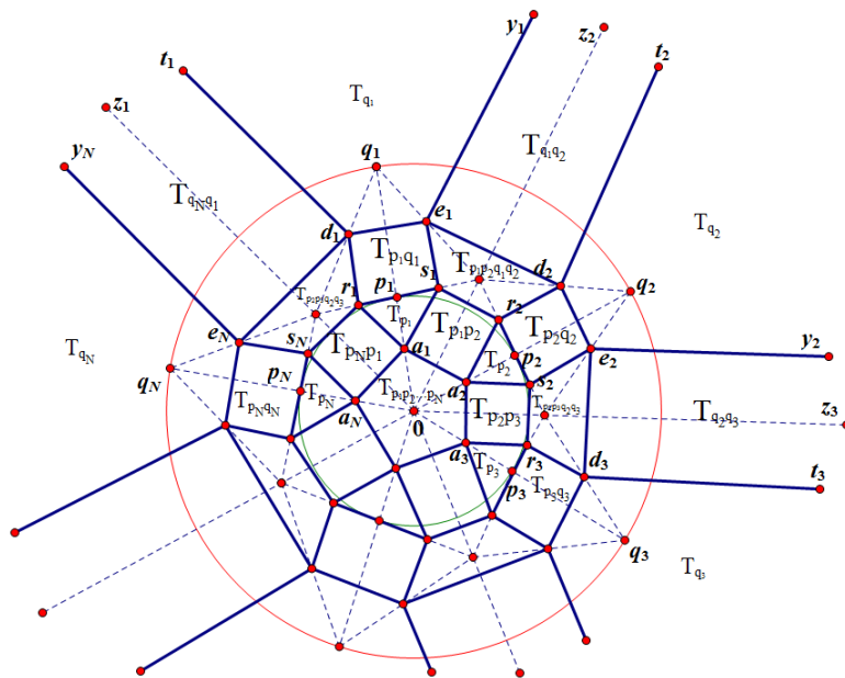
Figure 3.23: The function w^-
