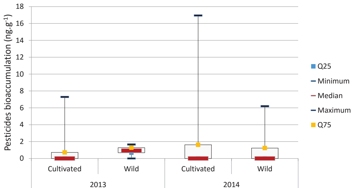
Figure 5: Metolachlor bioaccumulation ( \text{ng.g}^{-1} ) in summer 2013 and 2014 in adults oysters. Data represent the median, minimum and maximum concentrations in \text{ng.g}^{-1} dry weight \pm SD of the cultivated or wild oysters in summer 2013 and 2014. Each sample represent a pool of 30 oysters in 2013 or 50 oysters in 2014
