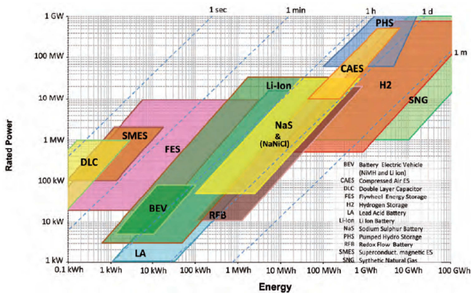
Figure 1.9 Comparison of rated power, energy content and discharge time of different energy storage technologies (Fraunhofer ISE) [40]
