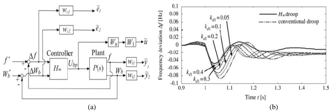
Figure 1.11 H infinity controller for energy storage
