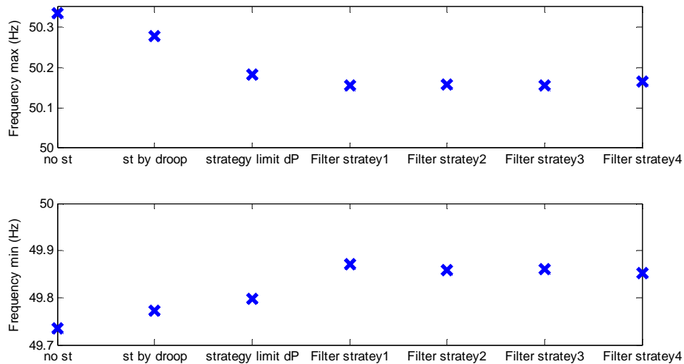
Figure 5.58 Frequency maximal and minimum of different strategies for energy storage with cut-off frequency 0.025Hz for filtering strategy #2 and #3 in 20/10/2011
