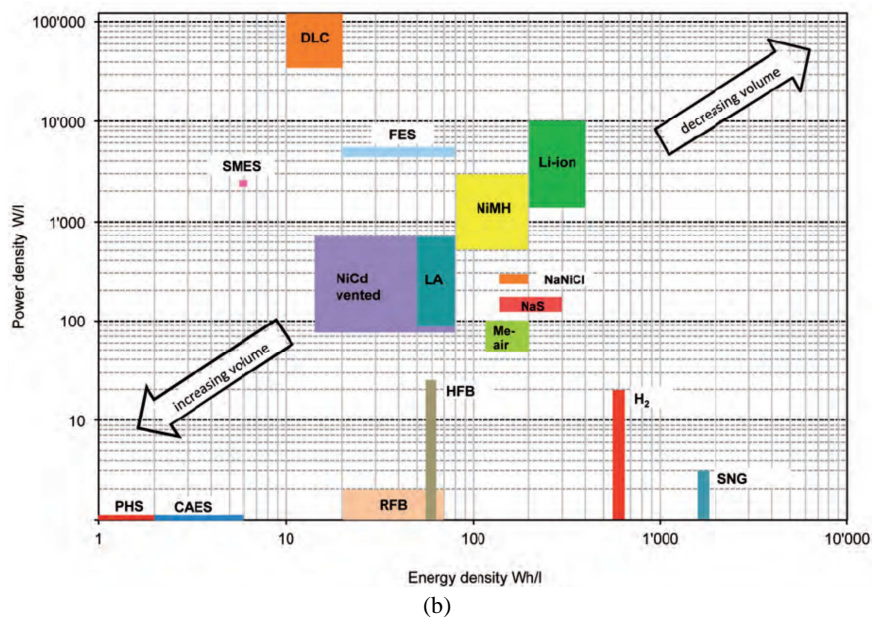
Figure 1.8 (a) Ragone chart of different energy storage technologies [48] (b) Chart of power density and energy density in ratio to volume for various energy storage technologies [40]
