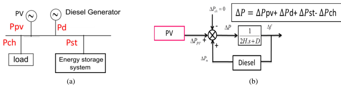
Figure 5.1 Simulated system
