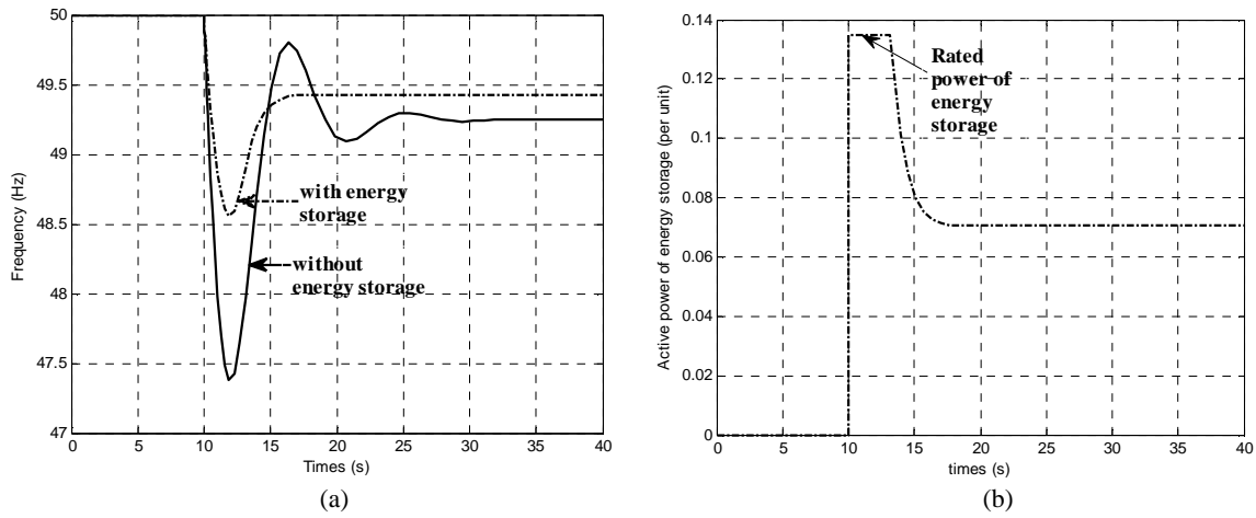
Figure 1.10 (a) Frequency response (b) Active power of energy storage for energy storage as impulse source in [13]
