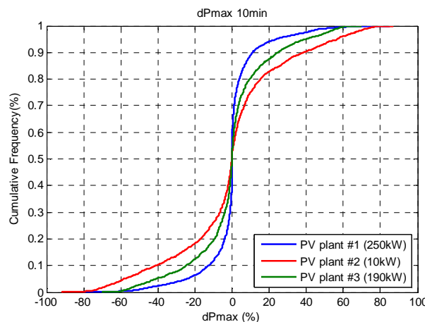
Figure 2.26 Cumulative distribution of PV plant #1, #2, and #3 for time duration 10 minutes
