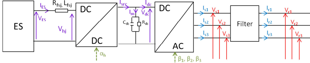
Figure 4.2 Energy storage device connected to system via DC/DC converter, inverter, and AC filter
