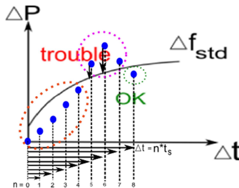
Figure 5.6 Control strategy
