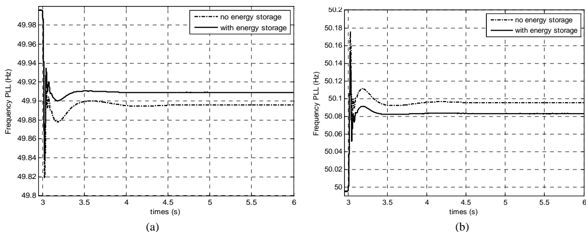
Figure 4.38 Frequency response of system without and with ESS (a) increasing of load power (b) decreasing of load power 100kW
