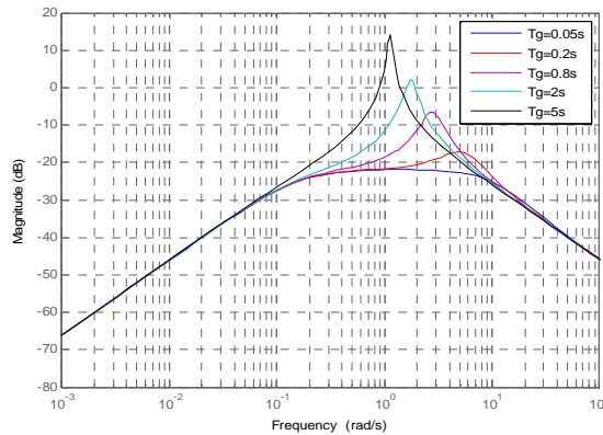
Figure 3.10 Bode diagram of system (with primary and secondary control of diesel generator) with different time response of diesel generator
