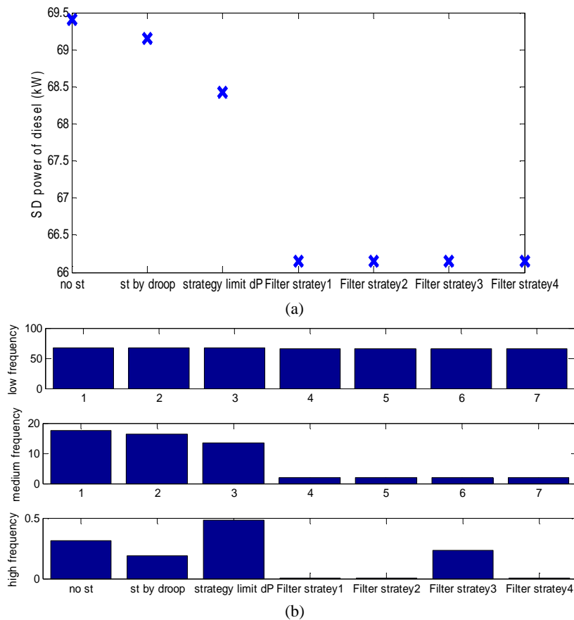
Figure 5.63 (a) Spectral (b) FHC in each frequency range of power total of diesel generator
