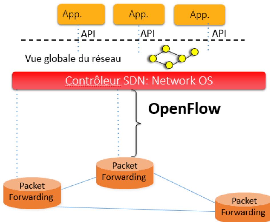
Figure 25 : Architecture SDN
