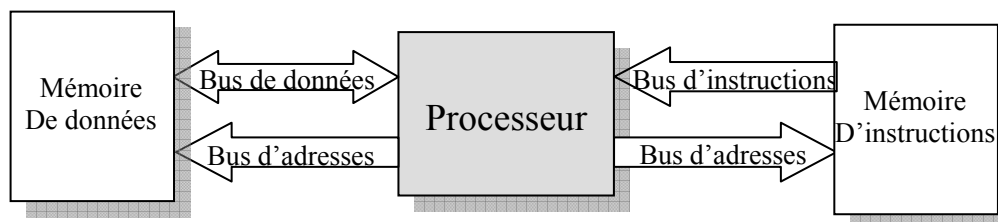
Figure 31. Architecture Harvard
