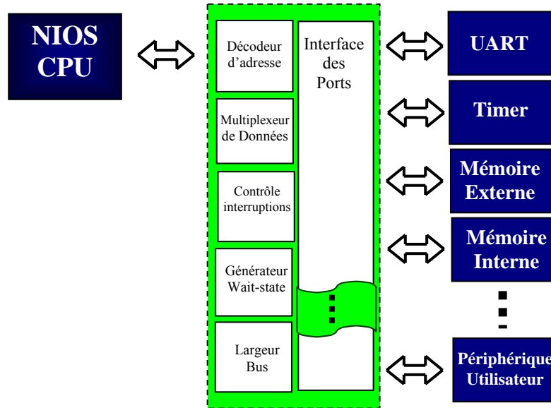
Figure 36. Bus Avalon
