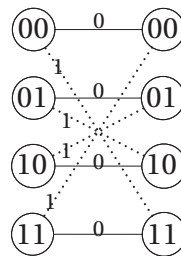
Figure 3.8. Section-product cell1 \otimes cell1 .
