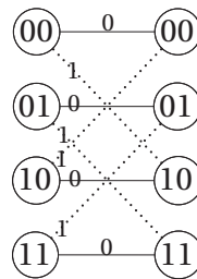
Figure 3.7. Section-product cell1 \otimes cell0 .
