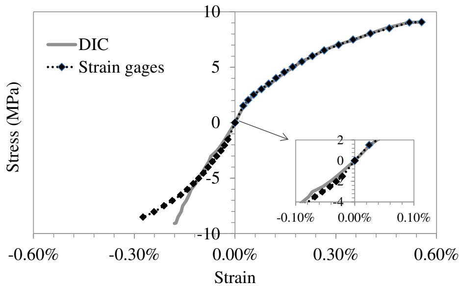
Figure III-14: Comparison between experimental results of AT VF obtained using DIC and conventional gages
