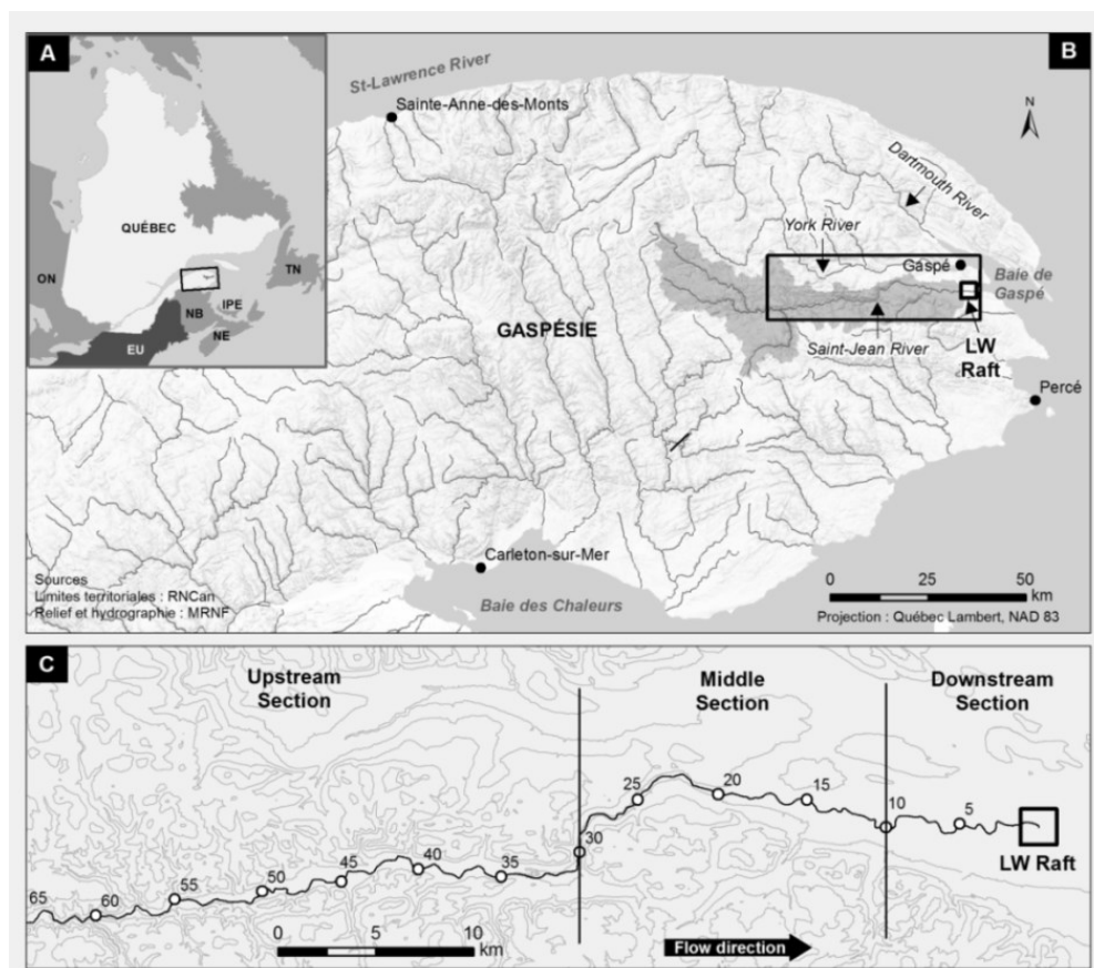
Figure 39. (A) Large-scale map showing the location of the Saint-Jean River in Québec, Canada. (B) Location of the Saint-Jean River on the Gaspé Peninsula. (C) Detailed map showing the studied river corridor with distance from the river mouth in kilometres (kilometric point: PK)
