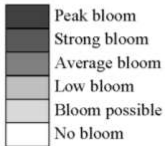
Figure III-3. Blooming calendar of host plant of Orthops palus in Reunion Island
