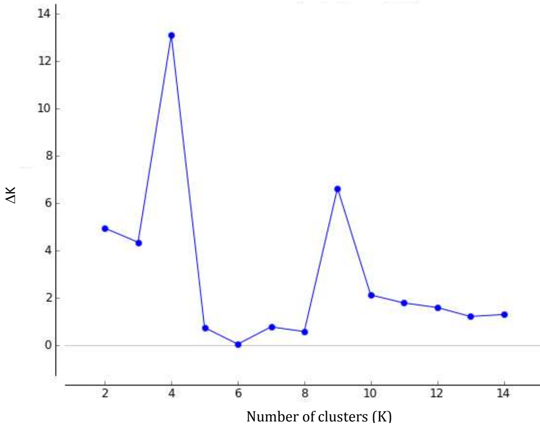
Figure IV-S5. Average likelihood of runs in structure and optimal number of clusters ( K ) of Orthops palus populations of Mauritius according to Evanno et al. (2005)
