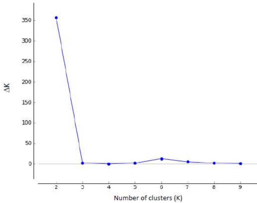
Figure IV-S2. Average likelihood of runs in structure and optimum number of clusters (delta K ) according to Evanno et al. (2005)
