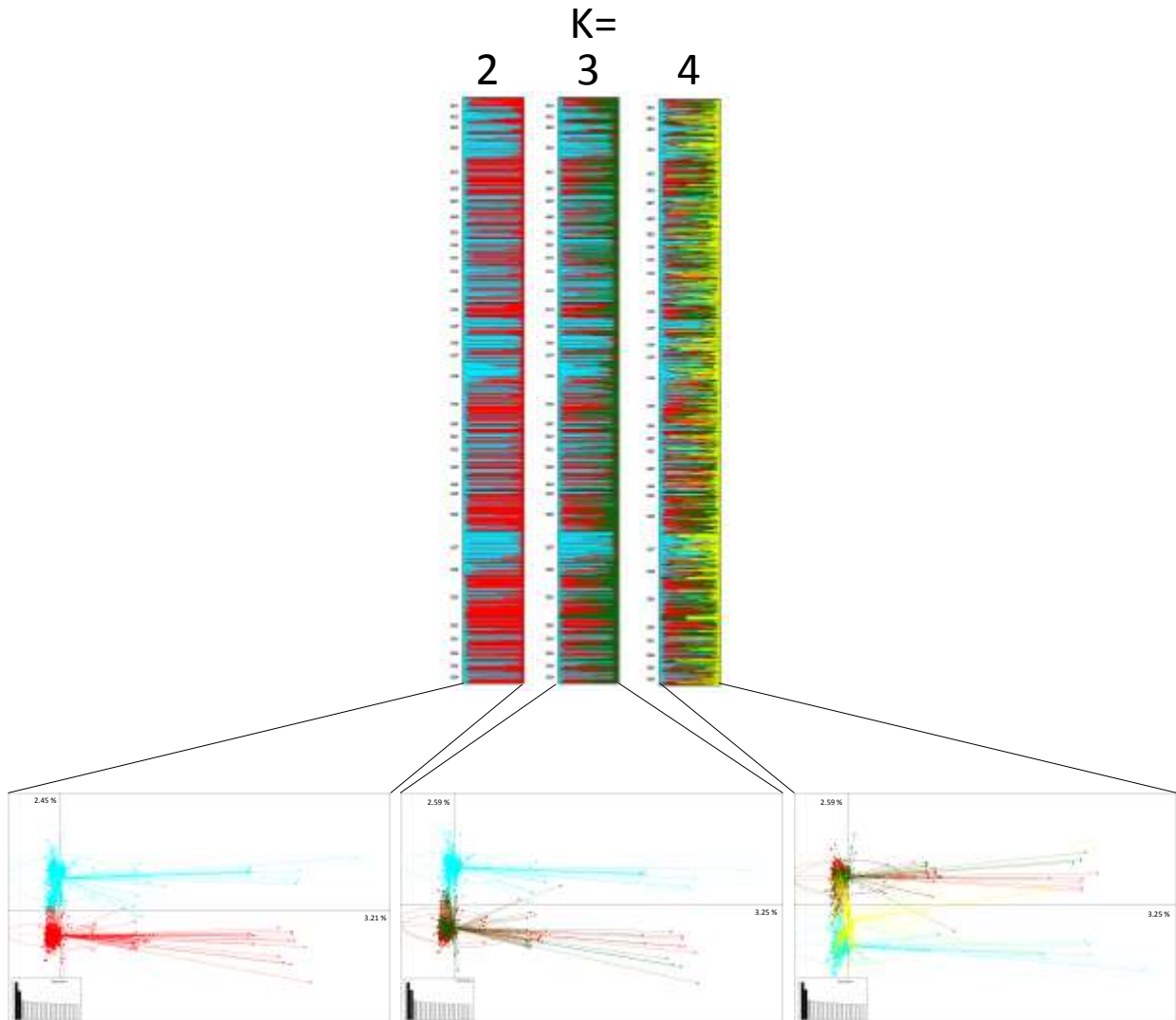
Figure IV-S4. Admixture proportions and Principal Component Analysis among genotypic clusters
