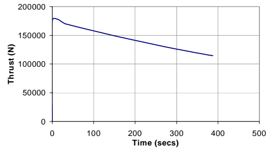
Figure 12. Ascent Engine Thrust.
