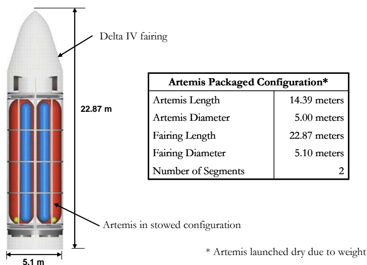
Figure 6. Artemis in Stowed Configuration.
