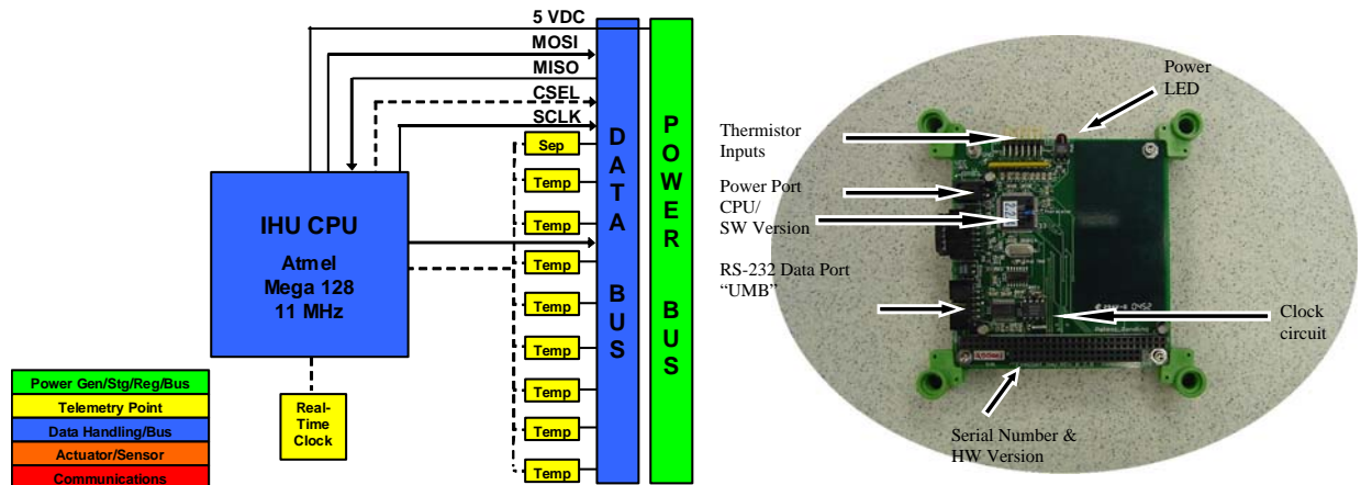
Figure 5. Data Handling Block Diagram and Module
