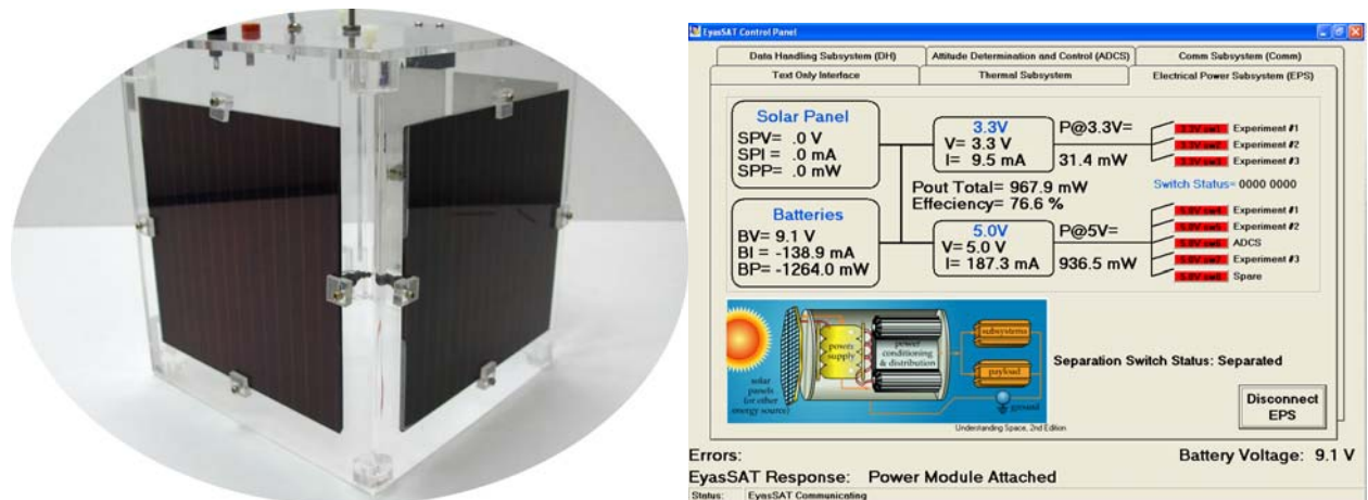
Figure 4. Electrical Power Subsystem Solar panels and GUI Screen. Embedded subsystem diagrams on the GUI screens used throughout this paper are from Understanding Space 19 and can be used as a classroom demonstration and teaching aide
