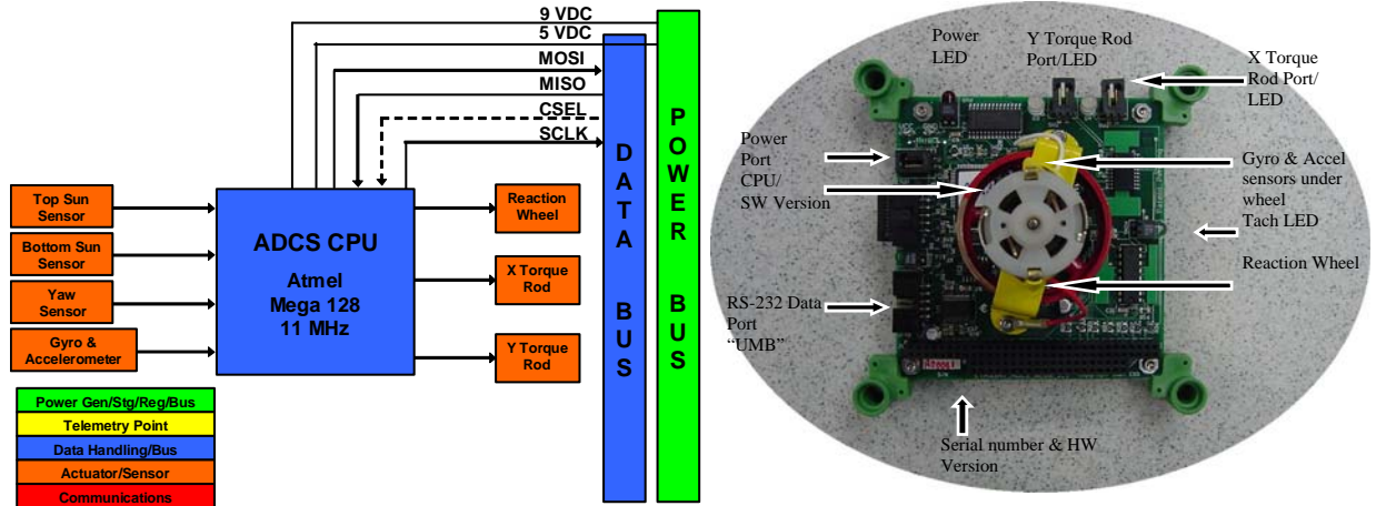
Figure 9. ADCS Module Features Integrated Reaction Wheel, Accelerometers, and Gyroscope
