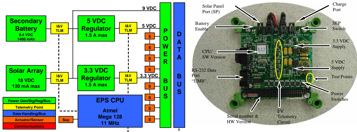
Figure 3. Electrical Power Subsystem Block Diagram and Module
