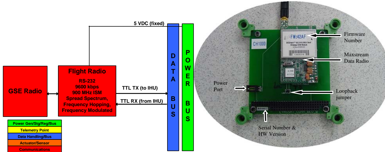
Figure 7. Communication Block Diagram and Module
