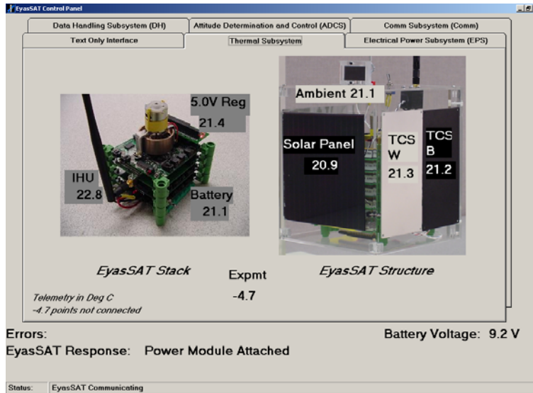
Figure 12. Thermal Control Subsystem GUI Screen
