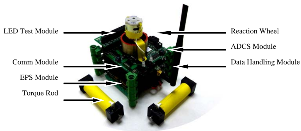
Figure 1. EyasSAT Subsystems
