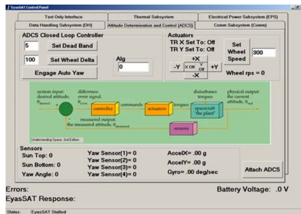
Figure 11. Attitude Determination and Control GUI Screen
