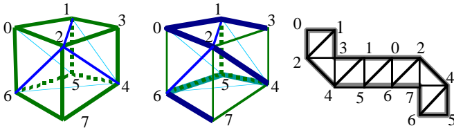
Figure 1: The triangulation of a polyhedron (left) may be cut (thick blue edges) into a flat triangulated polygon without interior vertices (right). When this polygon has no bifurcation, it may be represented by a single triangle strip where triangles are attached to free edges of the previous triangle. OpenGL requires to alternate between the left and the right free edge. Except for the first and last ones, each vertex has 3 incident edges (right). Note that each vertex, except for 3 and 7, which are the end-vertices of the strip, is encoded twice. Indeed, general vertices appear either in the boundary of a strip or are separated by non-consecutive triangles within the same strip.
