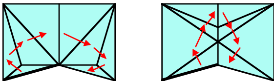
Figure 2: The two meshes have the same boundaries and triangle-spanning trees, as shown by red arrows and described by the sequence of moves left, right, right, right, left, right.
