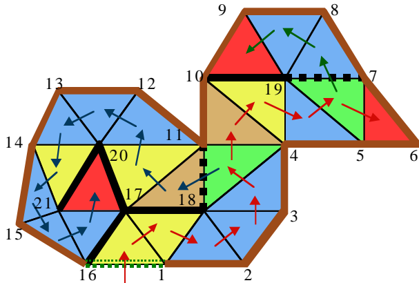
Figure 4: The triangle X , identified because it is the triangle in the remaining portion of the mesh that is incident upon the gate g , will be removed. The operation is of type C if the third vertex v of X that is bounding g has not yet been visited. If it has, then it is included in B . If it both immediately precedes g and immediately precedes the start of g along B , then X is the last triangle of R_0 and we record an E operation immediately follows, but does not precede it. If v does not immediately follow but precedes g , we record an L operation. Finally, if v lies between g and g but is not immediately precedes or follows the vertices of g , we record an S operation.
