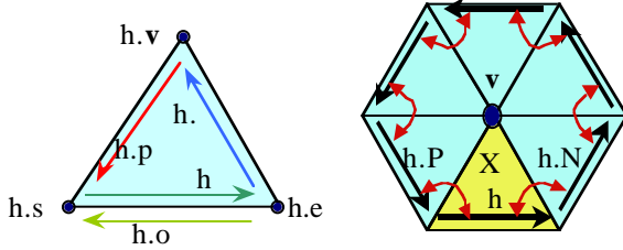
Figure 6: A half-edge, h , green arrow (left), starting and ending vertices, s and h.e and to the opposite vertex, v . The other two edges of the triangle associated with h are denoted (red and blue arrows). The opposite half-edge, h.o (lime arrow) provides access to the adjacent triangle when it exists. Curved red bi-directional arrows (right) present links h.P and h.N that organize the half-edges of B into a doubly-linked cyclic list.
