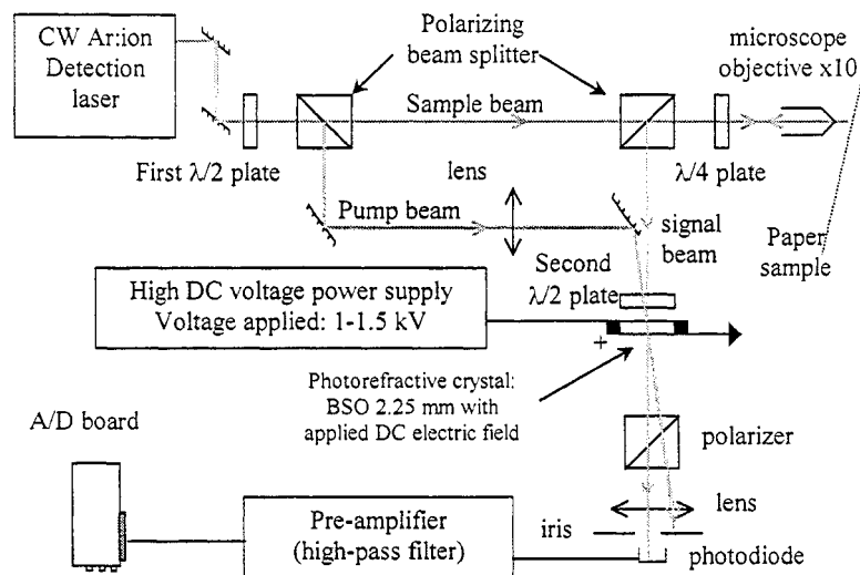
Fig. 3. Schematic diagram of the photorefractive interferometer setup [30].
