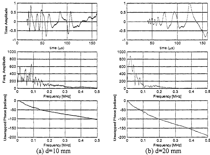
Fig. 8. A_0 mode analysis of signals on static copy paper in CD; top: zero-padded A_0 signal in time domain, middle: amplitude spectrum, bottom: unwrapped phase angle spectrum.
