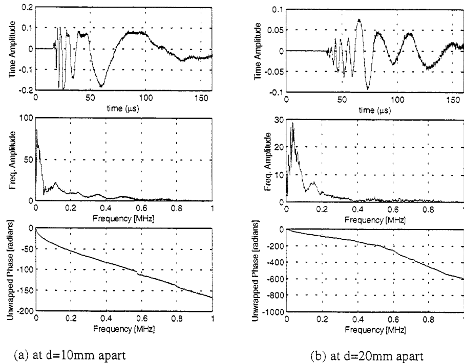
Fig. 13. A_0 mode analysis at 10- and 20-mm distances between generation and detection in copy paper in CD at 2 m/s.
