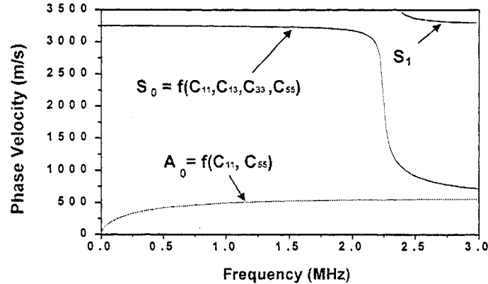
Fig. 5. Typical calculated dispersion curves in MD for copy paper.
