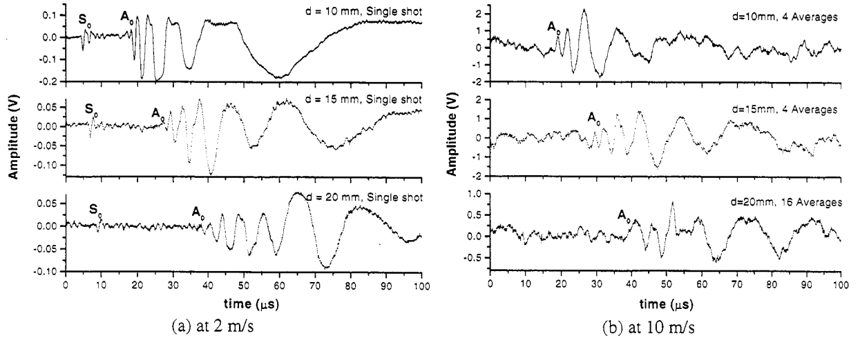
Fig. 12. Comparison of Lamb waves for different generation-detection separation distances in copy paper in CD at 2 m/s and 10 m/s.
