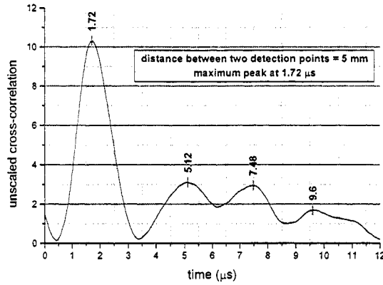
Fig. 7. Cross-correlation of two S_0 signals in Fig. 6 (a).
