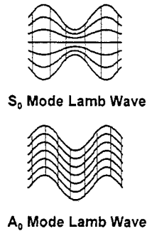
Fig. 2. Cross-sectional view of paper exhibiting the fundamental S_0 and A_0 modes for Lamb waves.
