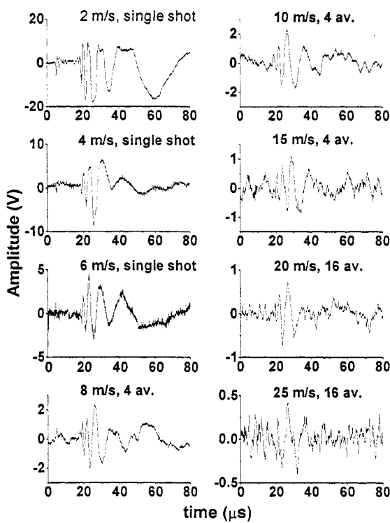
Fig. 10. Signals on moving copy paper in CD
