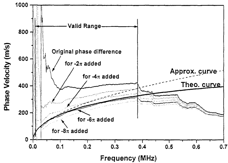
(a) A_0 Phase velocity vs. Frequency
