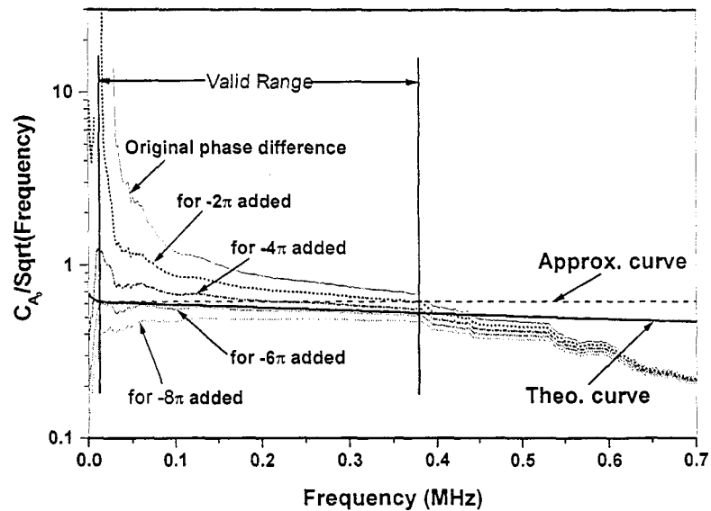
(b) C_{A_0} / \sqrt{\text{Freq}} vs. Frequency
