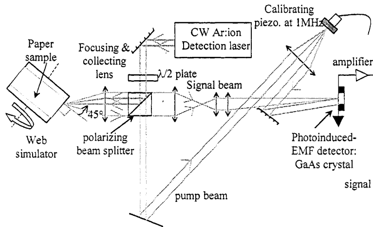
Fig. 4. Schematic diagram of the Photo-EMF interferometer [31]. The variable speed moving web simulator is shown on left side.
