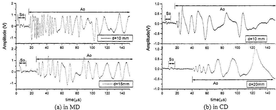
Fig. 6. Single shot signals collected with the TWM setup for non-moving copy paper in MD and CD.
