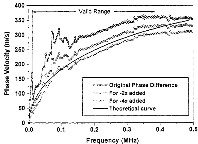
Fig. 9. A_0 mode phase velocities computed using Eq. 1 for different values of m (0,-1,-2) for phase correction.
