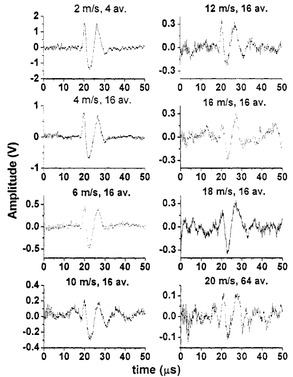
Fig. 11. Signals on moving 42-lb linerboard in MD
